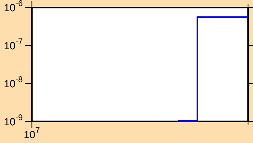
\sigma vs. E for ^{205}\text{Hg}(n,2n\alpha)
