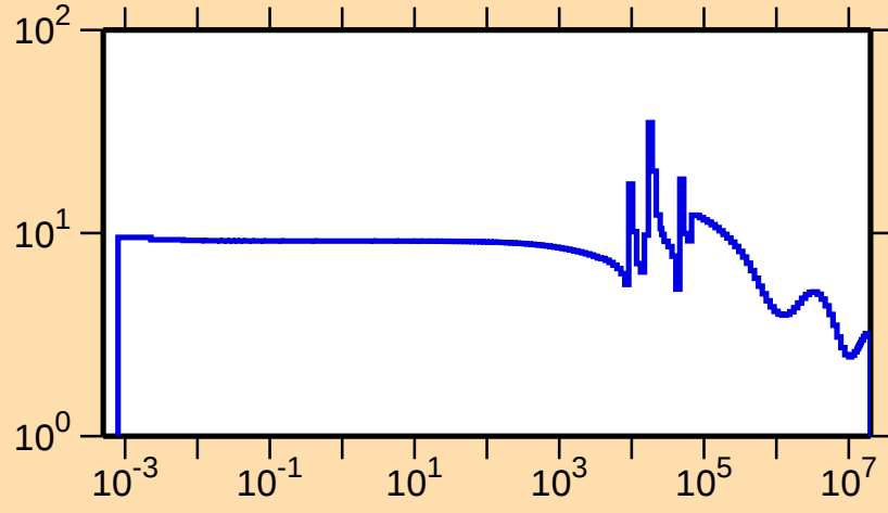
\sigma vs. E for ^{205}\text{Hg}(n,\text{el.})
