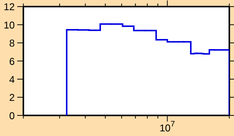
\Delta\sigma/\sigma vs. E for ^{205}\text{Hg}(n,n\text{onel.})
