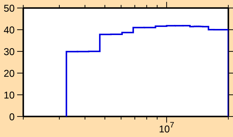
\Delta\sigma/\sigma vs. E for ^{205}\text{Hg}(n,n_1)
