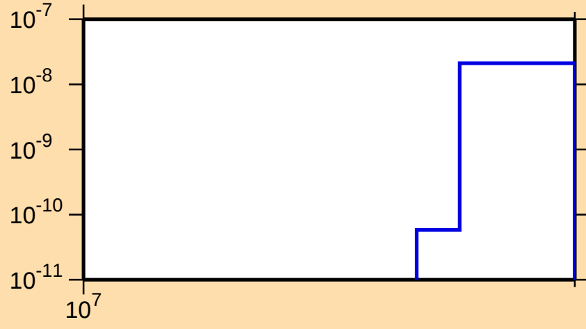
\sigma vs. E for ^{205}\text{Hg}(n,\text{nd})
