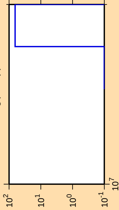
\Delta\sigma/\sigma vs. E for ^{205}\text{Hg}(n,2np)
