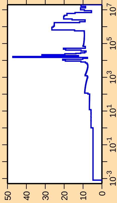
\Delta\sigma/\sigma vs. E for ^{205}\text{Hg}(n,\text{el.})
