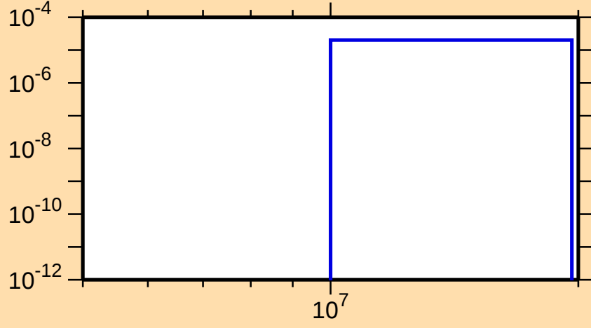
\sigma vs. E for ^{205}\text{Hg}(n,d)
