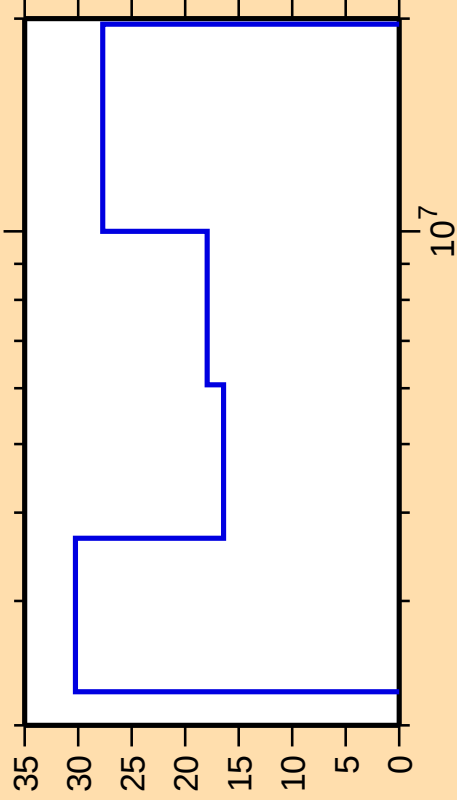
\Delta\sigma/\sigma vs. E for ^{205}\text{Hg}(\text{n},\text{ncont.})
