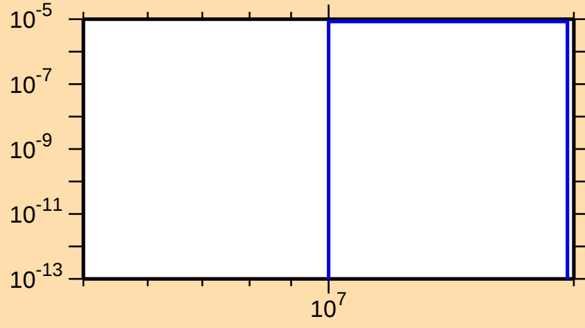
\sigma vs. E for ^{205}\text{Hg}(n,np)
