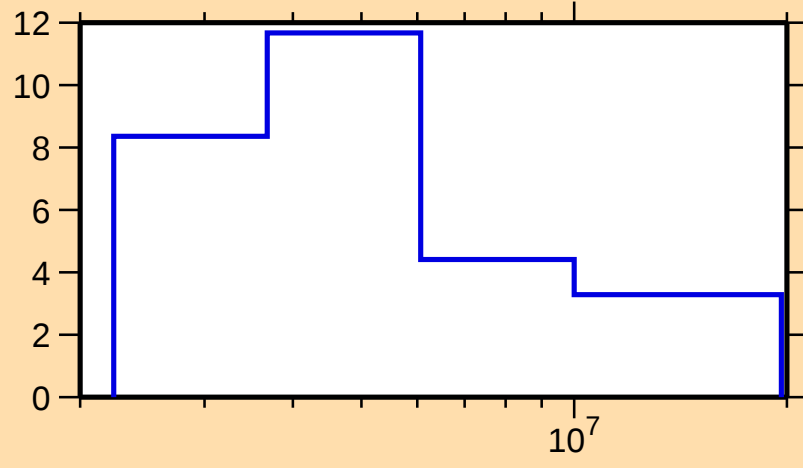
\Delta\sigma/\sigma vs. E for ^{205}\text{Hg}(\text{n},\text{tot.})
