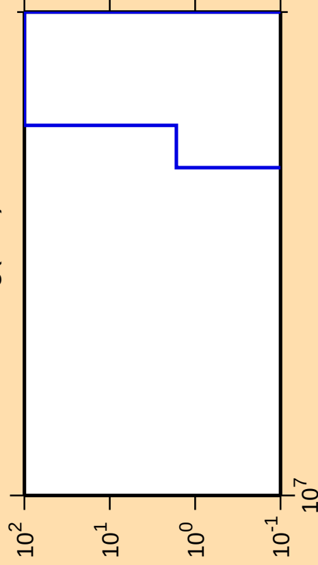
\Delta\sigma/\sigma vs. E for ^{206}\text{Hg}(n,\text{nt})
