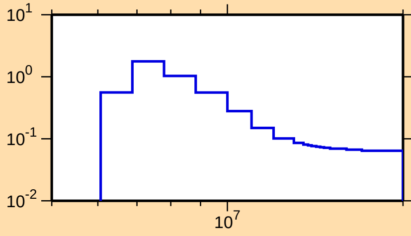
\sigma vs. E for ^{206}\text{Hg}(n,n\text{cont.})
