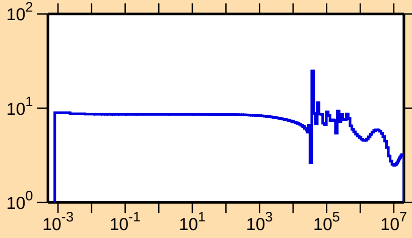
\sigma vs. E for ^{206}\text{Hg}(n,\text{el.})
