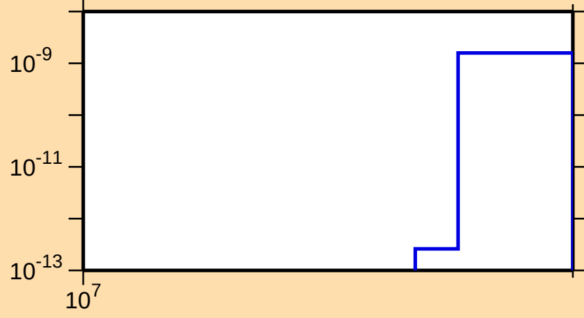
\sigma vs. E for ^{206}\text{Hg}(n,\text{nt})
