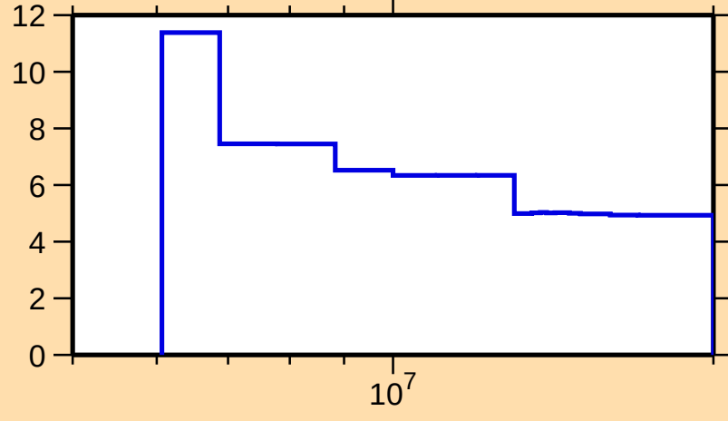
\Delta\sigma/\sigma vs. E for ^{206}\text{Hg}(n,n\text{oncl.})
