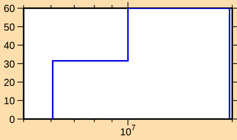
\Delta\sigma/\sigma vs. E for ^{206}\text{Hg}(n,p)
