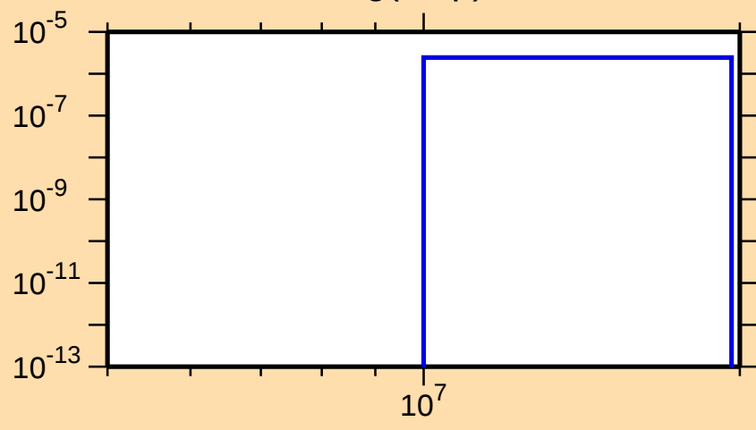
\sigma vs. E for ^{206}\text{Hg}(n,np)
