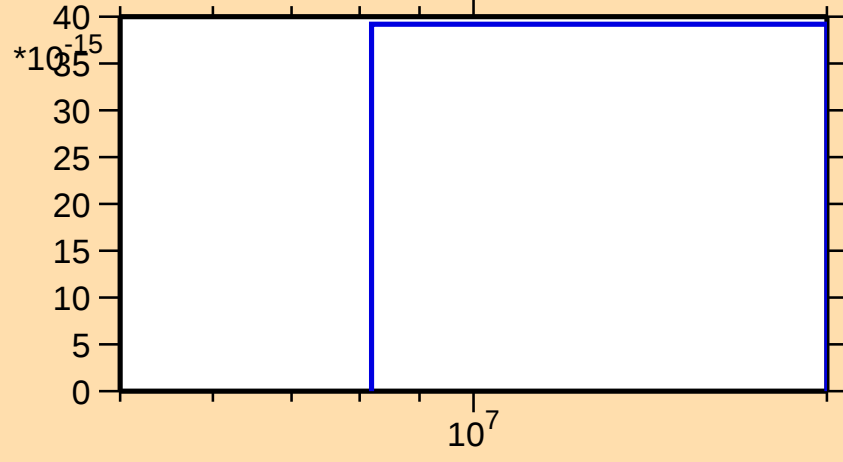
\sigma vs. E for ^{206}\text{Hg}(n,2n\alpha)
