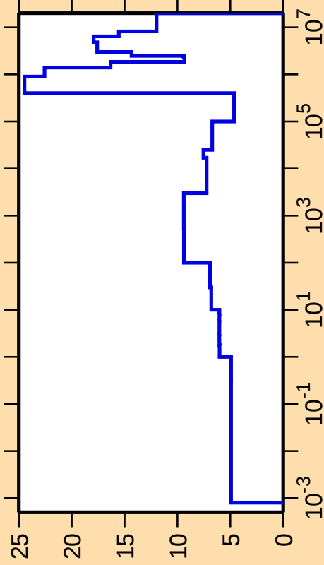
\Delta\sigma/\sigma vs. E for ^{206}\text{Hg}(n,\text{el.})
