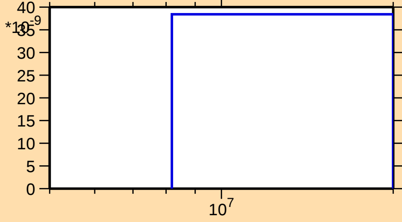
\sigma vs. E for ^{206}\text{Hg}(n,n\alpha)
