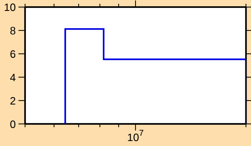
\Delta\sigma/\sigma vs. E for ^{206}\text{Hg}(n,\text{nonel.})
