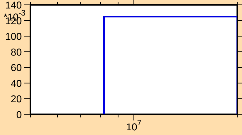
\sigma vs. E for ^{206}\text{Hg}(n,3n)
