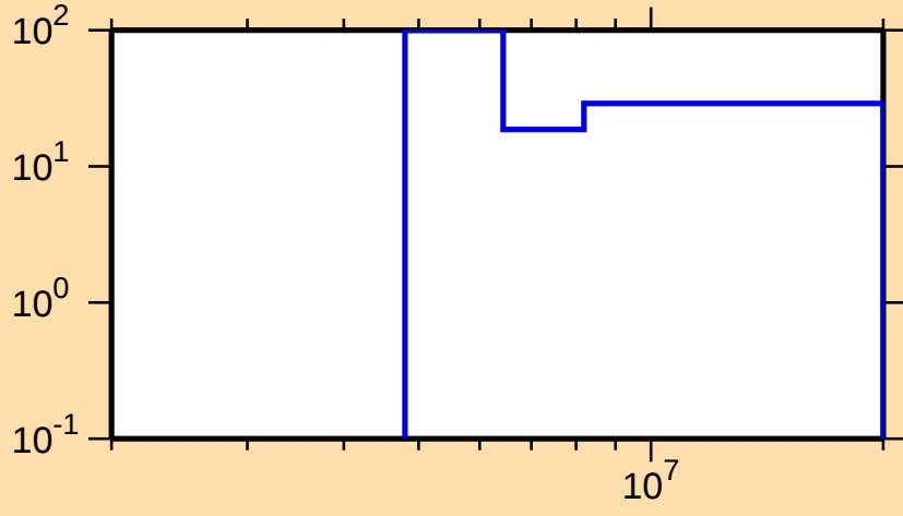
\Delta\sigma/\sigma vs. E for ^{206}\text{Hg}(n,n\text{cont.})
