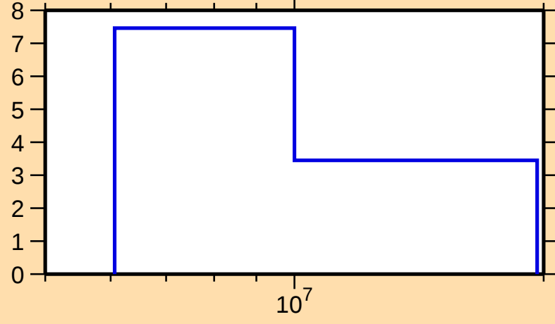
\Delta\sigma/\sigma vs. E for ^{207}\text{Hg}(n,\text{el.})
