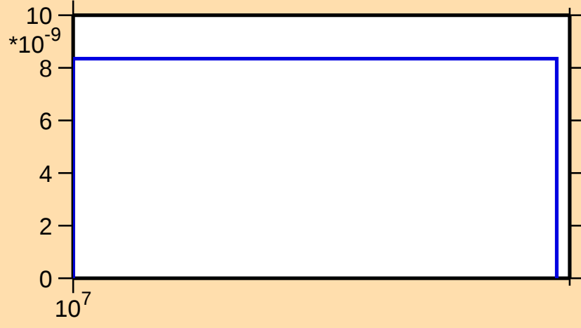
\sigma vs. E for ^{207}\text{Hg}(n,\text{nt})
