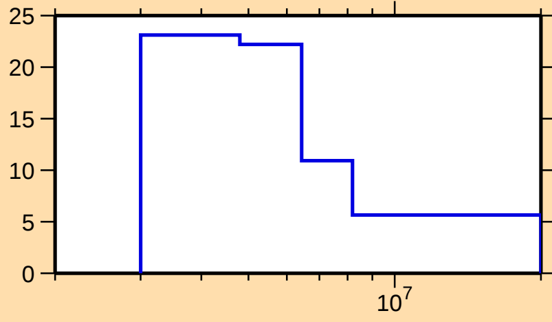
\Delta\sigma/\sigma vs. E for ^{207}\text{Hg}(n,2n)
