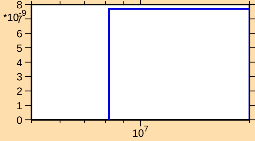
\sigma vs. E for ^{207}\text{Hg}(n,nt)
