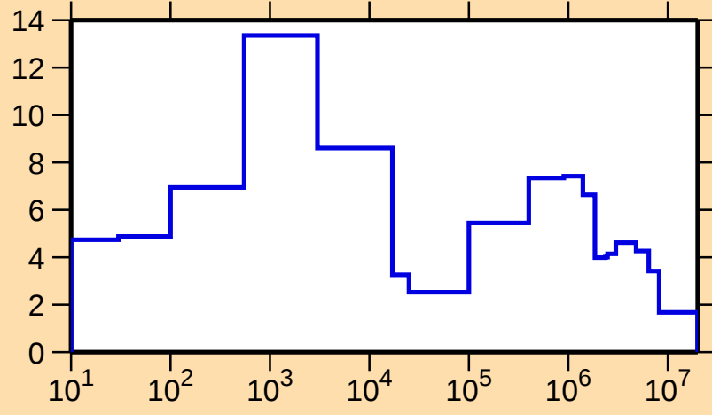
\Delta\sigma/\sigma vs. E for ^{207}\text{Hg}(n,\text{tot.})
