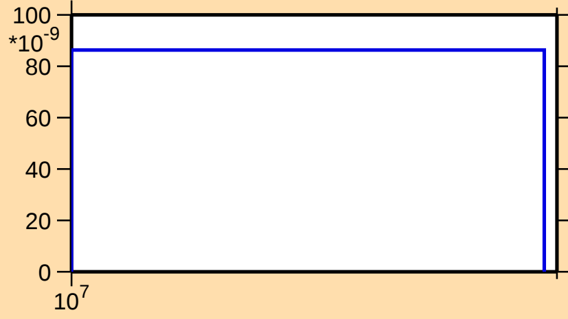
\sigma vs. E for ^{210}\text{Hg}(n,\text{nt})
