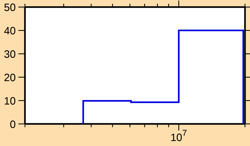
\Delta\sigma/\sigma vs. E for ^{210}\text{Hg}(n,2n)
