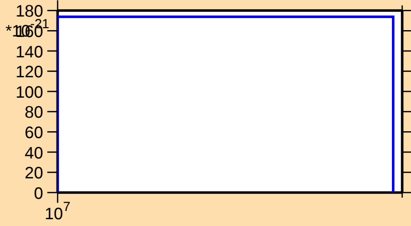
\sigma vs. E for ^{210}\text{Hg} (mt 42)
