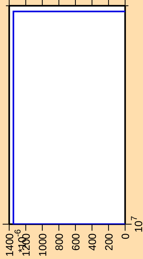
\Delta\sigma/\sigma vs. E for ^{210}\text{Hg} (mt 11)
