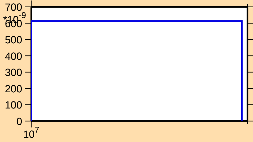
\sigma vs. E for ^{210}\text{Hg}(n,np)
