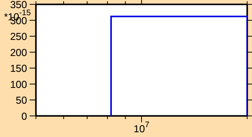
\sigma vs. E for ^{210}\text{Hg}(n,3n\alpha)
