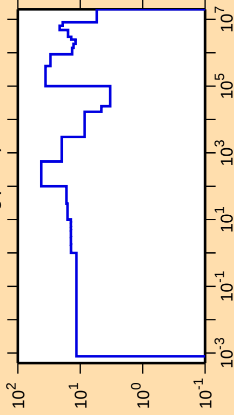
\Delta\sigma/\sigma vs. E for ^{210}\text{Hg}(n,\text{el.})
