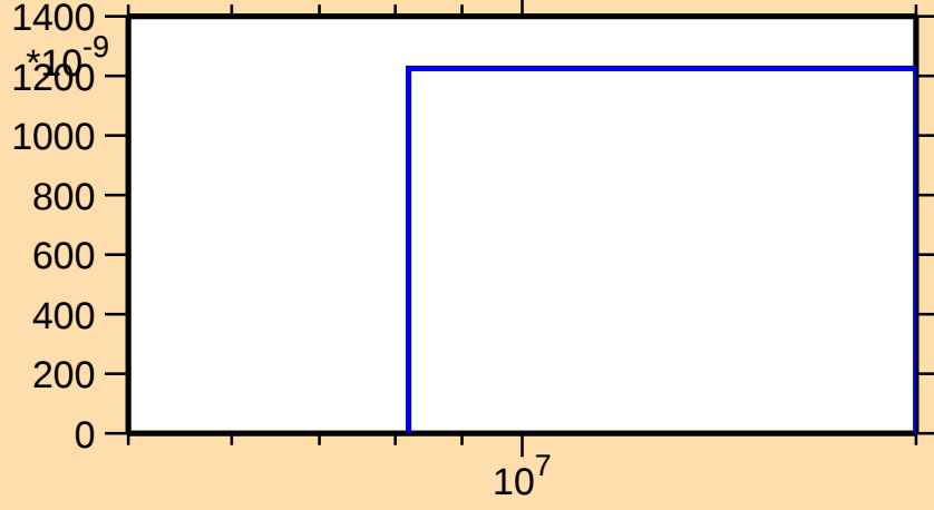
\sigma vs. E for ^{210}\text{Hg}(n,d)
