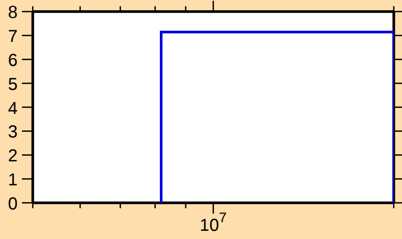
\Delta\sigma/\sigma vs. E for ^{210}\text{Hg}(n,\text{nonel.})
