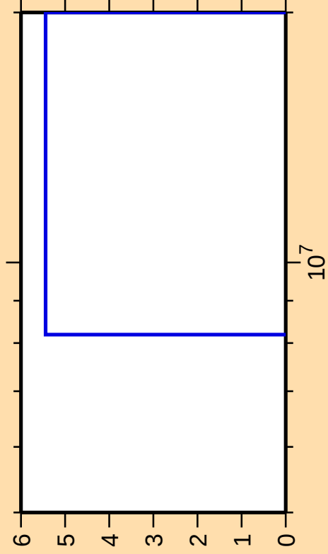
\Delta\sigma/\sigma vs. E for ^{210}\text{Hg}(n,2np)
