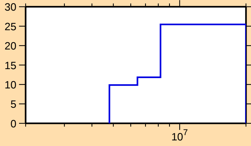
\Delta\sigma/\sigma vs. E for ^{210}\text{Hg}(n,2n)
