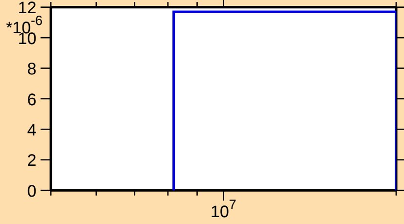
\sigma vs. E for ^{210}\text{Hg}(n,p)
