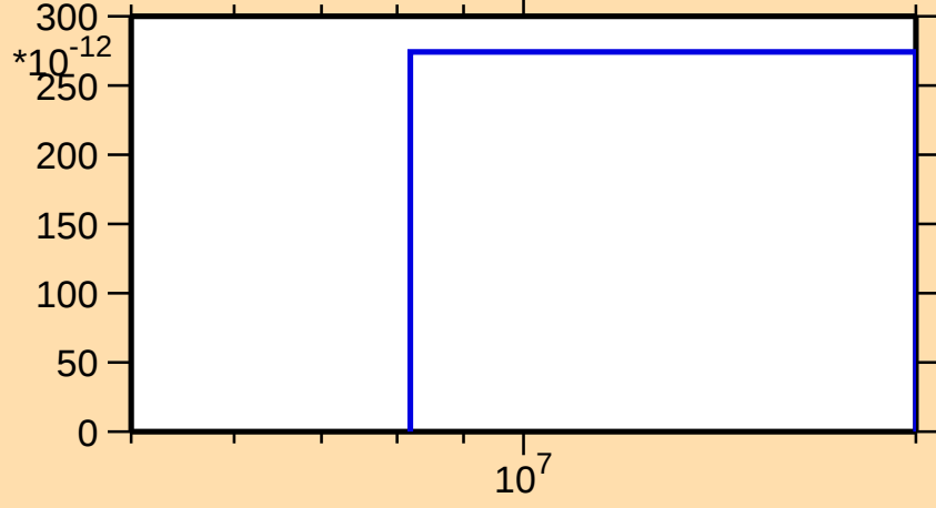
\sigma vs. E for ^{210}\text{Hg}(n,\text{nd})
