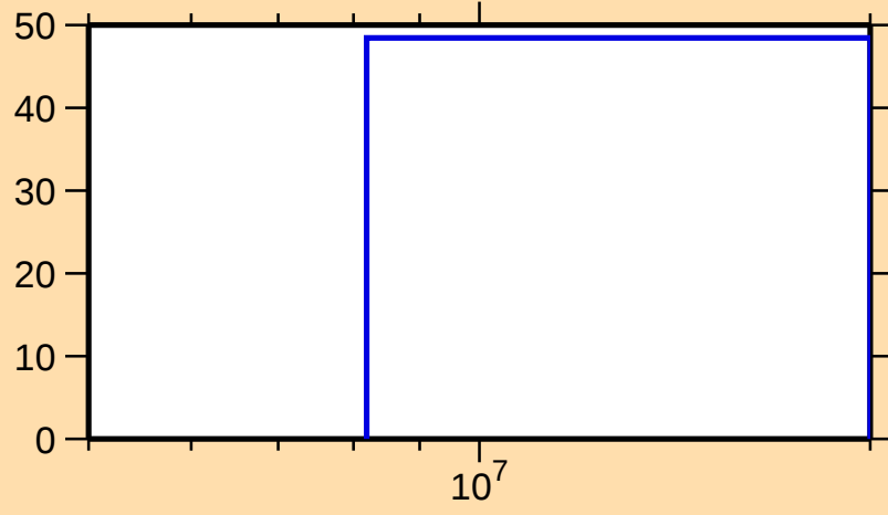
\Delta\sigma/\sigma vs. E for ^{210}\text{Hg}(n,n_1)
