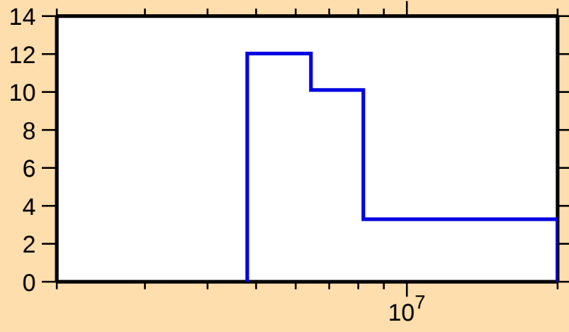
\Delta\sigma/\sigma vs. E for ^{210}\text{Hg}(n,\text{tot.})
