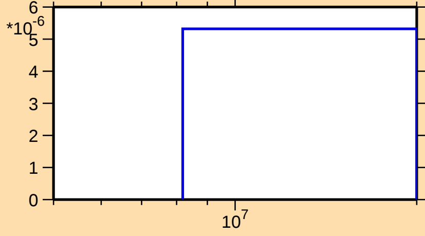
\sigma vs. E for ^{210}\text{Hg}(n,t)
