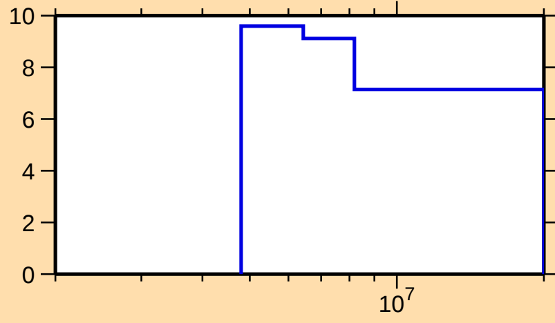
\Delta\sigma/\sigma vs. E for ^{210}\text{Hg}(n,\text{nonel.})
