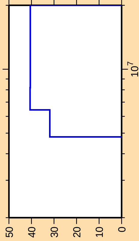
\Delta\sigma/\sigma vs. E for ^{210}\text{Hg}(n,n\text{cont.})
