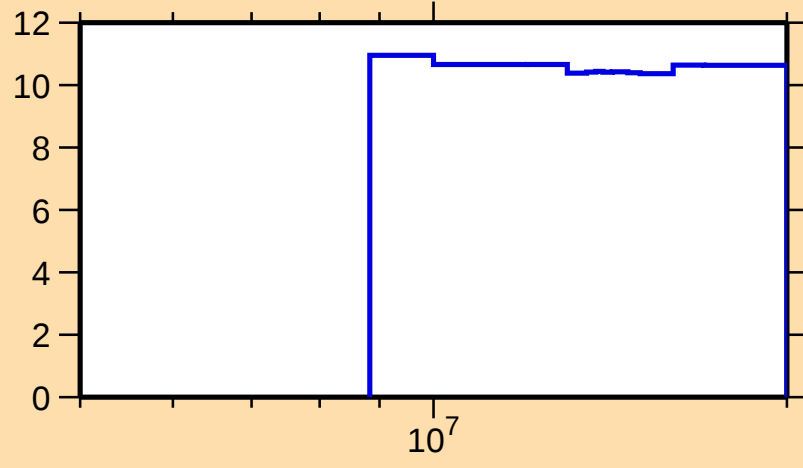
\Delta\sigma/\sigma vs. E for ^{213}\text{Hg}(n,\text{nonel.})
