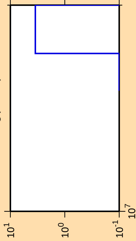
\Delta\sigma/\sigma vs. E for ^{213}\text{Hg} (mt 11)
