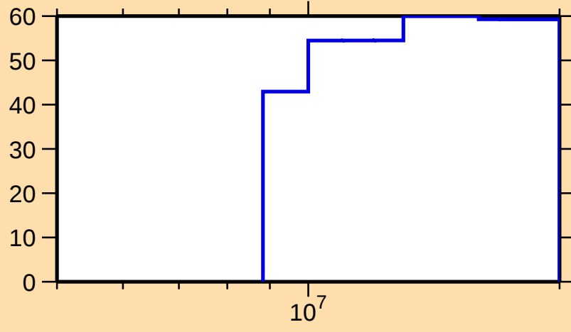
\Delta\sigma/\sigma vs. E for ^{213}\text{Hg}(n,2n)
