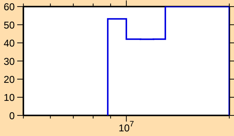
\Delta\sigma/\sigma vs. E for ^{213}\text{Hg}(n,\gamma)
