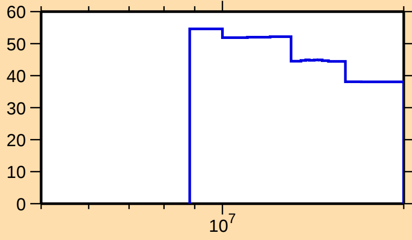
\Delta\sigma/\sigma vs. E for ^{213}\text{Hg}(n,n\text{cont.})
