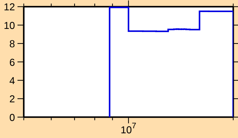
\Delta\sigma/\sigma vs. E for ^{213}\text{Hg}(n,\text{el.})
