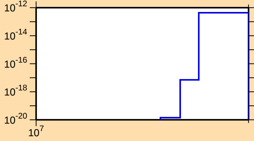
\sigma vs. E for ^{213}\text{Hg} (mt 11)
