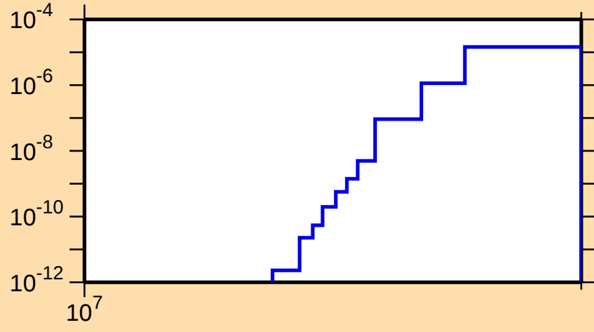
\sigma vs. E for ^{213}\text{Hg}(n,\text{nt})
