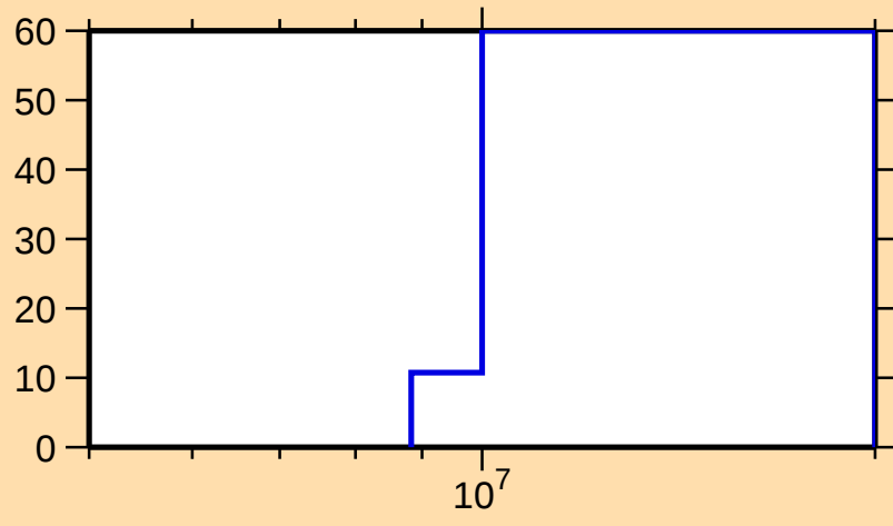
\Delta\sigma/\sigma vs. E for ^{213}\text{Hg}(n,p)
