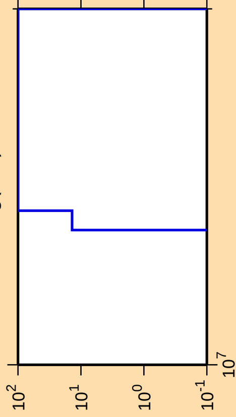
\Delta\sigma/\sigma vs. E for ^{213}\text{Hg}(n,\text{nt})
