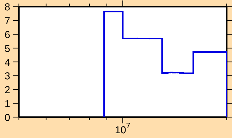
\Delta\sigma/\sigma vs. E for ^{213}\text{Hg}(n,\text{tot.})
