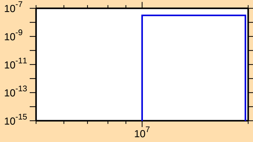
\sigma vs. E for ^{213}\text{Hg}(n,2n\alpha)
