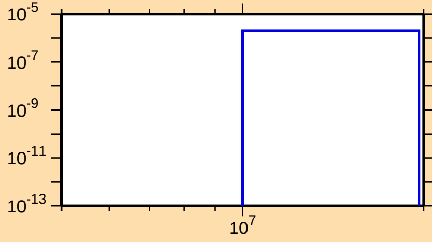
\sigma vs. E for ^{213}\text{Hg}(n,d)
