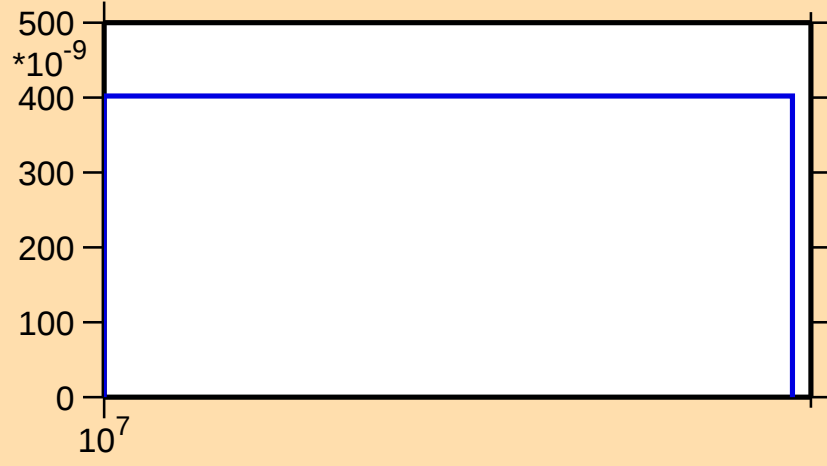
\sigma vs. E for ^{213}\text{Hg}(n,np)
