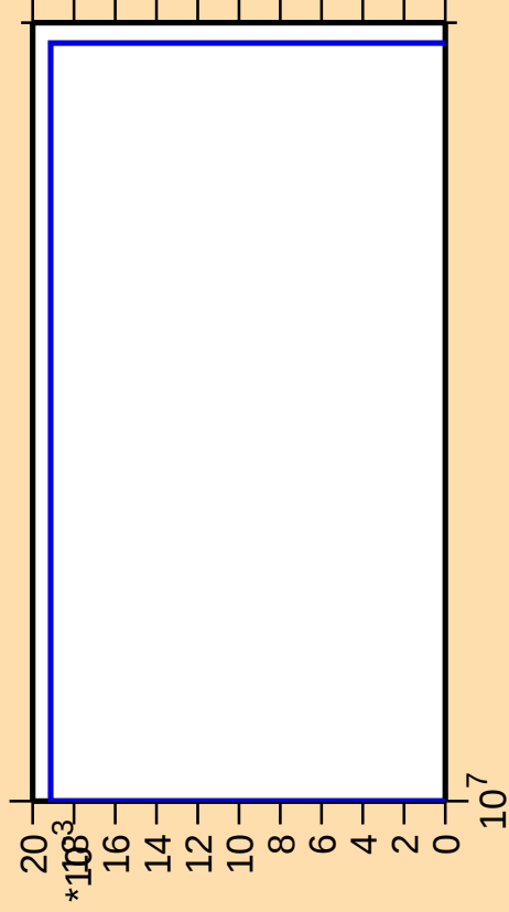
\Delta\sigma/\sigma vs. E for ^{213}\text{Hg} (mt 11)
