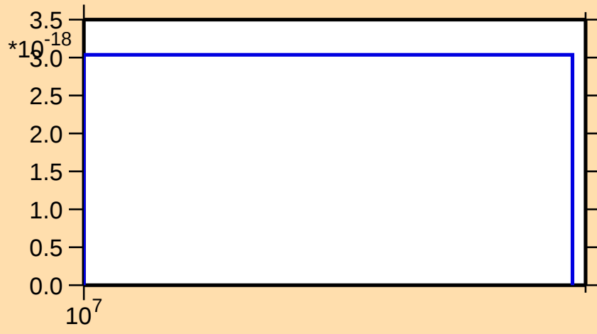
\sigma vs. E for ^{213}\text{Hg} (mt 42)
