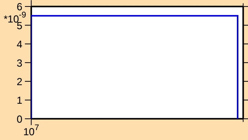
\sigma vs. E for ^{213}\text{Hg}(n,\text{nd})
