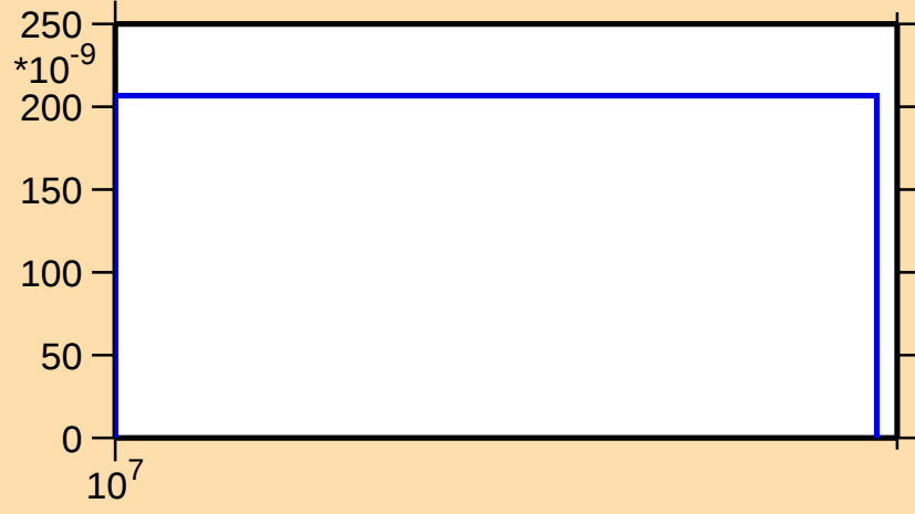
\sigma vs. E for ^{213}\text{Hg}(n,\text{nt})
