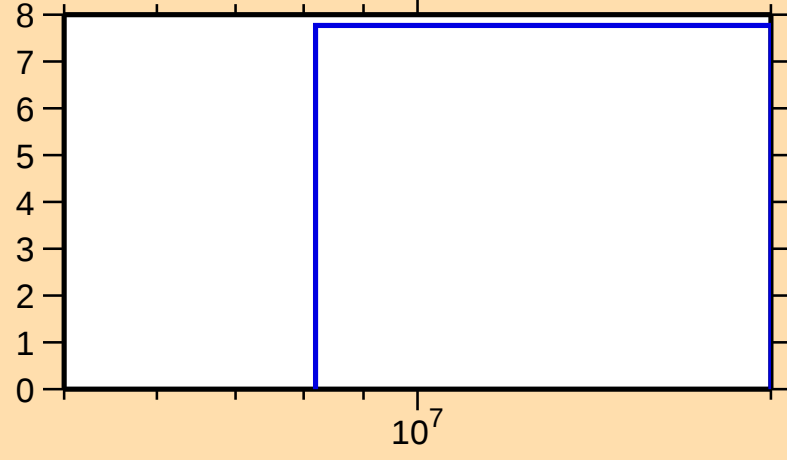
\Delta\sigma/\sigma vs. E for ^{213}\text{Hg}(n,\text{el.})
