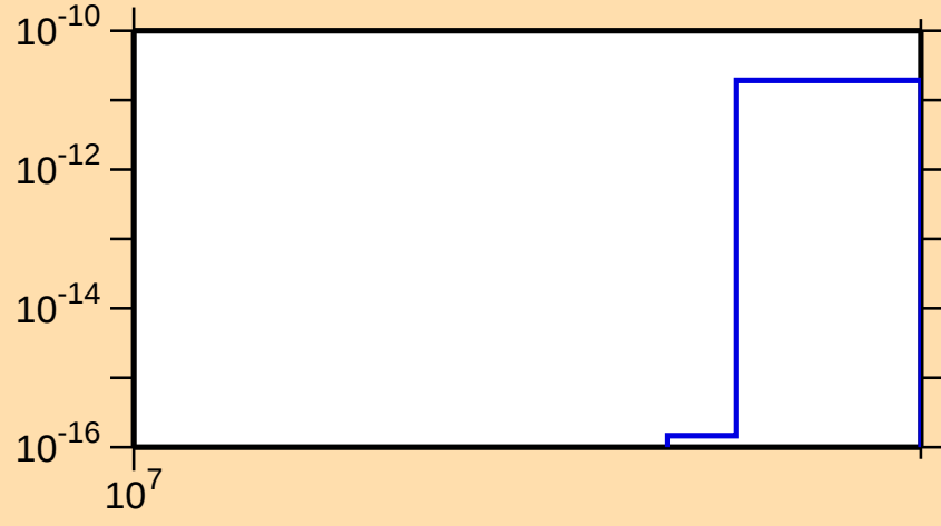
\sigma vs. E for ^{147}\text{Ho}(n,\text{nt})
