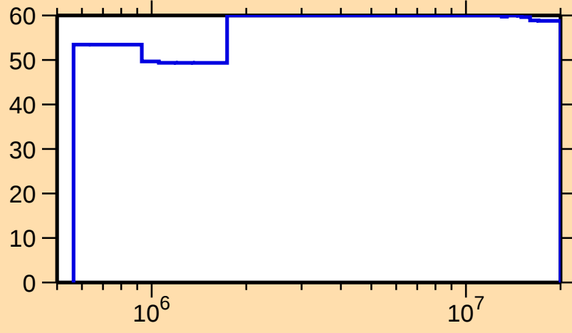
\Delta\sigma/\sigma vs. E for ^{147}\text{Ho}(n,n_1)
