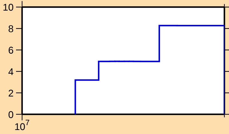
\Delta\sigma/\sigma vs. E for ^{147}\text{Ho}(n,\text{tot.})
