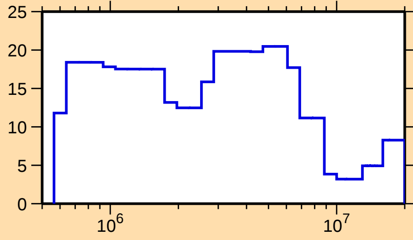
\Delta\sigma/\sigma vs. E for ^{147}\text{Ho}(n,\text{tot.})
