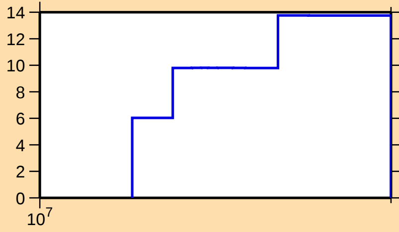
\Delta\sigma/\sigma vs. E for ^{147}\text{Ho}(n,\text{el.})
