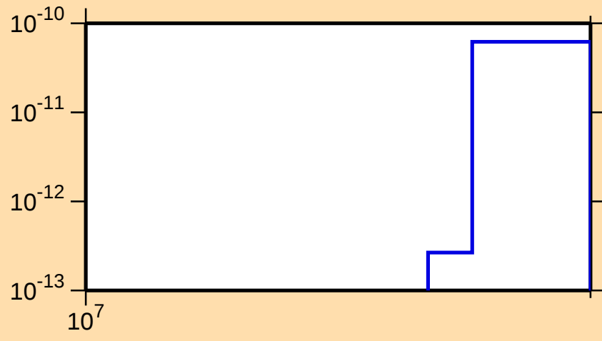
\sigma vs. E for ^{147}\text{Ho}(n,2n\alpha)
