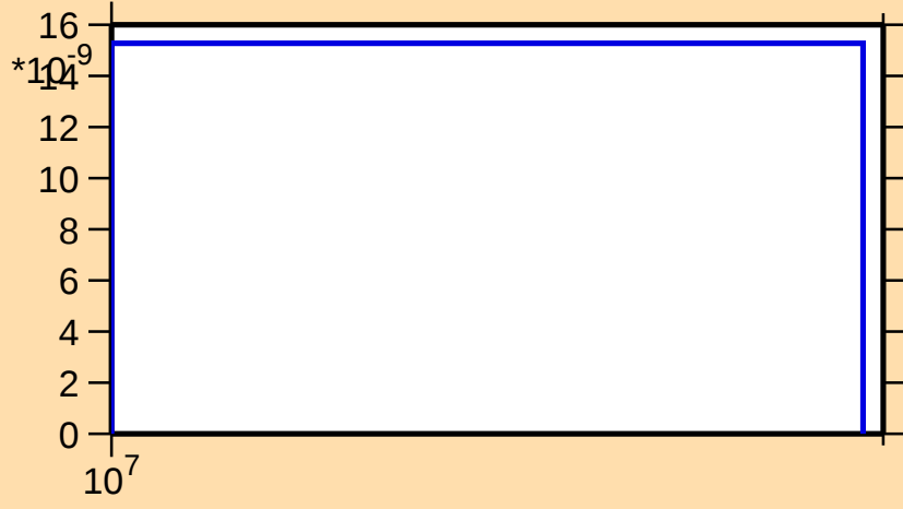
\sigma vs. E for ^{147}\text{Ho}(n,\text{nd})
