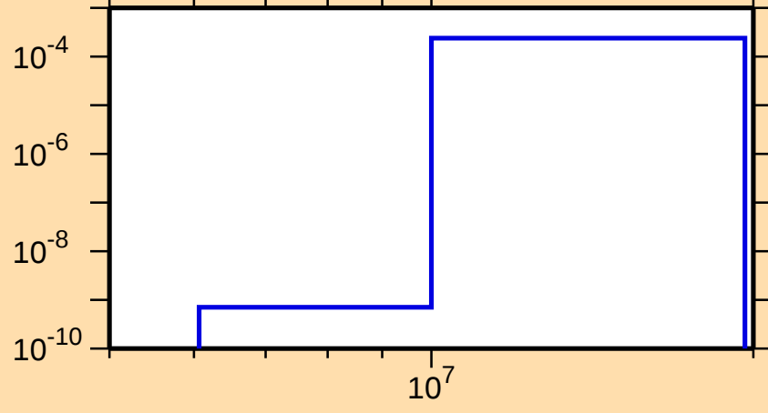
\sigma vs. E for ^{147}\text{Ho}(n,\text{pd})
