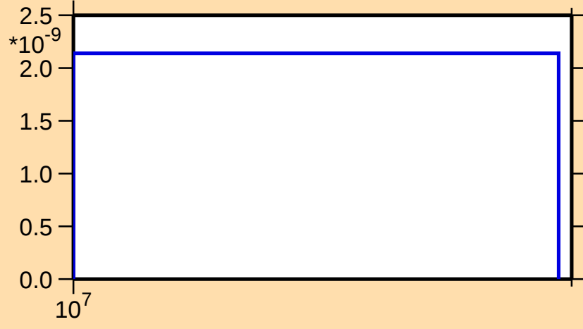
\sigma vs. E for ^{147}\text{Ho}(n,\text{pt})
