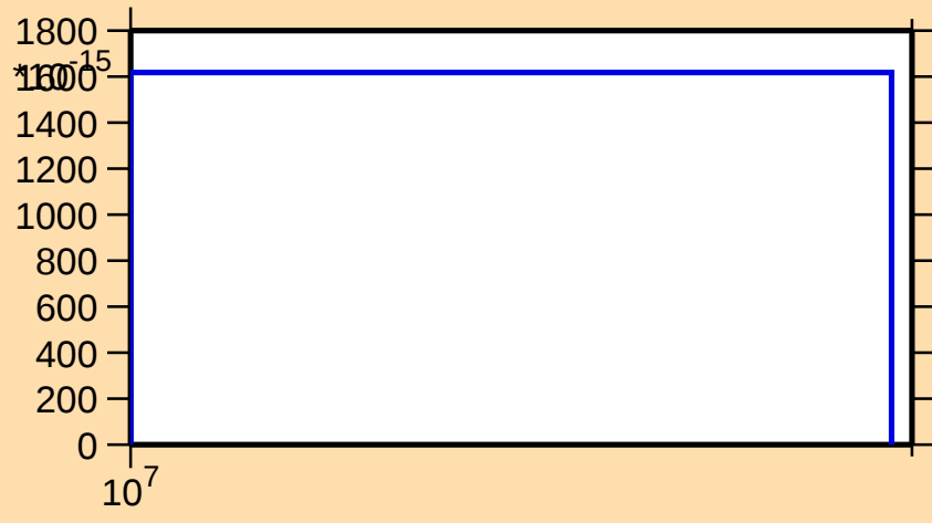
\sigma vs. E for ^{147}\text{Ho} (mt 34)
