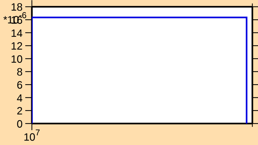
\sigma vs. E for ^{147}\text{Ho}(n,2np)
