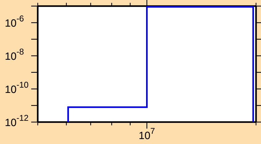
\sigma vs. E for ^{147}\text{Ho} (mt 45)
