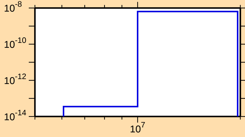
\sigma vs. E for ^{147}\text{Ho}(\text{mt117})
