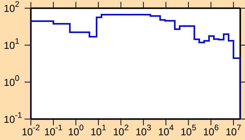
\Delta\sigma/\sigma vs. E for ^{147}\text{Ho}(\text{n,tot.})
