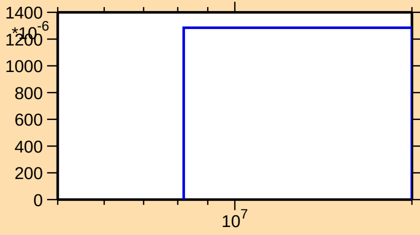
\sigma vs. E for ^{147}\text{Ho}(n,2n)
