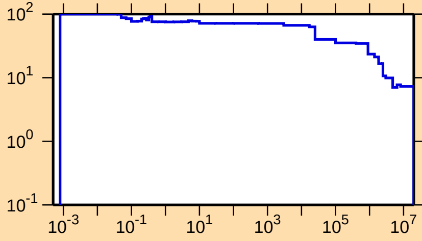
\Delta\sigma/\sigma vs. E for ^{147}\text{Ho}(n,\text{nonel.})
