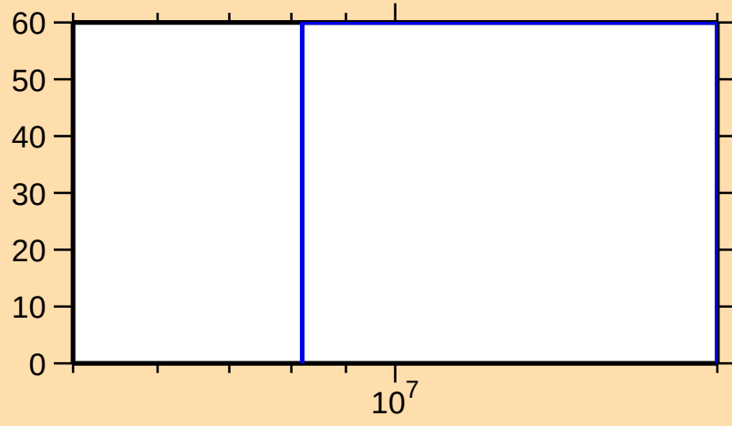
\Delta\sigma/\sigma vs. E for ^{147}\text{Ho}(n,2n)
