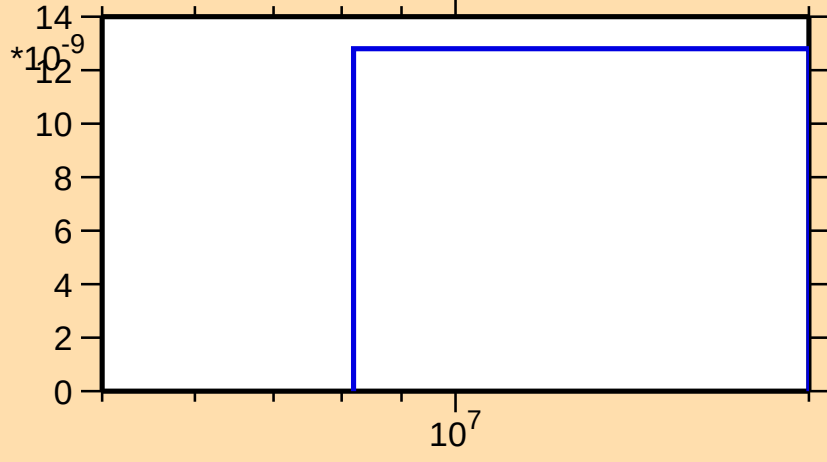
\sigma vs. E for ^{147}\text{Ho}(n,\text{nd})
