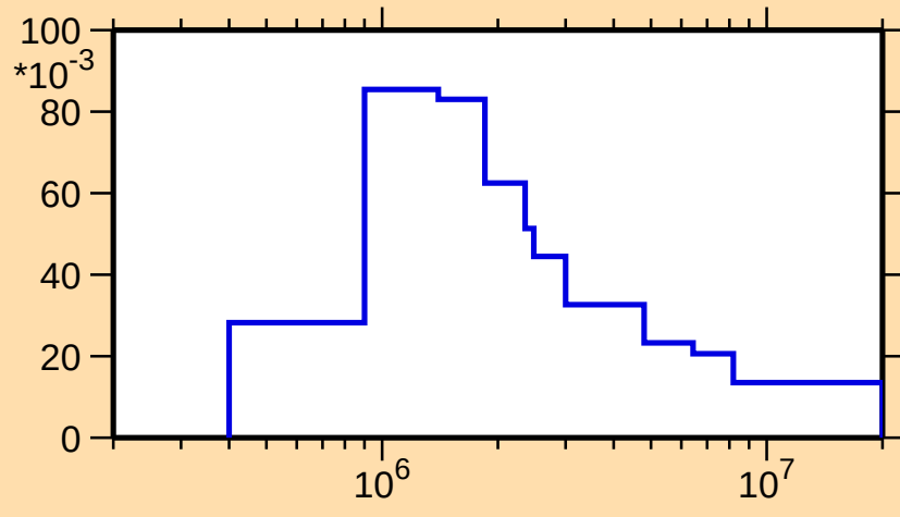
\sigma vs. E for ^{147}\text{Ho}(n,n_1)
