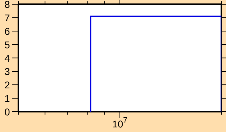
\Delta\sigma/\sigma vs. E for ^{147}\text{Ho}(n,\text{el.})
