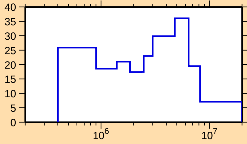
\Delta\sigma/\sigma vs. E for ^{147}\text{Ho}(n,\text{el.})
