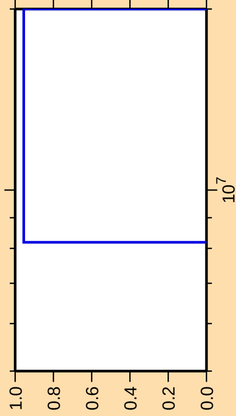
\Delta\sigma/\sigma vs. E for ^{147}\text{Ho}(n,nt)
