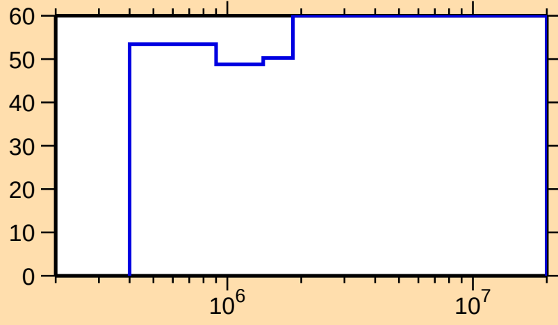
\Delta\sigma/\sigma vs. E for ^{147}\text{Ho}(n,n_1)
