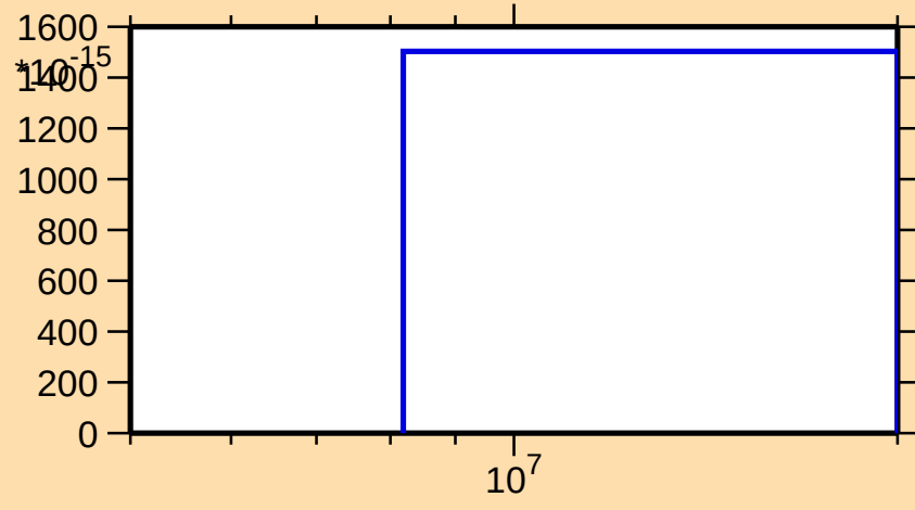
\sigma vs. E for ^{147}\text{Ho} (mt 34)
