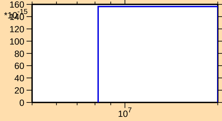
\sigma vs. E for ^{147}\text{Ho}(n,nt)
