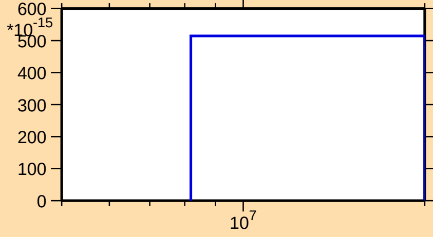
\sigma vs. E for ^{147}\text{Ho}(n,2n\alpha)
