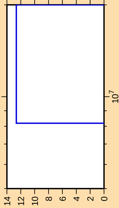
\Delta\sigma/\sigma vs. E for ^{147}\text{Ho} (mt 34)
