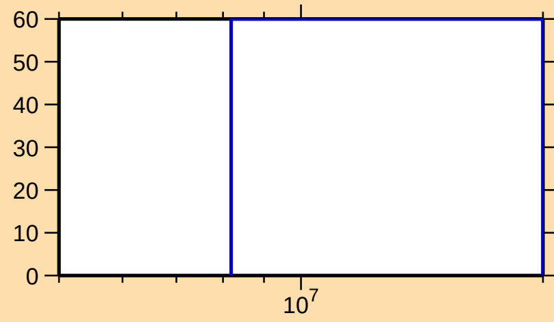
\Delta\sigma/\sigma vs. E for ^{147}\text{Ho}(n,2n)
