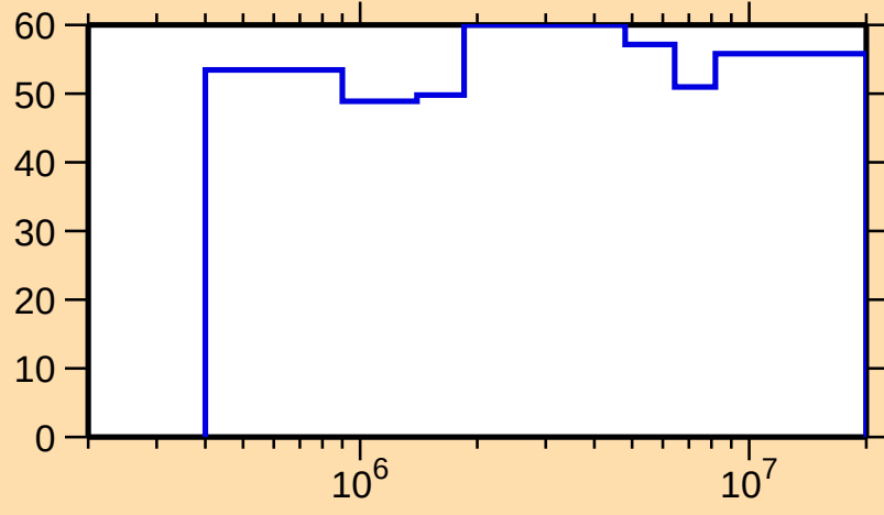
\Delta\sigma/\sigma vs. E for ^{147}\text{Ho}(n,\text{inel.})
