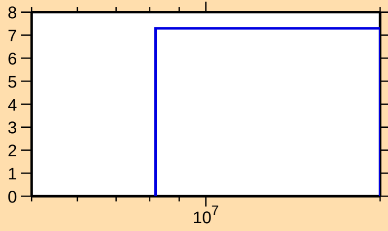
\Delta\sigma/\sigma vs. E for ^{147}\text{Ho}(n,\text{nonel.})
