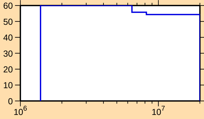
\Delta\sigma/\sigma vs. E for ^{147}\text{Ho}(n,n\text{cont.})
