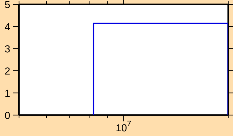
\Delta\sigma/\sigma vs. E for ^{147}\text{Ho}(n,\text{tot.})
