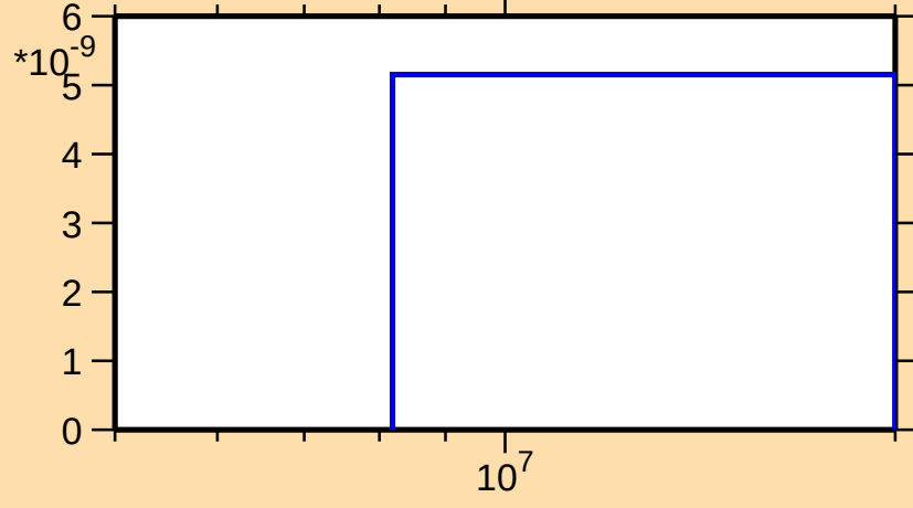
\sigma vs. E for ^{147}\text{Ho}(\text{mt117})
