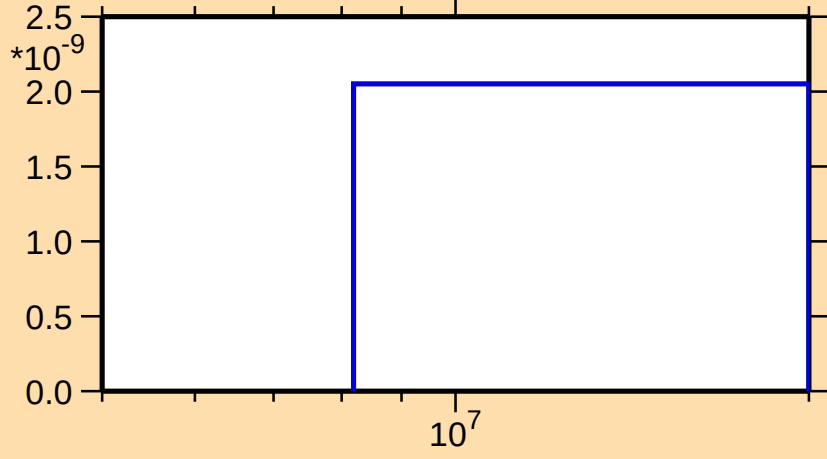
\sigma vs. E for ^{147}\text{Ho}(n,\text{pt})
