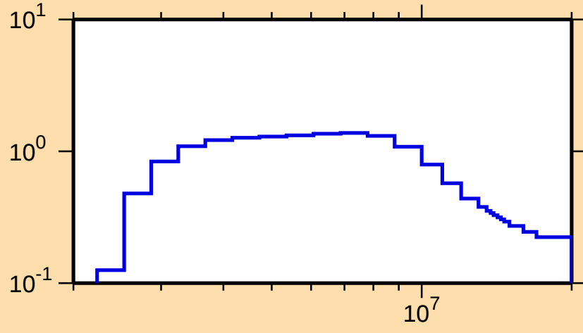
\sigma vs. E for ^{149}\text{Ho}(n,n\text{cont.})
