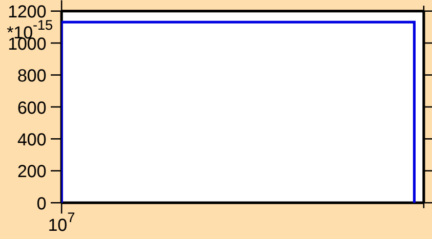
\sigma vs. E for ^{149}\text{Ho}(\text{mt } 34)
