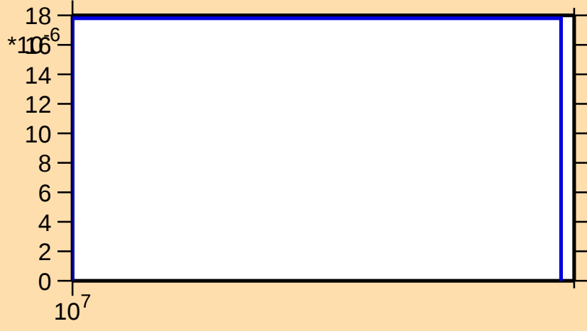
\sigma vs. E for ^{149}\text{Ho}(n,2np)
