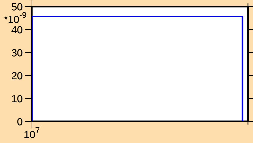
\sigma vs. E for ^{149}\text{Ho}(n,\text{nd})
