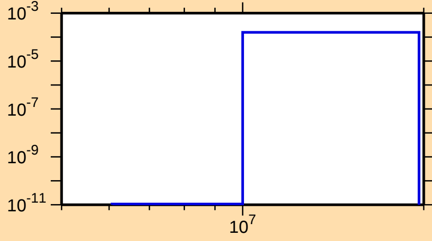
\sigma vs. E for ^{149}\text{Ho}(n,t)
