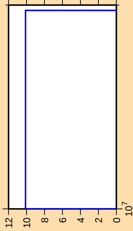
\Delta\sigma/\sigma vs. E for ^{149}\text{Ho}(\text{mt } 34)
