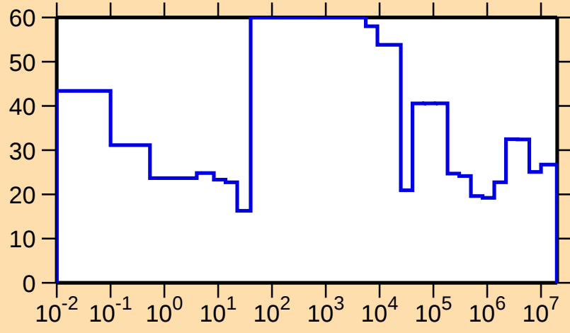
\Delta\sigma/\sigma vs. E for ^{149}\text{Ho}(n,\text{tot.})
