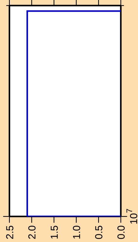
\Delta\sigma/\sigma vs. E for ^{149}\text{Ho}(n,\text{nt})
