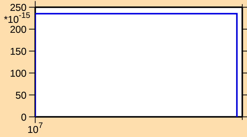
\sigma vs. E for ^{149}\text{Ho}(n,\text{nt})
