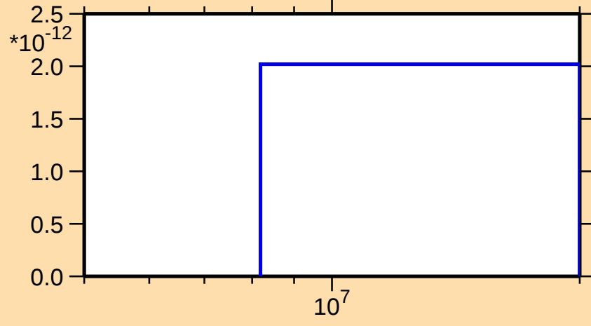
\sigma vs. E for ^{149}\text{Ho}(n,2n\alpha)
