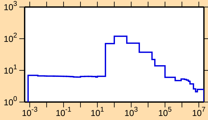
\sigma vs. E for ^{149}\text{Ho}(n,\text{el.})
