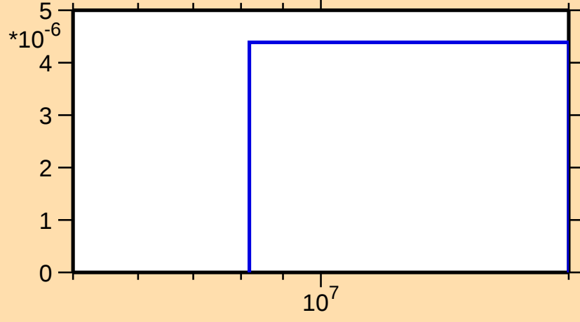
\sigma vs. E for ^{149}\text{Ho}(n,\text{pd})
