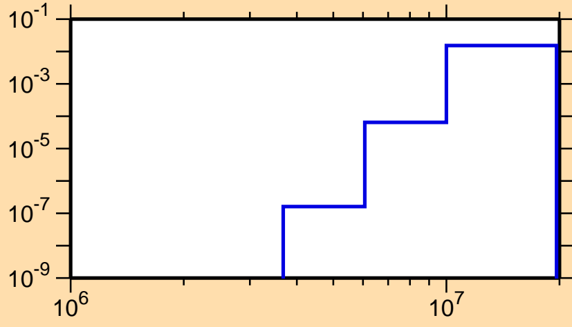
\sigma vs. E for ^{150}\text{Ho}(n,n\alpha)
