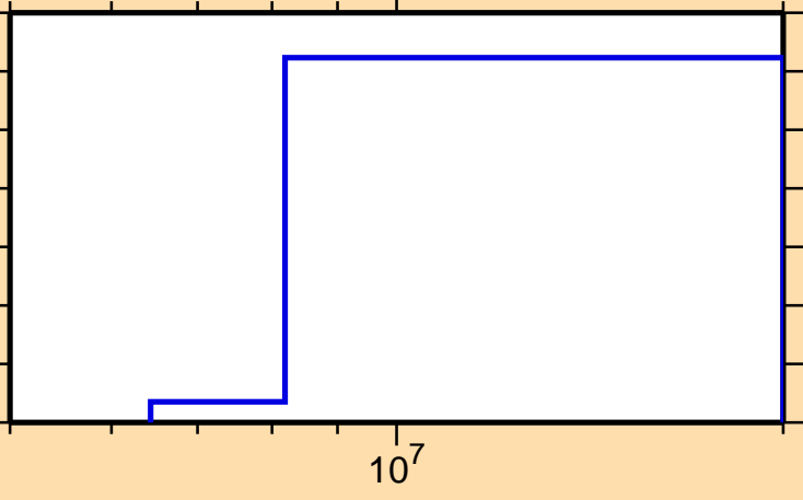
\sigma vs. E for ^{152}\text{Ho}(\text{mt117})
