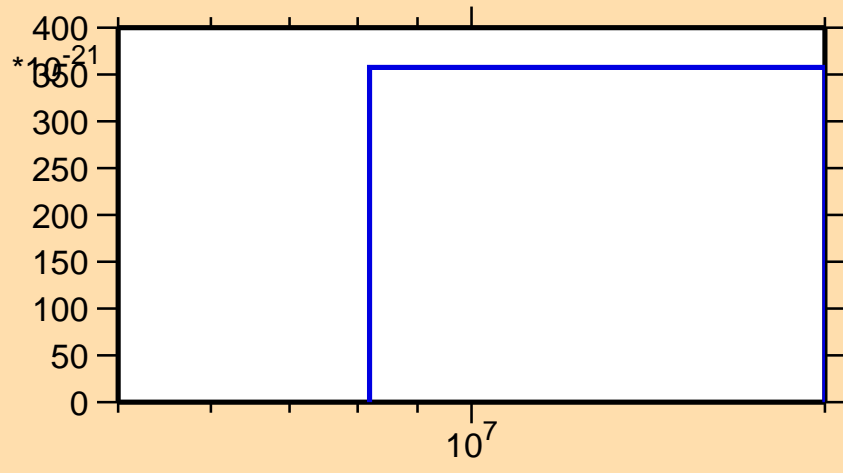
\sigma vs. E for ^{152}\text{Ho} (mt 42)
