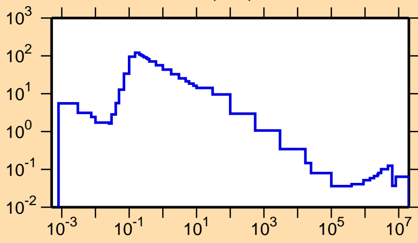
\sigma vs. E for ^{152}\text{Ho}(n,\alpha)
