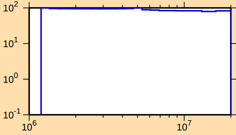
\Delta\sigma/\sigma vs. E for ^{152}\text{Ho}(n,n\text{cont.})
