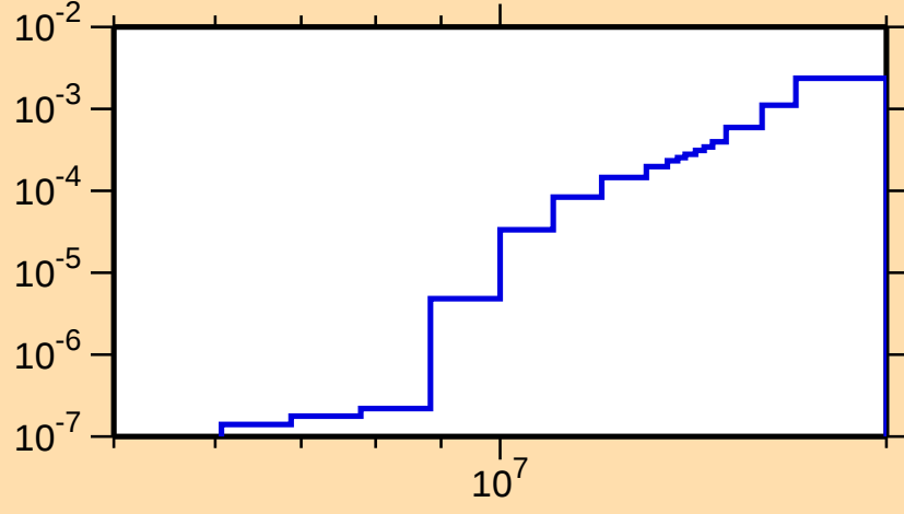
\sigma vs. E for ^{152}\text{Ho}(n,2n\alpha)
