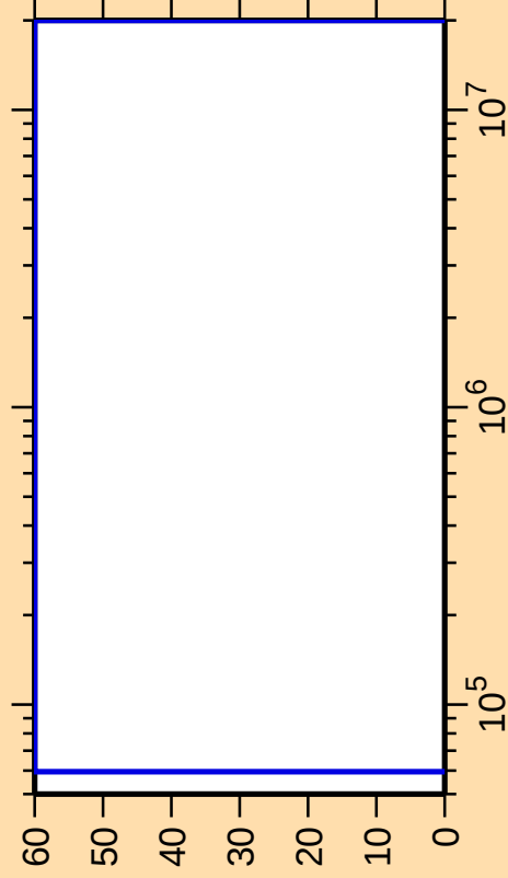
\Delta\sigma/\sigma vs. E for ^{152}\text{Ho}(n,\text{inel.})
