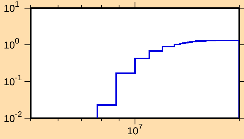
\sigma vs. E for ^{152}\text{Ho}(n,2n)
