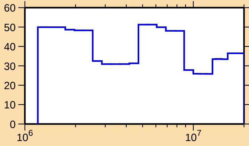
\Delta\sigma/\sigma vs. E for ^{152}\text{Ho}(n,\text{el.})
