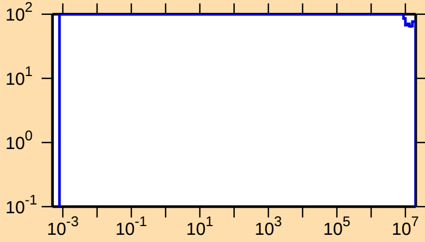
\Delta\sigma/\sigma vs. E for ^{152}\text{Ho}(n,p)
