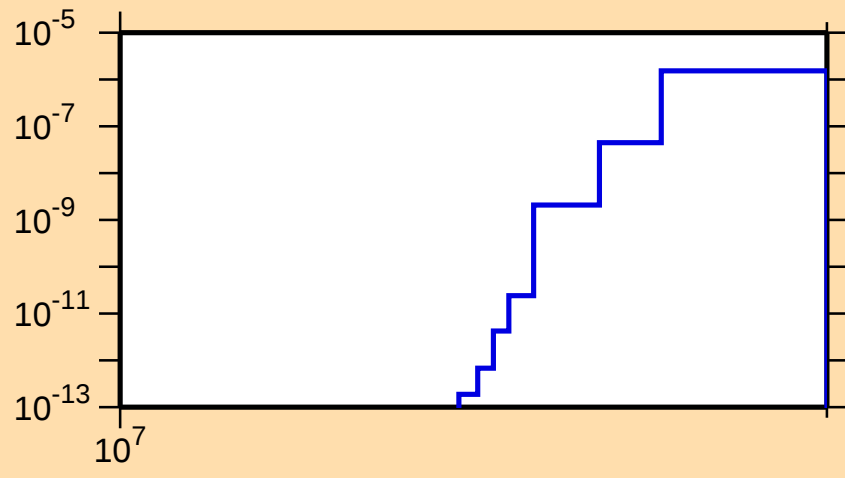
\sigma vs. E for ^{152}\text{Ho}(n,nt)
