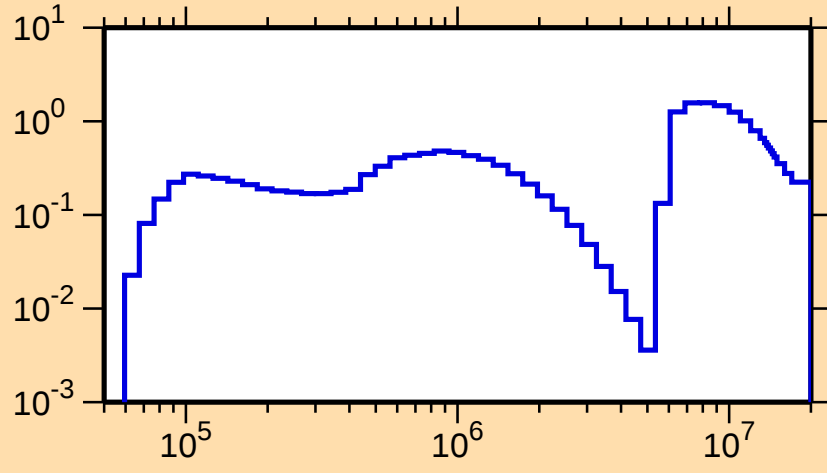
\sigma vs. E for ^{152}\text{Ho}(n,\text{inel.})
