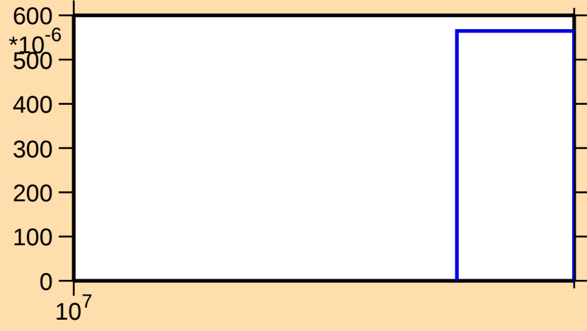
\sigma vs. E for ^{152}\text{Ho}(n,3n)
