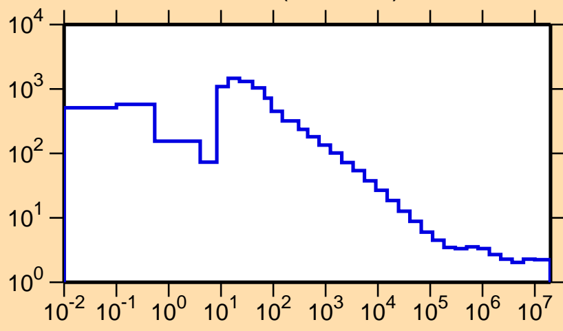
\sigma vs. E for ^{152}\text{Ho}(n,\text{nonel.})
