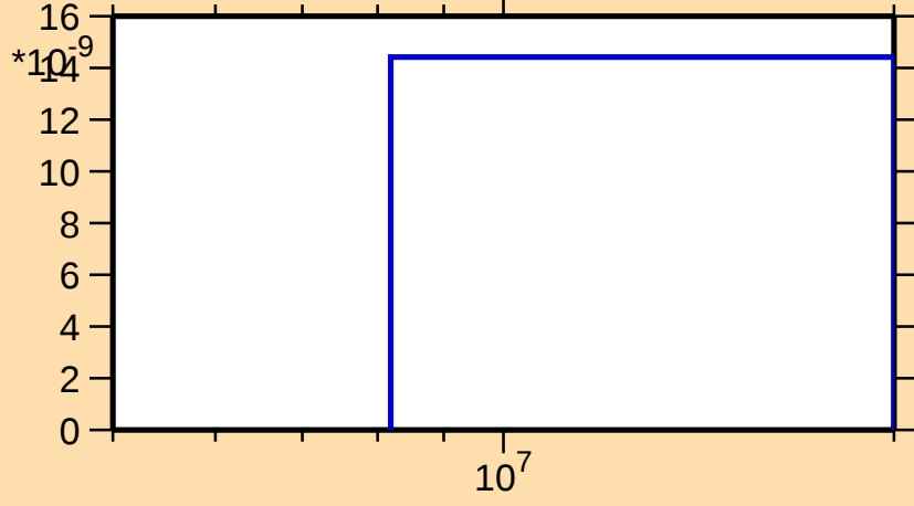
\sigma vs. E for ^{152}\text{Ho}(n,nt)
