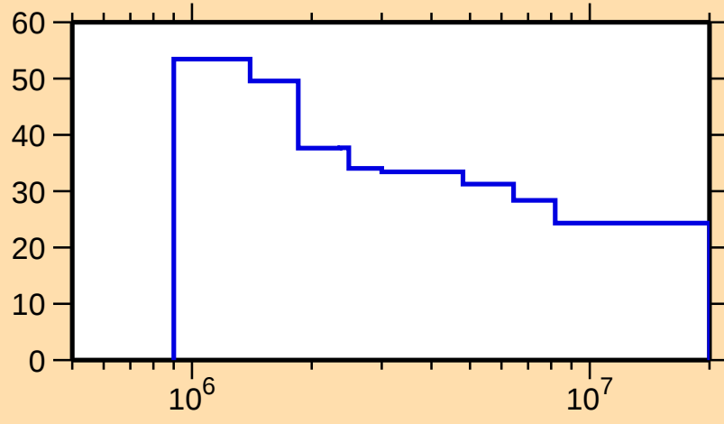
\Delta\sigma/\sigma vs. E for ^{152}\text{Ho}(n,\text{nonel.})
