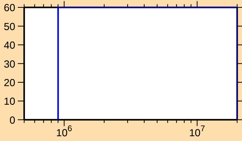
\Delta\sigma/\sigma vs. E for ^{152}\text{Ho}(n,n\text{cont.})
