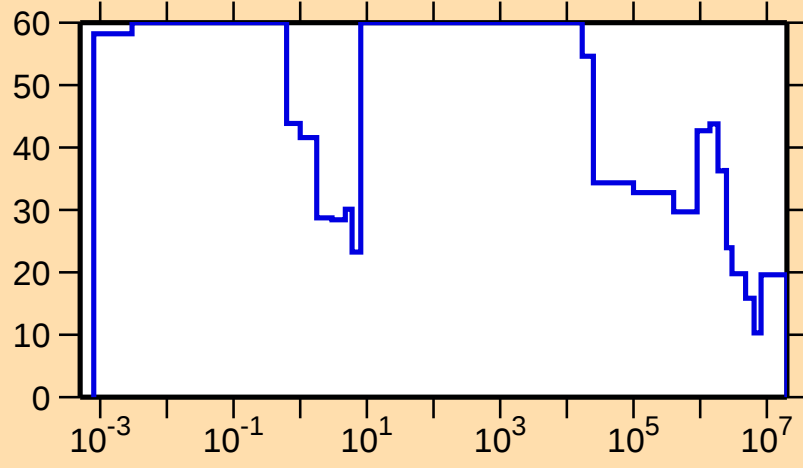
\Delta\sigma/\sigma vs. E for ^{152}\text{Ho}(n,\text{tot.})
