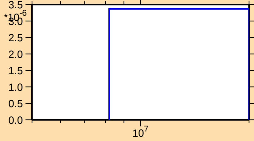
\sigma vs. E for ^{152}\text{Ho}(n,\text{nd})
