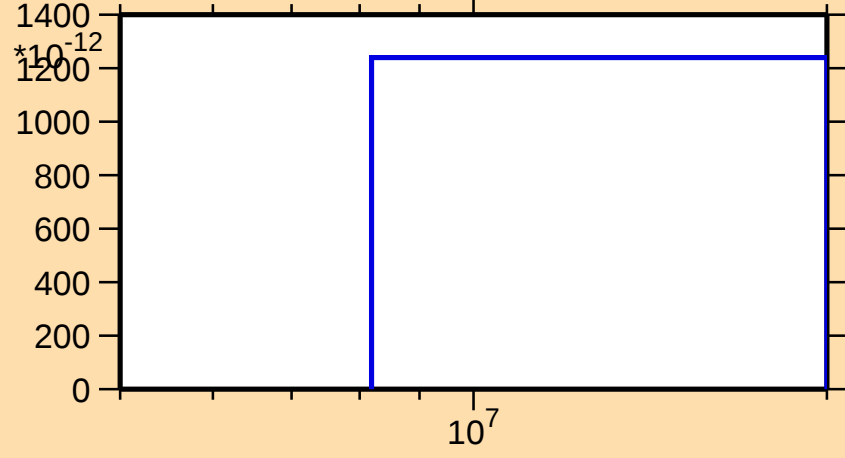
\sigma vs. E for ^{152}\text{Ho}(n,\text{pt})
