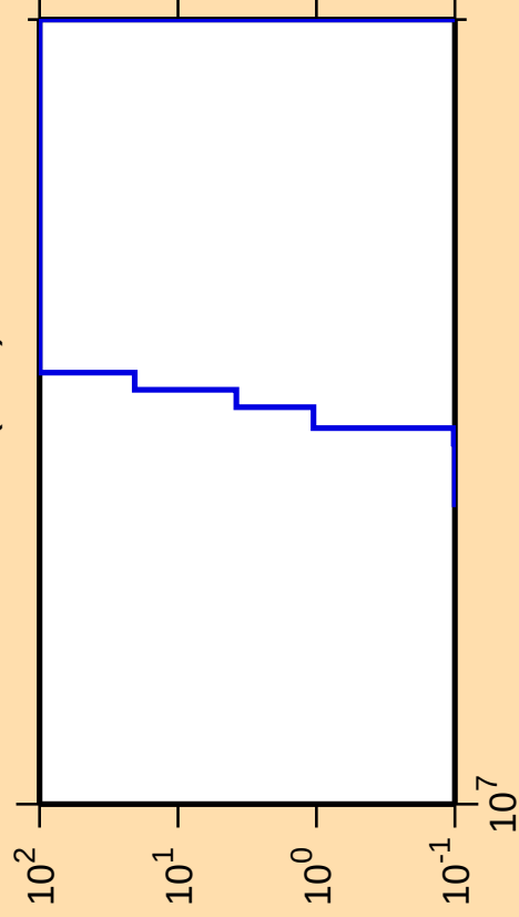
\Delta\sigma/\sigma vs. E for ^{153}\text{Ho}(n,\text{nt})
