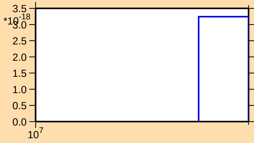
\sigma vs. E for ^{153}\text{Ho} (mt 42)
