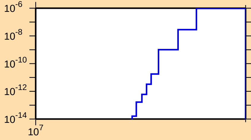
\sigma vs. E for ^{153}\text{Ho}(n,\text{nt})
