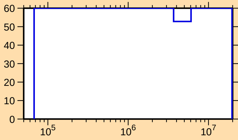
\Delta\sigma/\sigma vs. E for ^{153}\text{Ho}(n,n_1)
