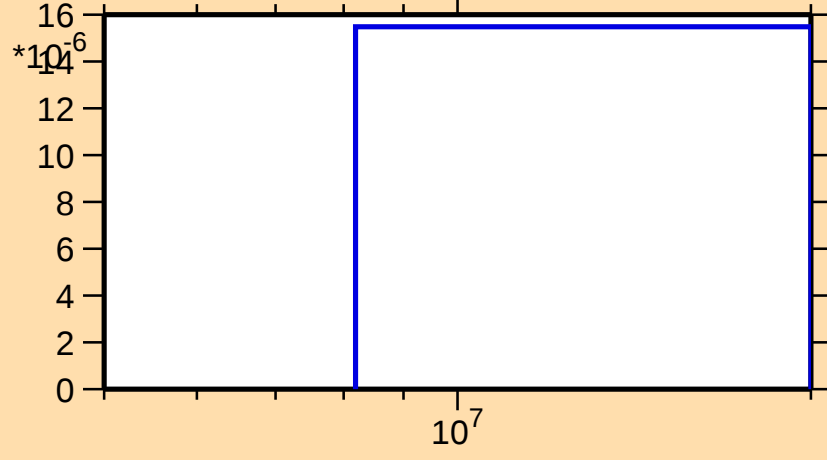
\sigma vs. E for ^{153}\text{Ho}(n,3n)
