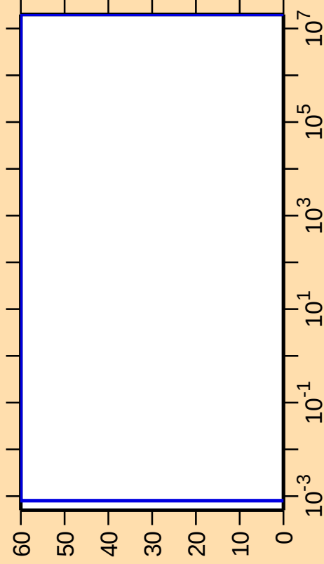
\Delta\sigma/\sigma vs. E for ^{153}\text{Ho}(n,\alpha)
