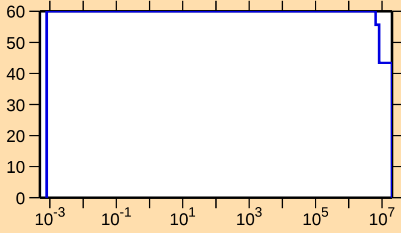
\Delta\sigma/\sigma vs. E for ^{153}\text{Ho}(n,p)
