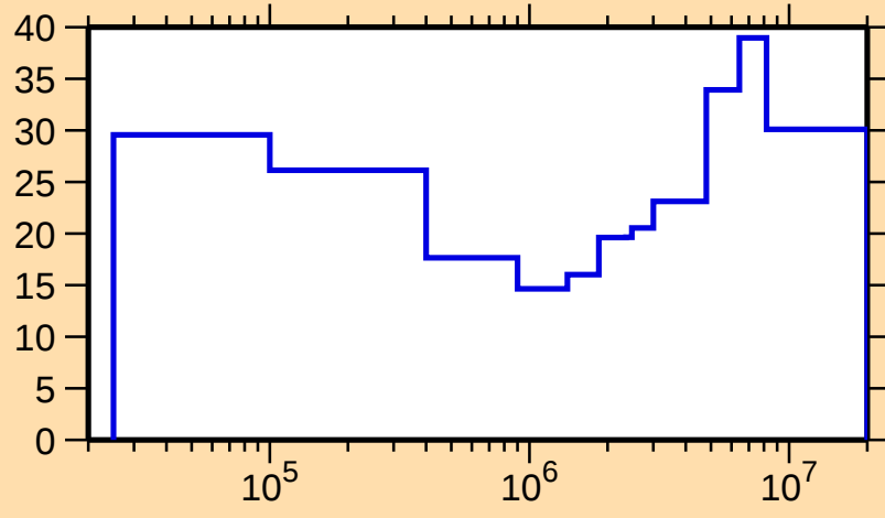
\Delta\sigma/\sigma vs. E for ^{153}\text{Ho}(n,\text{tot.})
