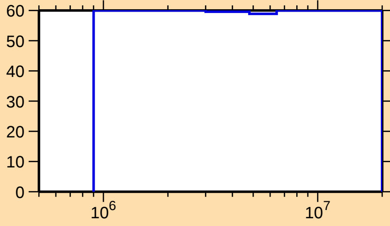
\Delta\sigma/\sigma vs. E for ^{153}\text{Ho}(n,n_1)
