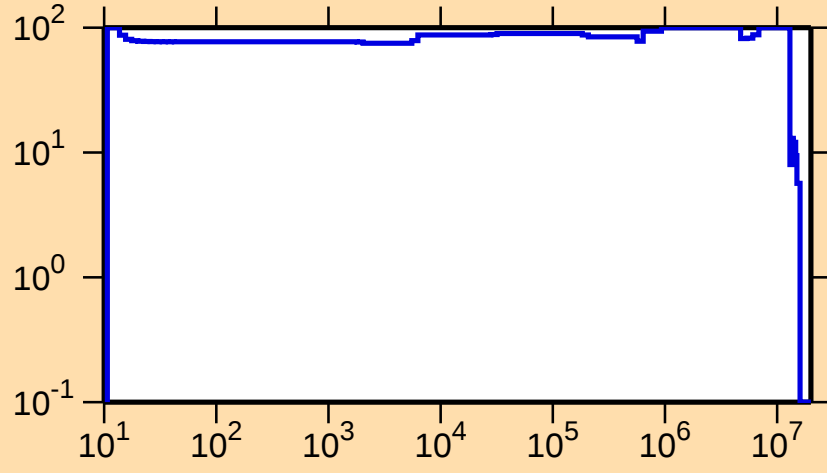
\Delta\sigma/\sigma vs. E for ^{154}\text{Ho}(n,n_1)
