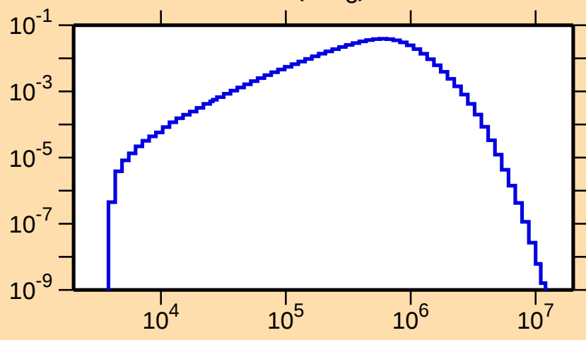
\sigma vs. E for ^{154}\text{Ho}(n,n_3)
