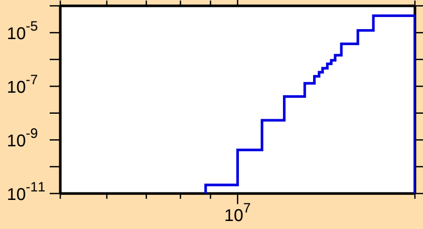
\sigma vs. E for ^{154}\text{Ho}(n,\text{He3})
