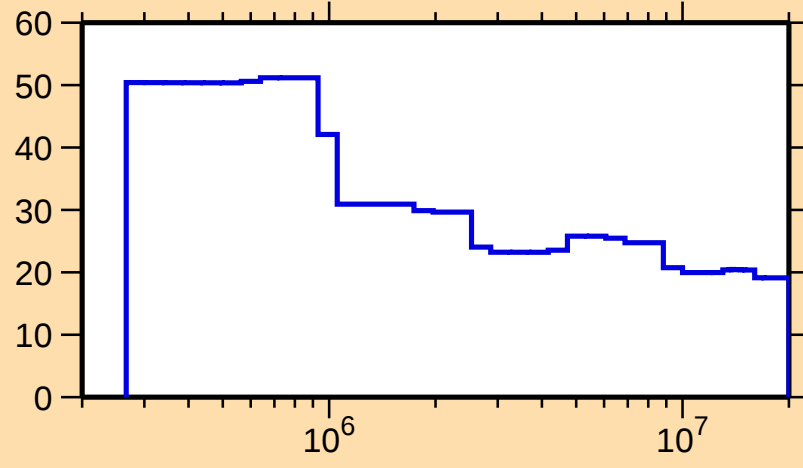
\Delta\sigma/\sigma vs. E for ^{154}\text{Ho}(n,n\text{onel.})
