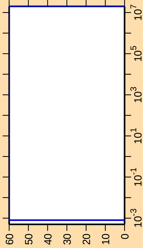
\Delta\sigma/\sigma vs. E for ^{154}\text{Ho}(n,\alpha)
