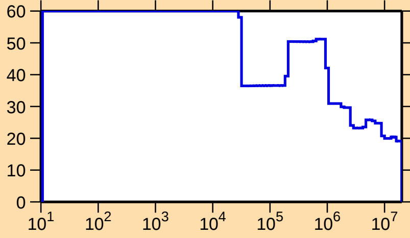
\Delta\sigma/\sigma vs. E for ^{154}\text{Ho}(n,\text{nonel.})
