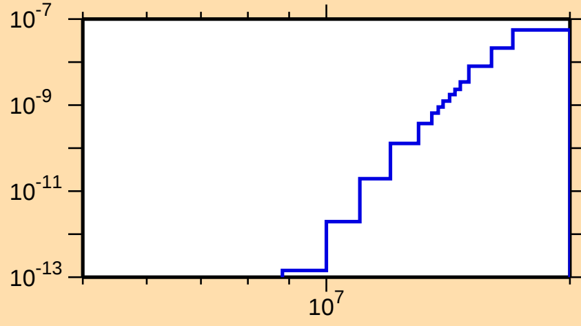
\sigma vs. E for ^{154}\text{Ho}(\text{mt117})
