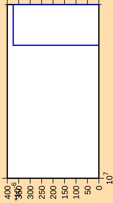
\Delta\sigma/\sigma vs. E for ^{154}\text{Ho} (mt 42)
