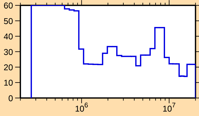
\Delta\sigma/\sigma vs. E for ^{154}\text{Ho}(n,\text{el.})
