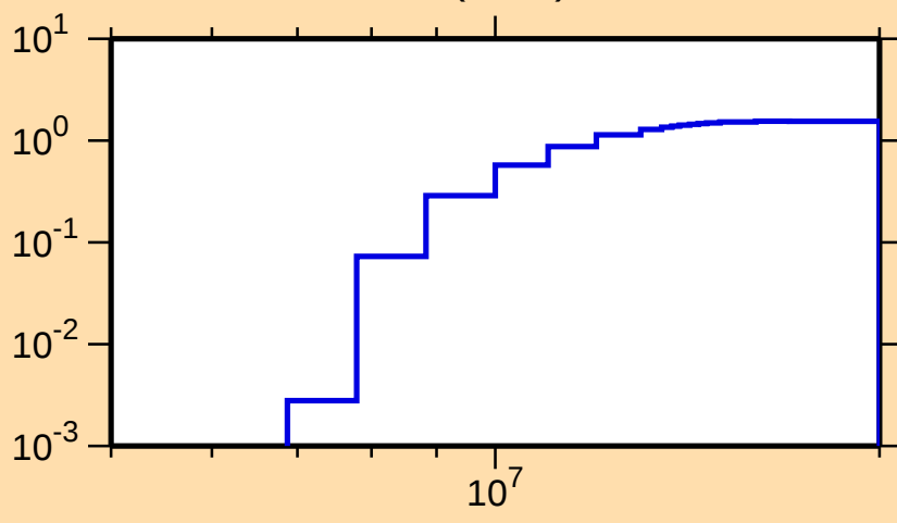
\sigma vs. E for ^{154}\text{Ho}(n,2n)
