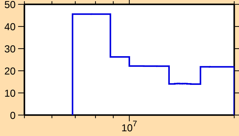
\Delta\sigma/\sigma vs. E for ^{154}\text{Ho}(n,\text{el.})
