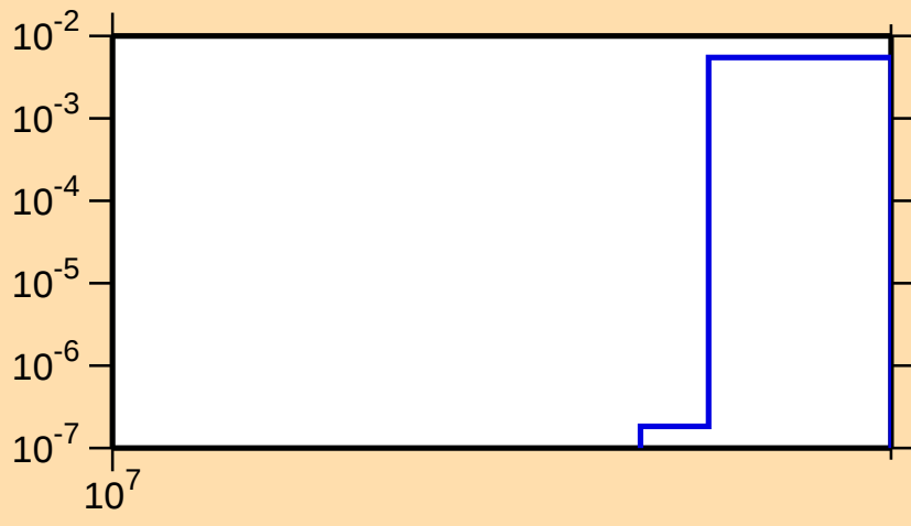
\sigma vs. E for ^{154}\text{Ho}(n,3n)
