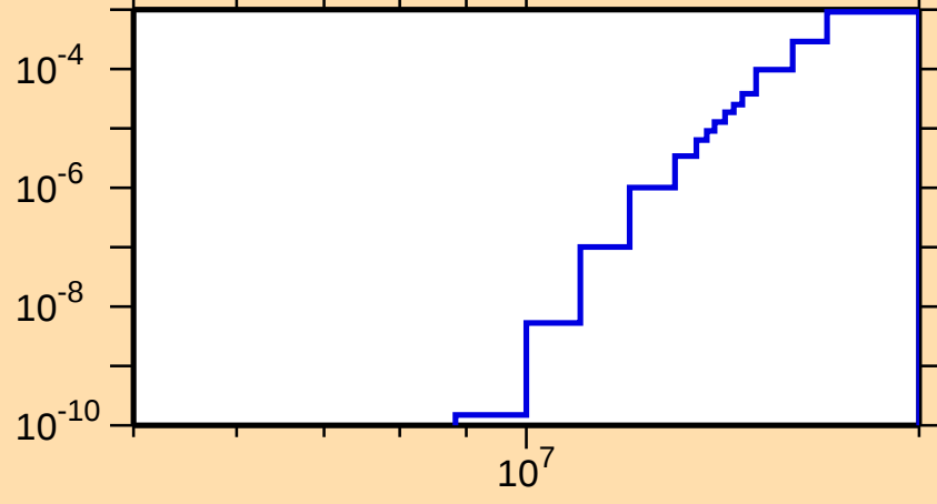
\sigma vs. E for ^{154}\text{Ho}(n,2n\alpha)
