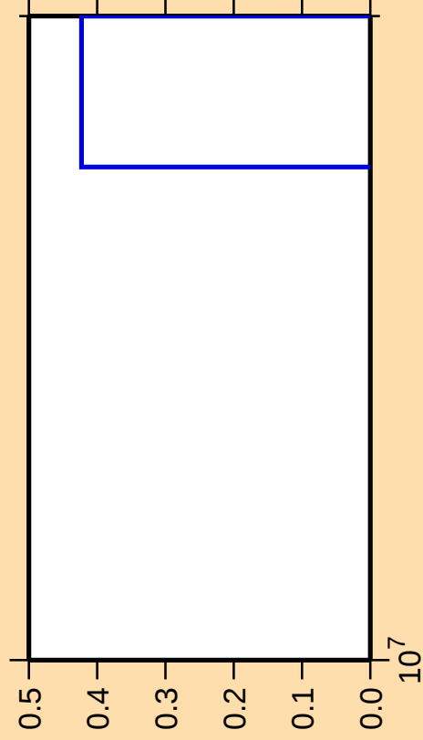
\Delta\sigma/\sigma vs. E for ^{154}\text{Ho} (mt 11)
