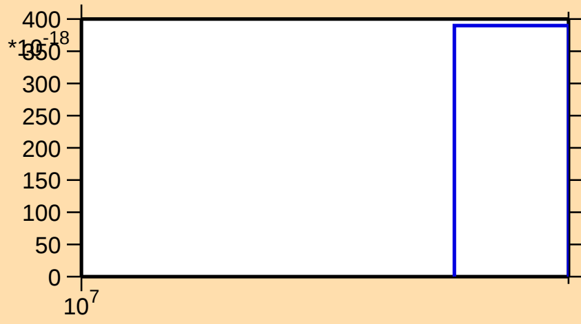
\sigma vs. E for ^{154}\text{Ho} (mt 42)
