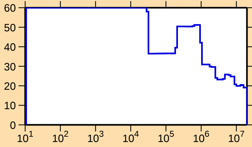
\Delta\sigma/\sigma vs. E for ^{154}\text{Ho}(n,\text{nonel.})
