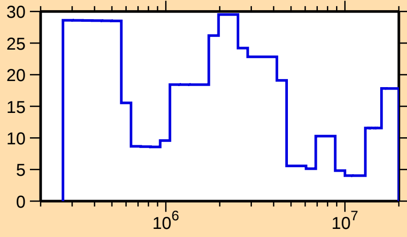
\Delta\sigma/\sigma vs. E for ^{154}\text{Ho}(n,\text{tot.})
