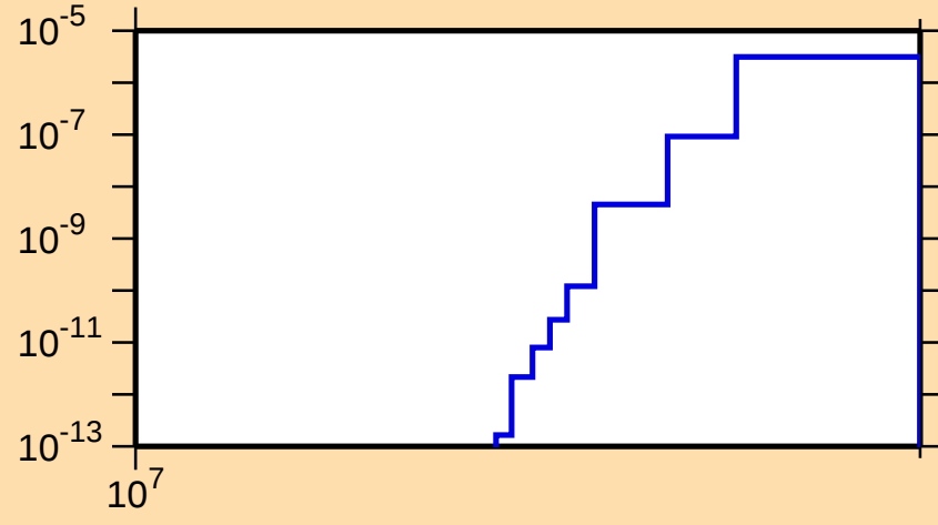
\sigma vs. E for ^{154}\text{Ho}(n,\text{nt})
