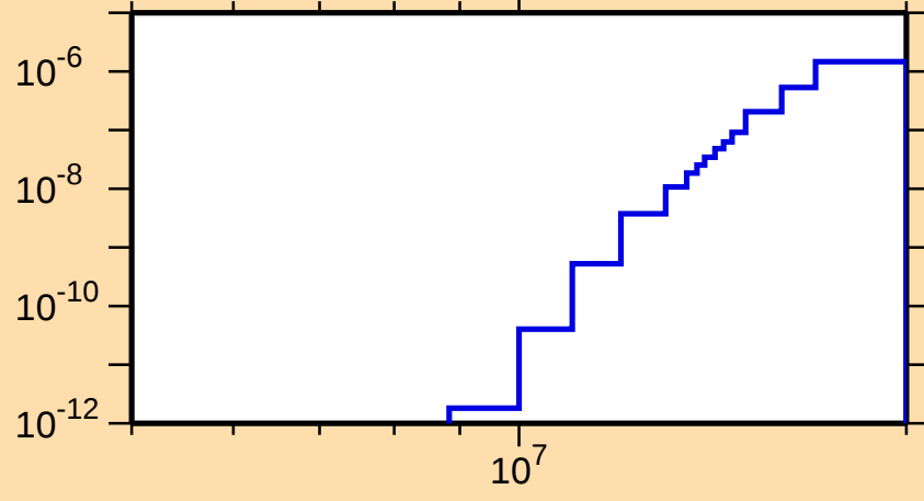
\sigma vs. E for ^{154}\text{Ho} (mt 45)
