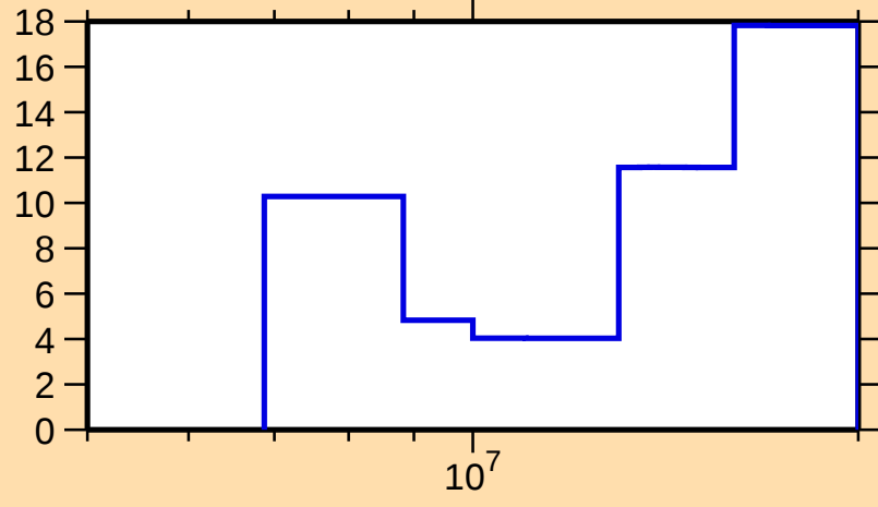
\Delta\sigma/\sigma vs. E for ^{154}\text{Ho}(n,\text{tot.})
