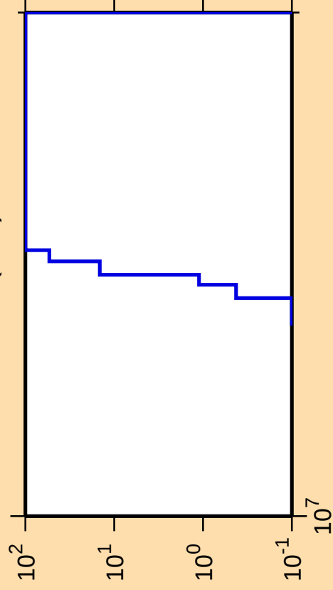
\Delta\sigma/\sigma vs. E for ^{154}\text{Ho}(n,\text{nt})
