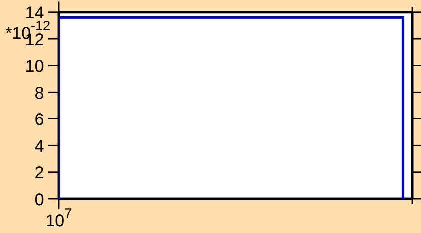
\sigma vs. E for ^{154}\text{Ho} (mt 34)
