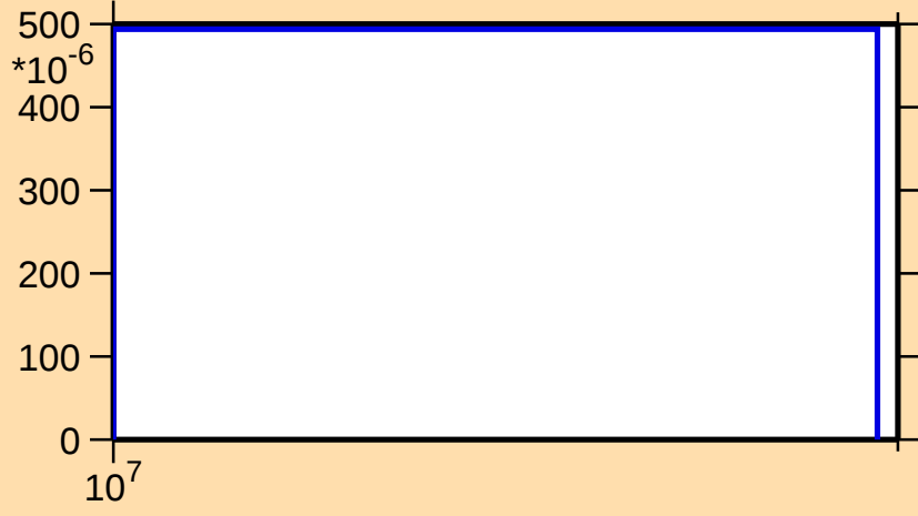
\sigma vs. E for ^{154}\text{Ho}(n,2np)
