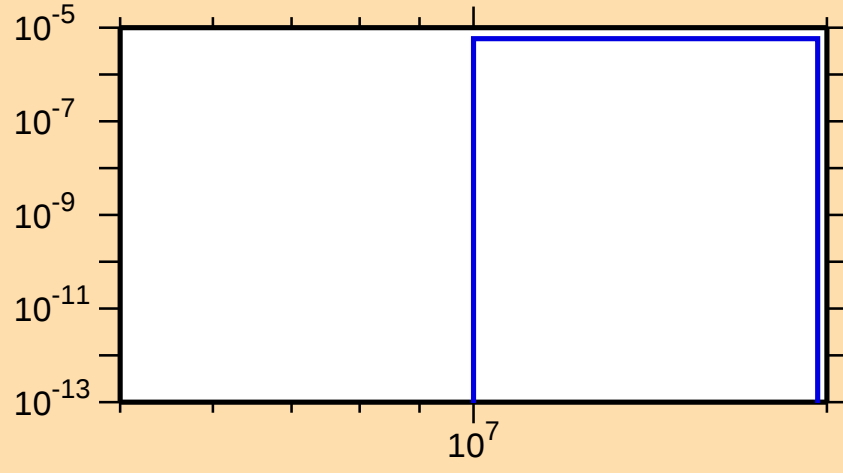
\sigma vs. E for ^{154}\text{Ho}(n,\text{nd})
