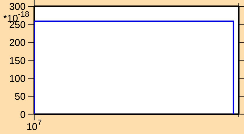
\sigma vs. E for ^{154}\text{Ho} (mt 11)
