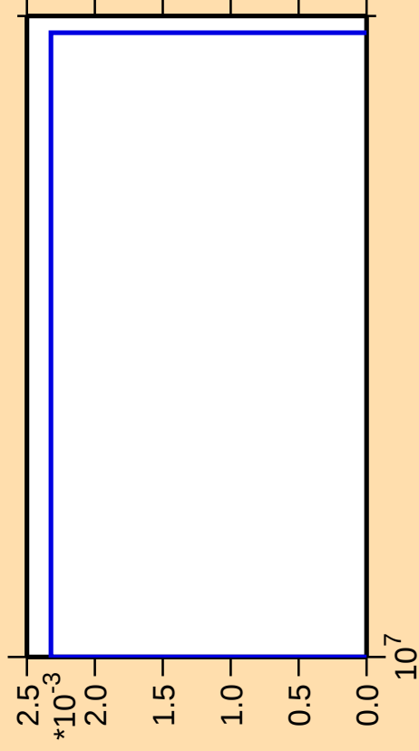
\Delta\sigma/\sigma vs. E for ^{154}\text{Ho} (mt 11)
