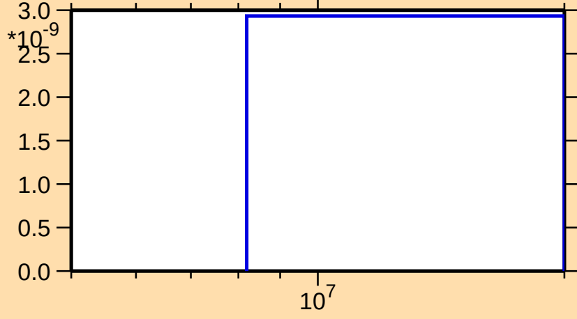
\sigma vs. E for ^{154}\text{Ho}(\text{mt117})
