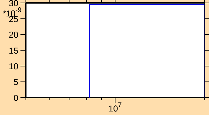
\sigma vs. E for ^{154}\text{Ho}(n,nt)
