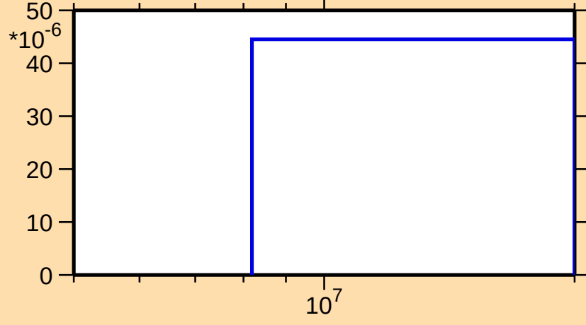
\sigma vs. E for ^{154}\text{Ho}(n,3n)
