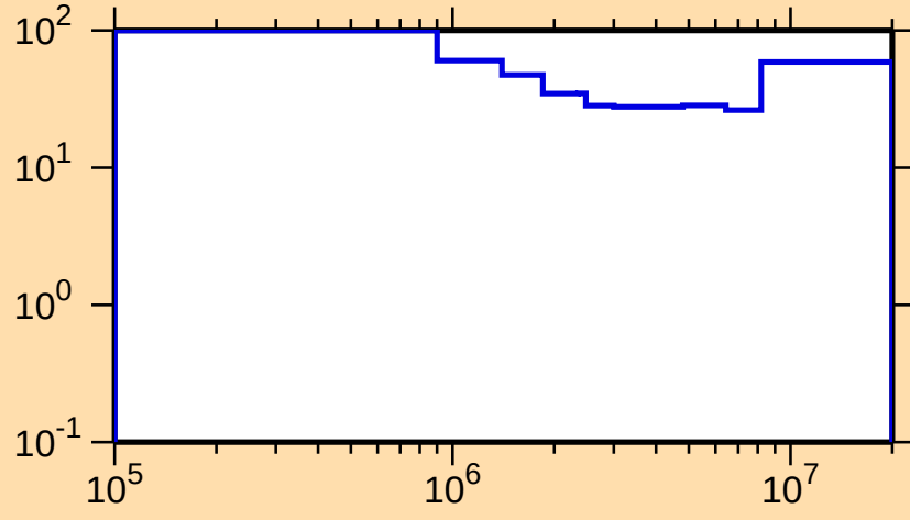
\Delta\sigma/\sigma vs. E for ^{154}\text{Ho}(n,n\text{cont.})
