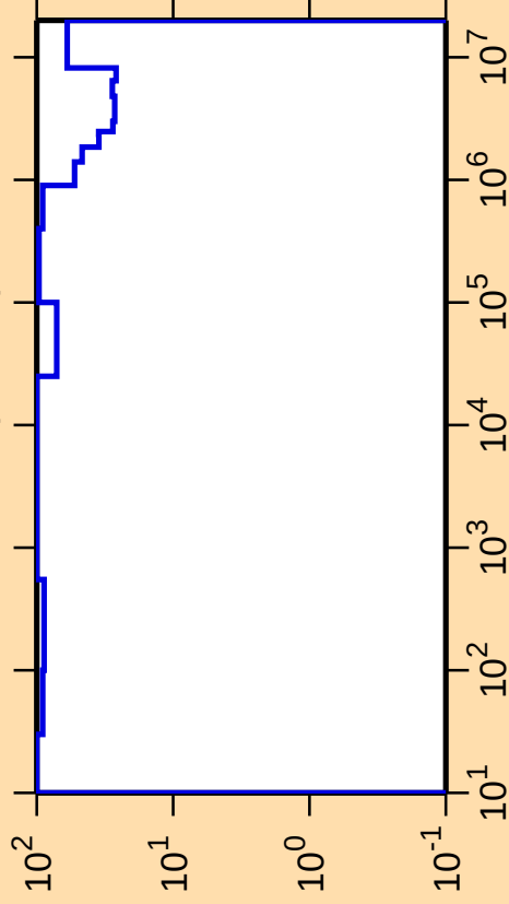
\Delta\sigma/\sigma vs. E for ^{154}\text{Ho}(n,\text{inel.})
