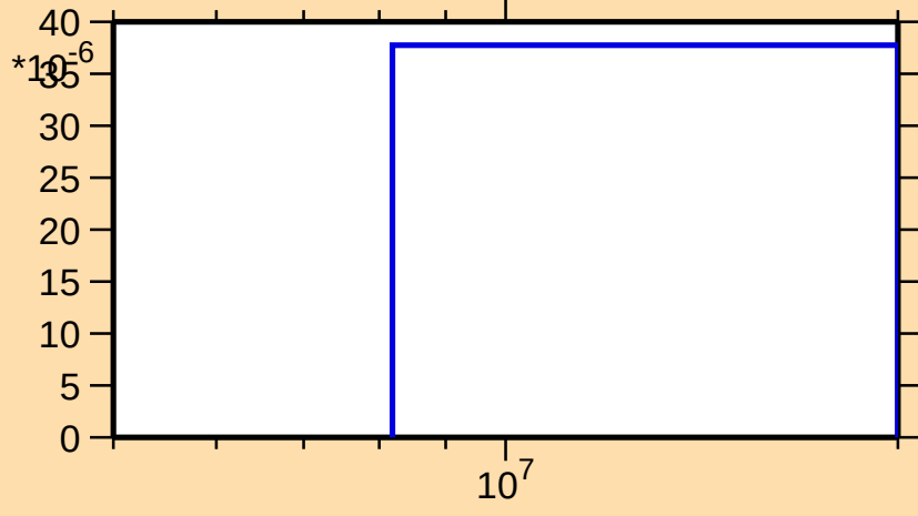
\sigma vs. E for ^{154}\text{Ho}(n,2n\alpha)
