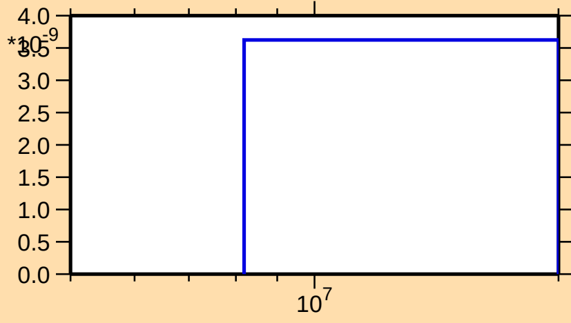
\sigma vs. E for ^{154}\text{Ho}(n,3n\alpha)
