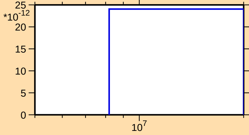
\sigma vs. E for ^{154}\text{Ho}(n,\text{pt})
