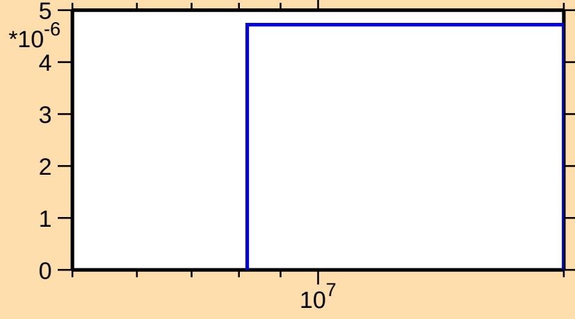
\sigma vs. E for ^{154}\text{Ho}(n,\text{nd})
