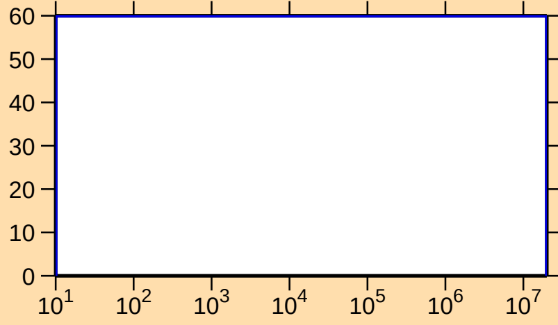
\Delta\sigma/\sigma vs. E for ^{154}\text{Ho}(n,n_1)
