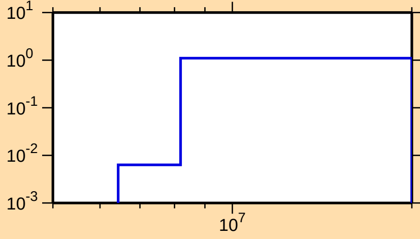
\sigma vs. E for ^{154}\text{Ho}(n,2n)
