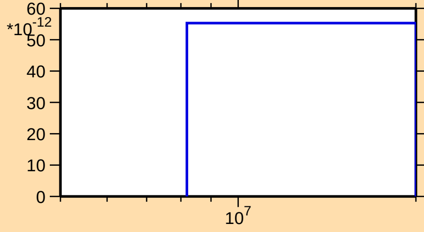
\sigma vs. E for ^{154}\text{Ho}(n,\text{pd})
