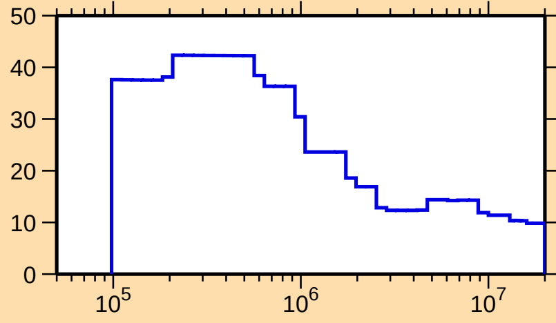
\Delta\sigma/\sigma vs. E for ^{155}\text{Ho}(n,\text{nonel.})
