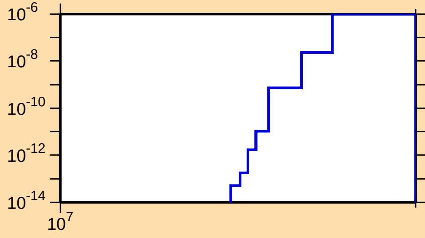
\sigma vs. E for ^{155}\text{Ho}(n,\text{nt})
