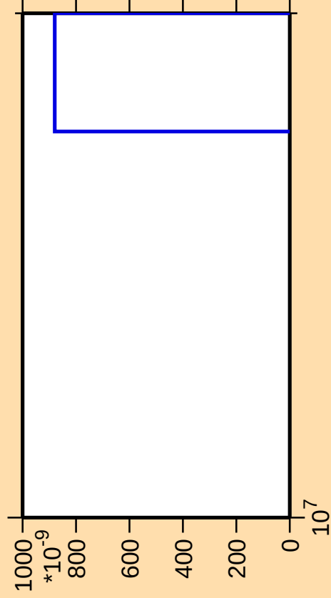
\Delta\sigma/\sigma vs. E for ^{155}\text{Ho} (mt 42)
