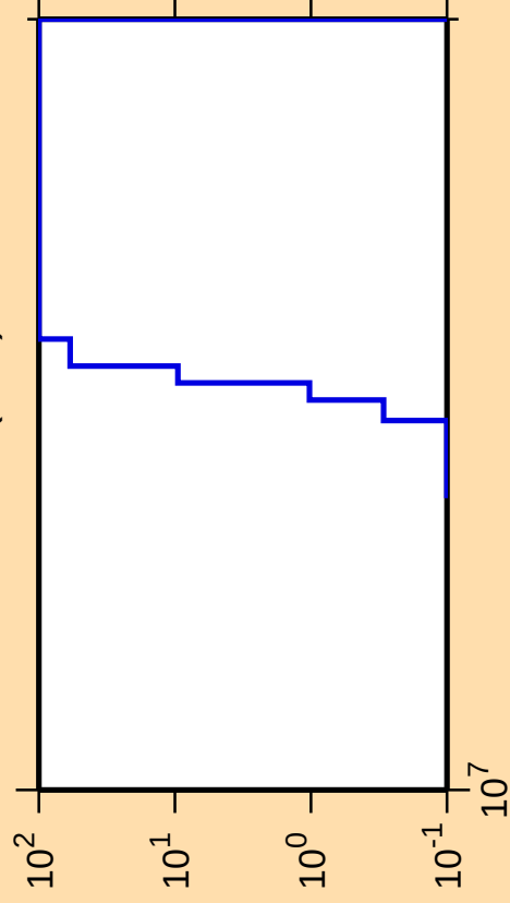
\Delta\sigma/\sigma vs. E for ^{155}\text{Ho}(n,\text{nt})
