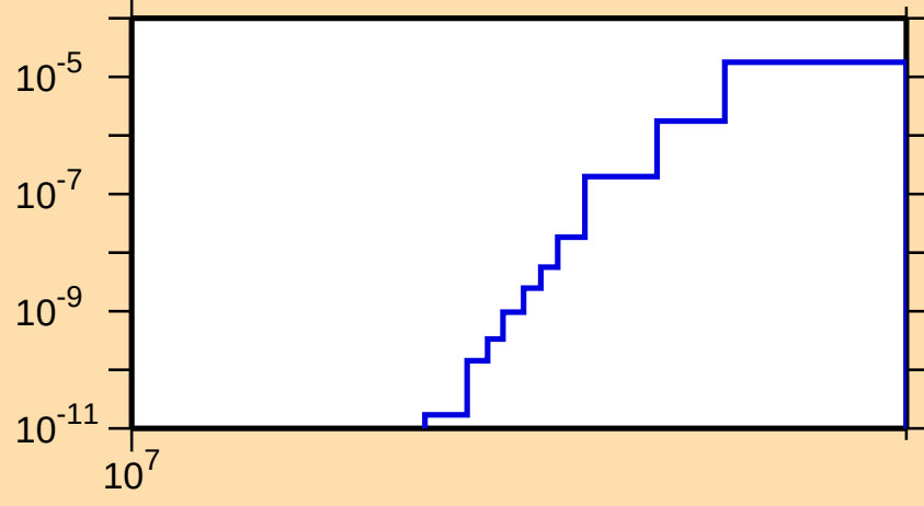
\sigma vs. E for ^{155}\text{Ho}(n,\text{nd})
