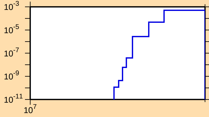
\sigma vs. E for ^{155}\text{Ho}(n,2np)
