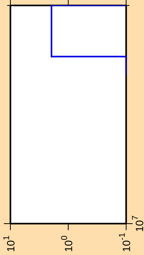
\Delta\sigma/\sigma vs. E for ^{155}\text{Ho}(n,\text{pt})
