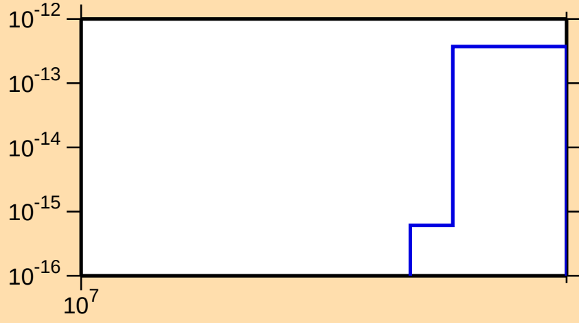
\sigma vs. E for ^{155}\text{Ho}(n,\text{pt})
