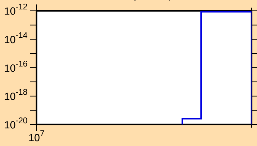
\sigma vs. E for ^{155}\text{Ho}(n,3n\alpha)
