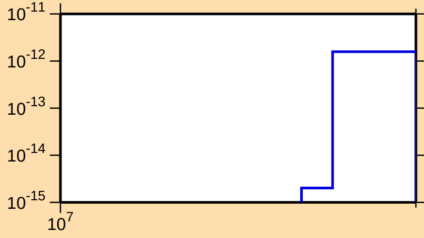
\sigma vs. E for ^{155}\text{Ho} (mt 34)
