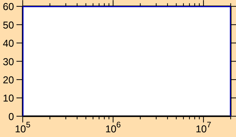
\Delta\sigma/\sigma vs. E for ^{155}\text{Ho}(n,n_1)
