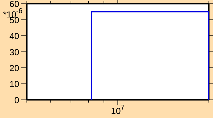
\sigma vs. E for ^{155}\text{Ho}(n,3n)
