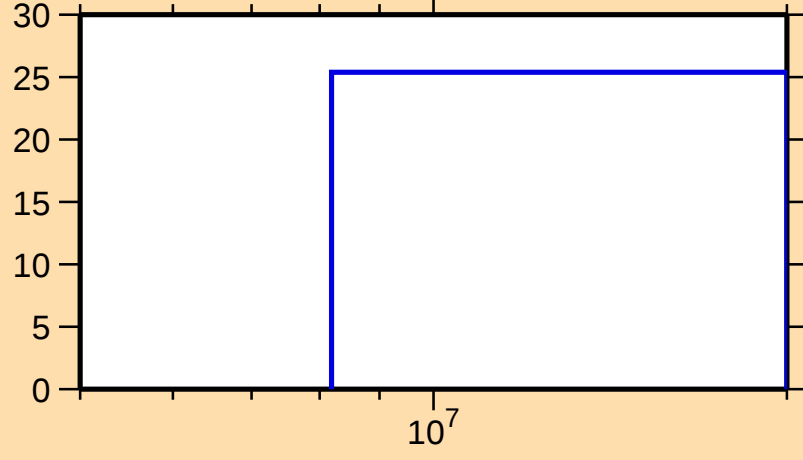
\Delta\sigma/\sigma vs. E for ^{155}\text{Ho}(n,\text{el.})
