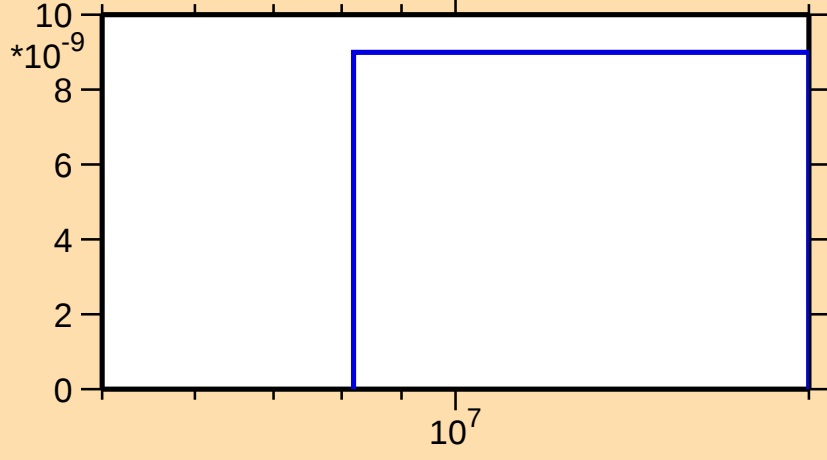
\sigma vs. E for ^{155}\text{Ho}(n,nt)
