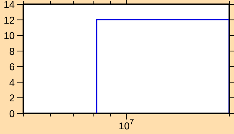
\Delta\sigma/\sigma vs. E for ^{155}\text{Ho}(n,\text{tot.})
