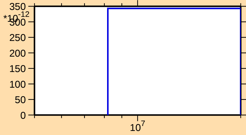
\sigma vs. E for ^{155}\text{Ho}(\text{mt117})
