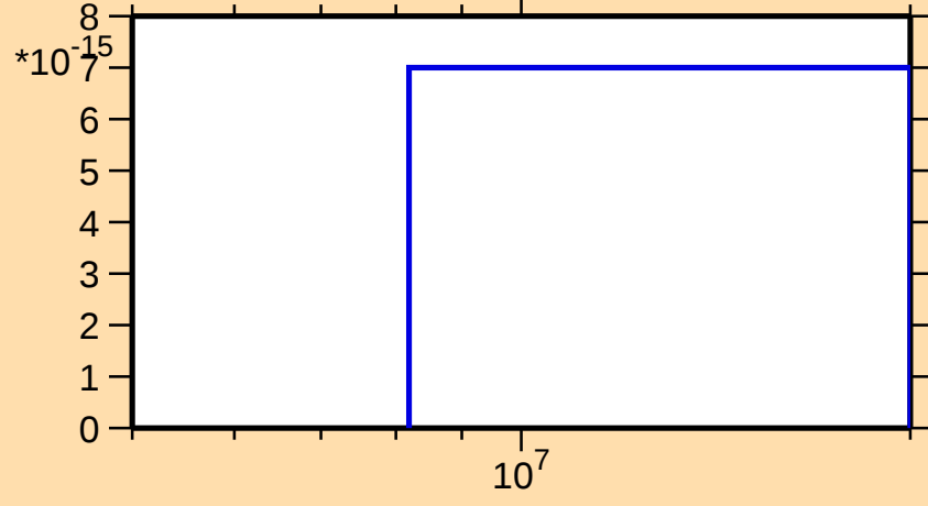
\sigma vs. E for ^{155}\text{Ho}(n,3n\alpha)
