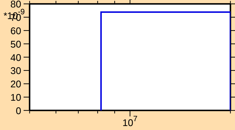
\sigma vs. E for ^{155}\text{Ho}(n,\text{He3})
