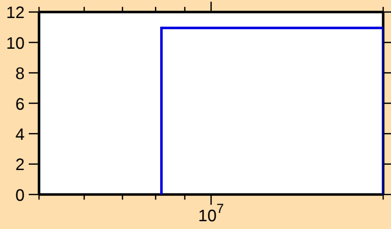
\Delta\sigma/\sigma vs. E for ^{155}\text{Ho}(n,\text{nonel.})
