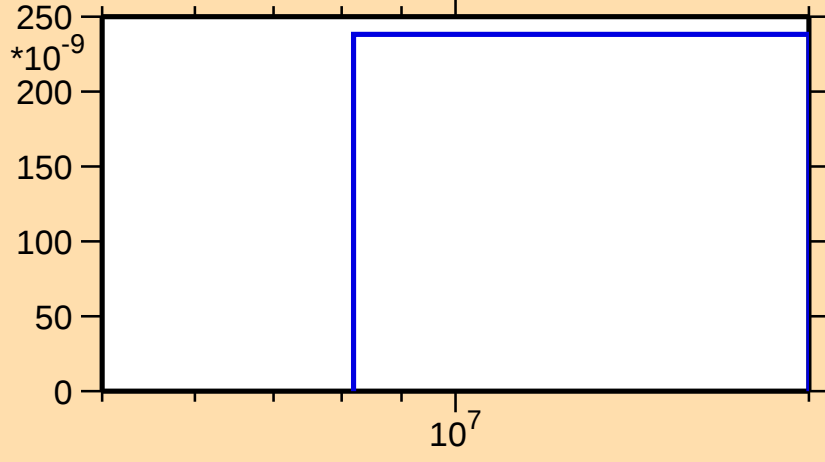
\sigma vs. E for ^{155}\text{Ho}(n,\text{nd})
