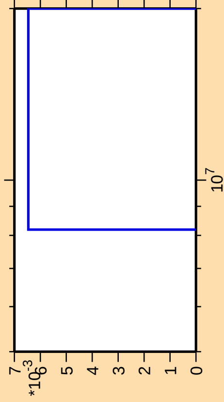
\Delta\sigma/\sigma vs. E for ^{155}\text{Ho}(n,3n\alpha)
