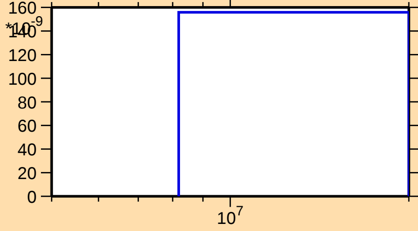
\sigma vs. E for ^{155}\text{Ho}(n,2n\alpha)
