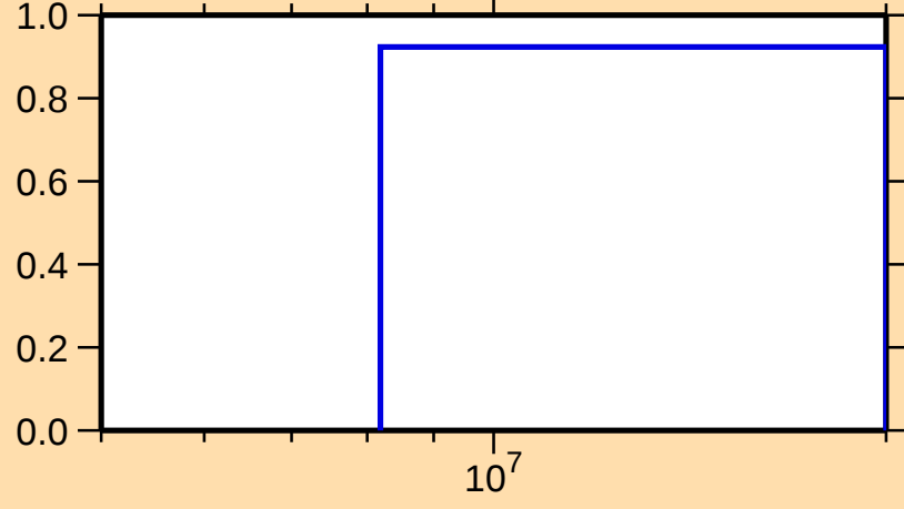
\sigma vs. E for ^{155}\text{Ho}(n,2n)
