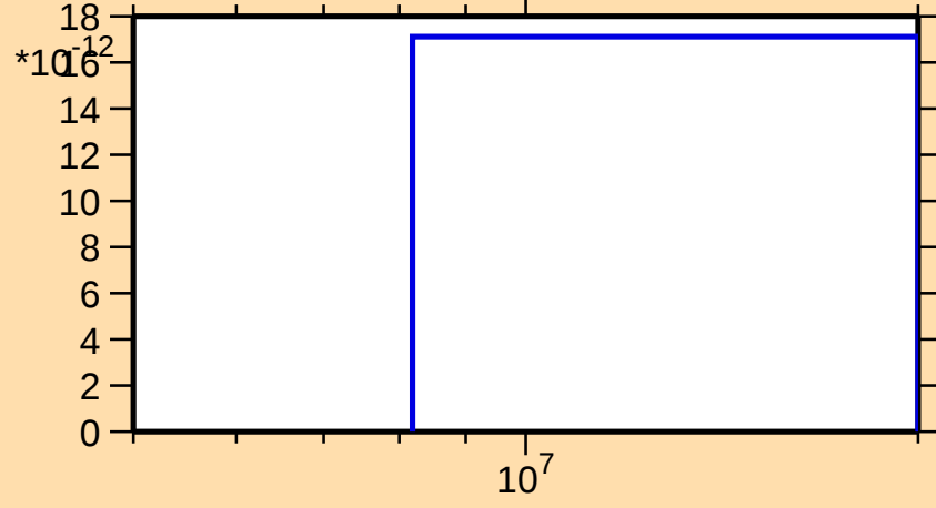
\sigma vs. E for ^{155}\text{Ho}(n,\text{pd})
