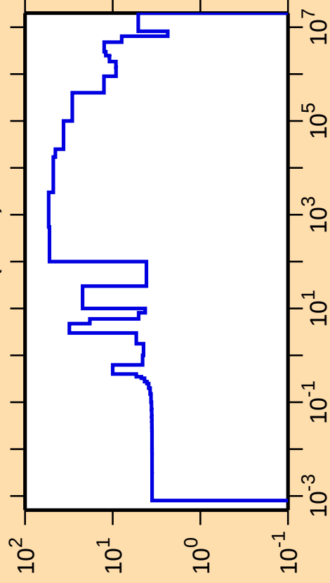
\Delta\sigma/\sigma vs. E for ^{168}\text{Ho}(n,\text{el.})
