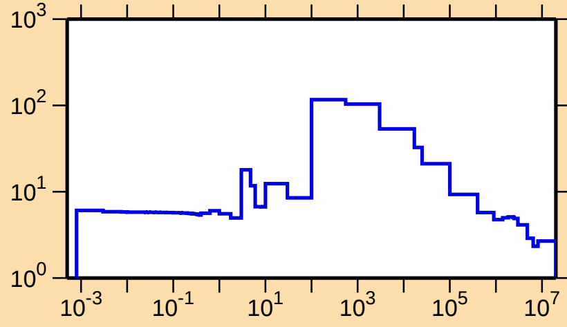
\sigma vs. E for ^{168}\text{Ho}(n,\text{el.})
