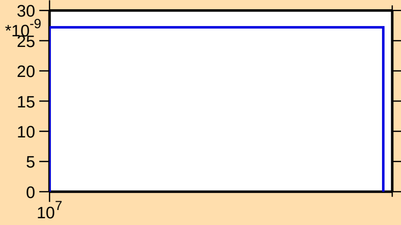
\sigma vs. E for ^{170}\text{Ho}(n,\text{nt})
