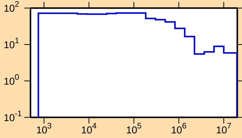
\Delta\sigma/\sigma vs. E for ^{170}\text{Ho}(\text{n,nonel.})
