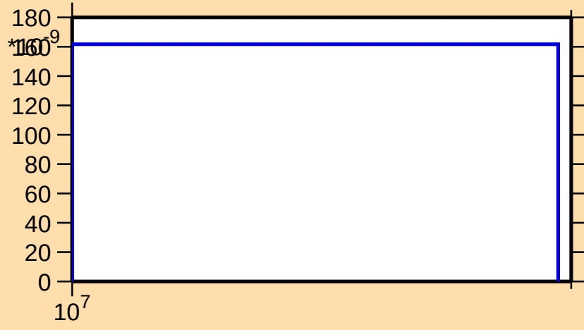
\sigma vs. E for ^{170}\text{Ho}(n,\text{nd})
