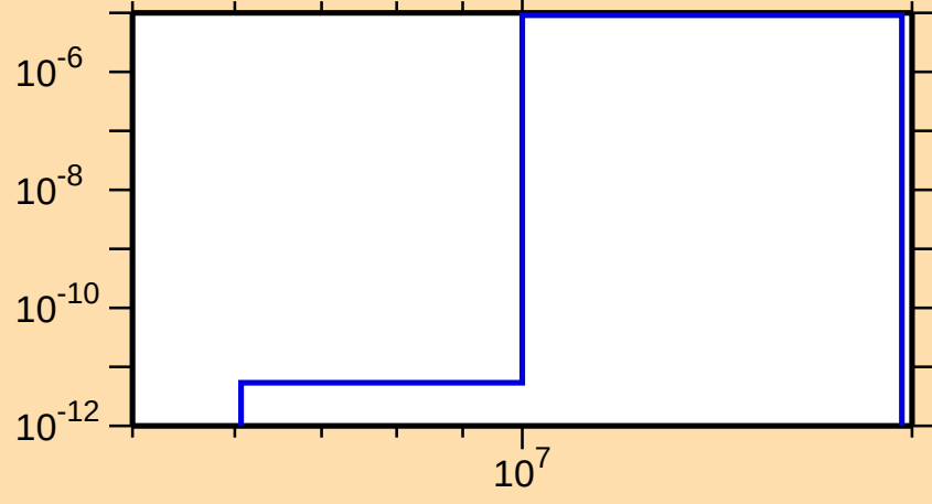
\sigma vs. E for ^{170}\text{Ho}(n,n\alpha)
