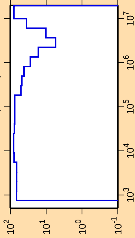
\Delta\sigma/\sigma vs. E for ^{170}\text{Ho}(\text{n,inel.})
