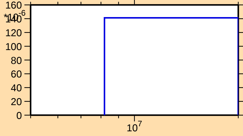
\sigma vs. E for ^{170}\text{Ho}(n,d)
