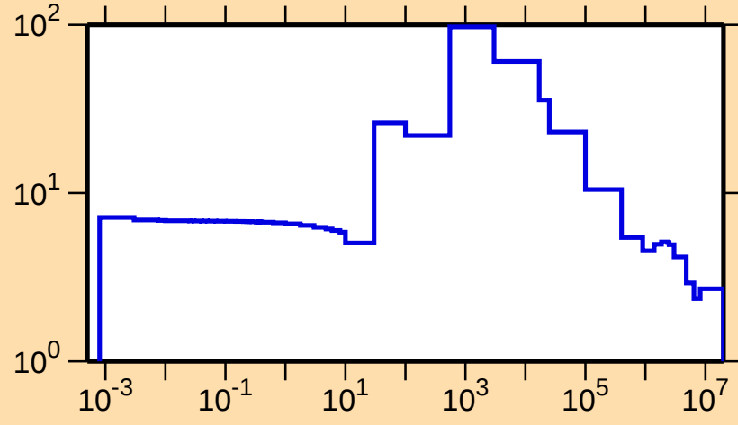
\sigma vs. E for ^{170}\text{Ho}(n,\text{el.})
