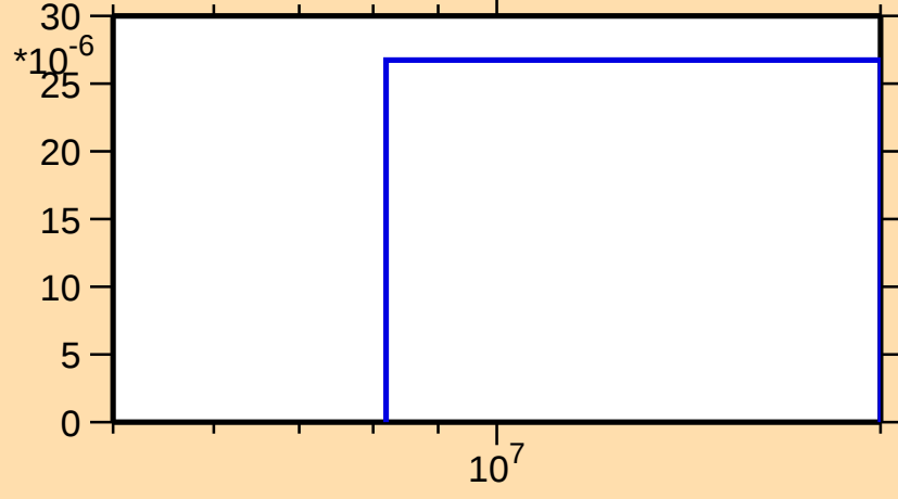
\sigma vs. E for ^{170}\text{Ho}(n,t)
