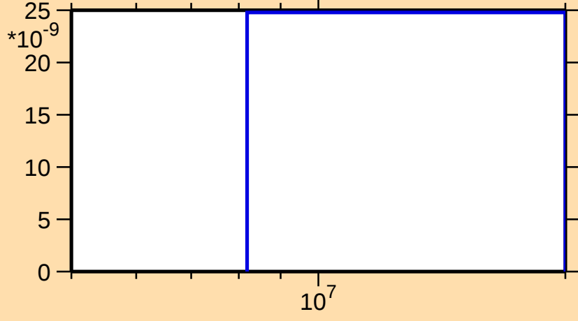
\sigma vs. E for ^{170}\text{Ho}(n,nt)
