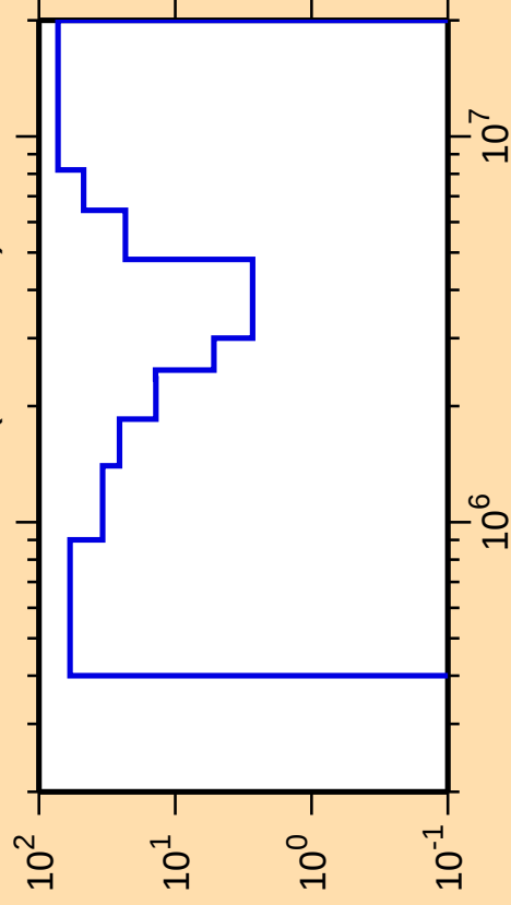
\Delta\sigma/\sigma vs. E for ^{170}\text{Ho}(\text{n},\text{ncont.})
