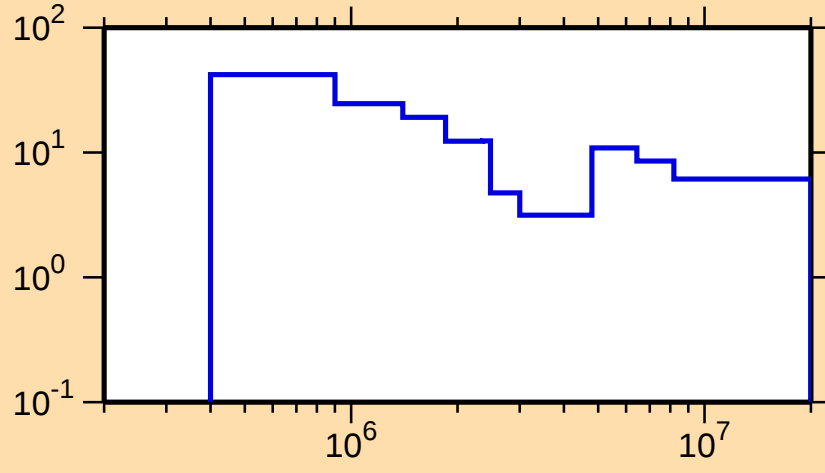
\Delta\sigma/\sigma vs. E for ^{170}\text{Ho}(\text{n},\text{nonel.})
