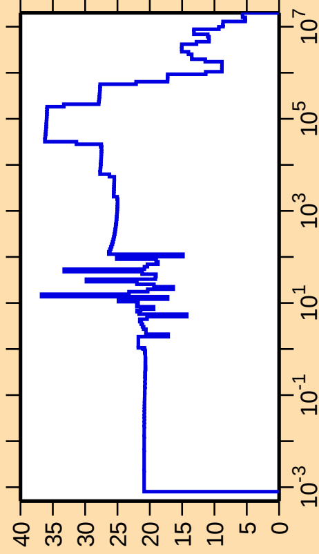
\Delta\sigma/\sigma vs. E for ^{111}\text{I}(\text{n},\text{el.})
