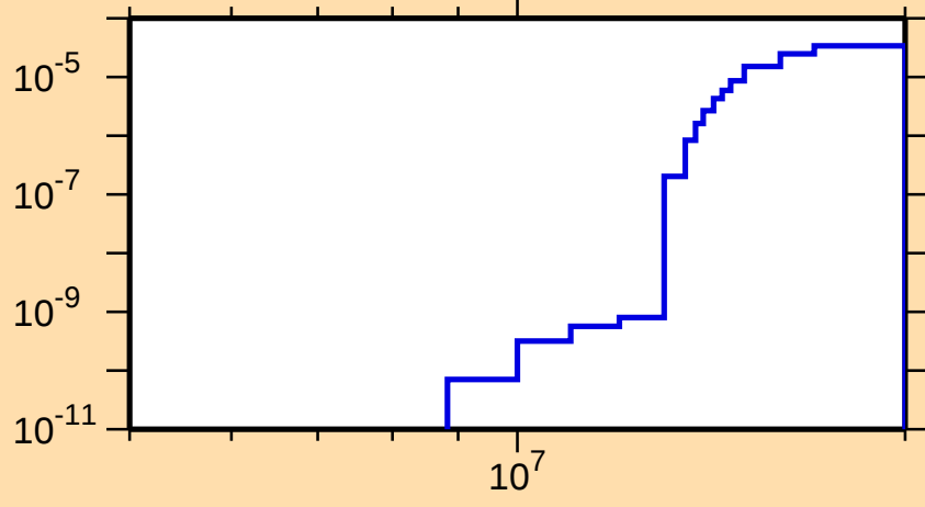
\sigma vs. E for ^{111}\text{I}(n,2n\alpha)
