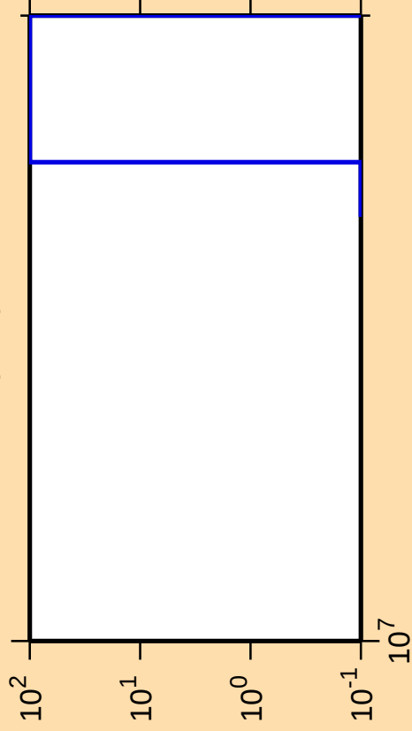
\Delta\sigma/\sigma vs. E for ^{111}\text{I}(n,\text{nt})
