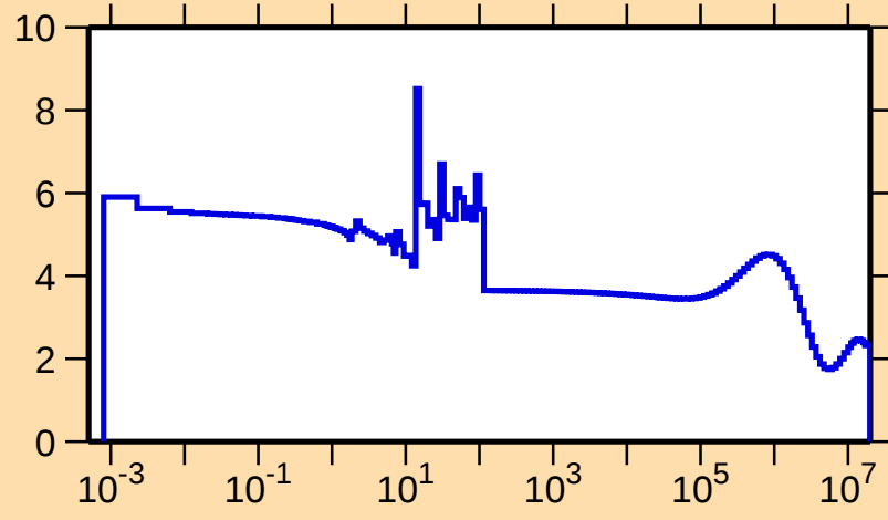
\sigma vs. E for ^{111}\text{I}(\text{n},\text{el.})
