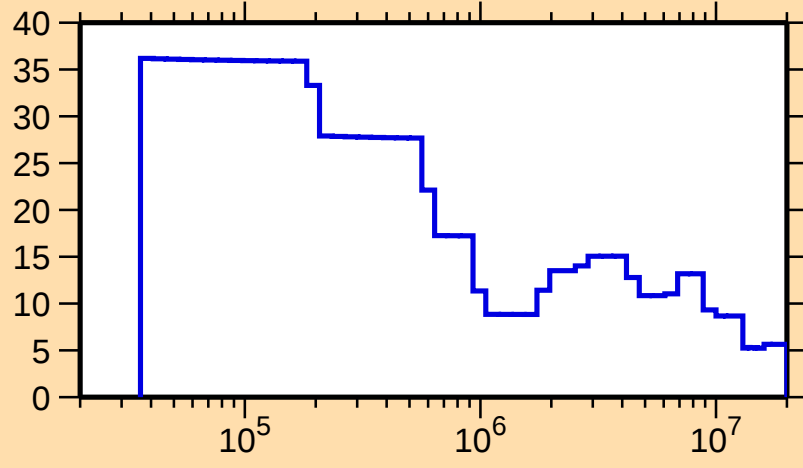
\Delta\sigma/\sigma vs. E for ^{111}\text{I}(\text{n,el.})
