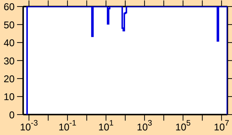
\Delta\sigma/\sigma vs. E for ^{111}\text{I}(n,\gamma)
