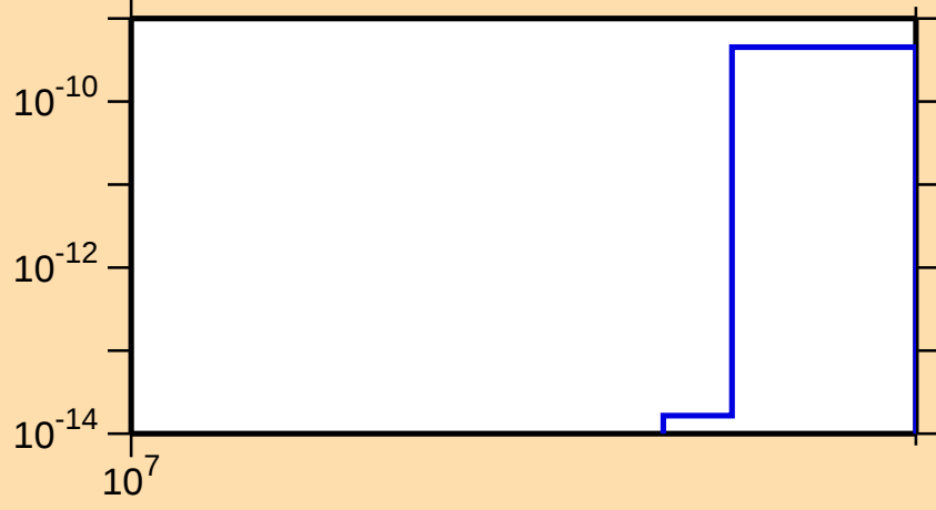
\sigma vs. E for ^{111}\text{I}(n,\text{nt})
