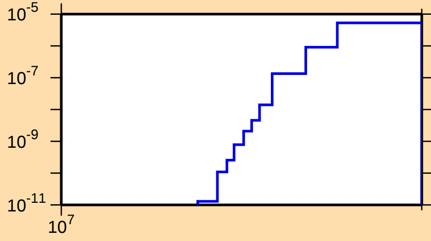
\sigma vs. E for ^{111}\text{I}(n,\text{nd})
