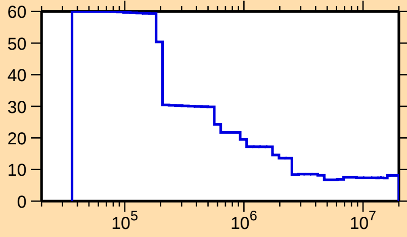
\Delta\sigma/\sigma vs. E for ^{111}\text{I}(\text{n,nonel.})
