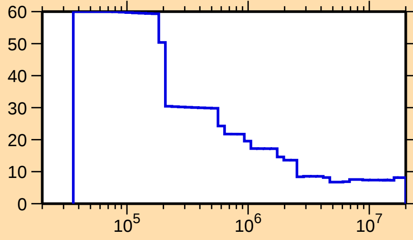
\Delta\sigma/\sigma vs. E for ^{111}\text{I}(n,\text{nonel.})
