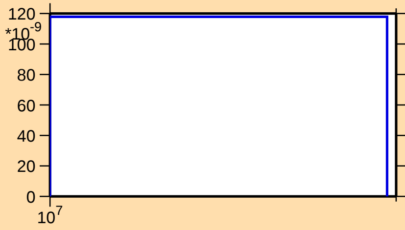
\sigma vs. E for ^{111}\text{I}(n,\text{nd})
