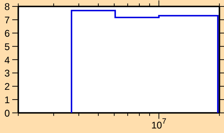
\Delta\sigma/\sigma vs. E for ^{111}\text{I}(n, \text{nonel.})
