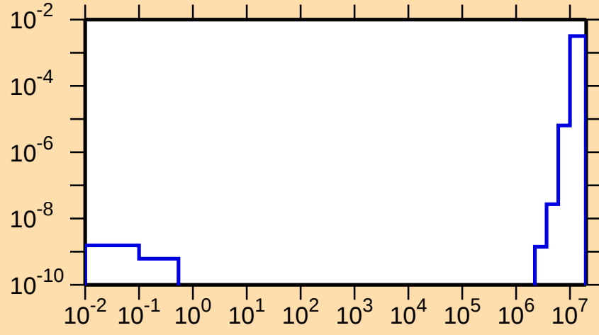
\sigma vs. E for ^{111}\text{I}(n,\text{He3})
