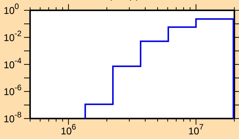
\sigma vs. E for ^{111}\text{I}(n,np)
