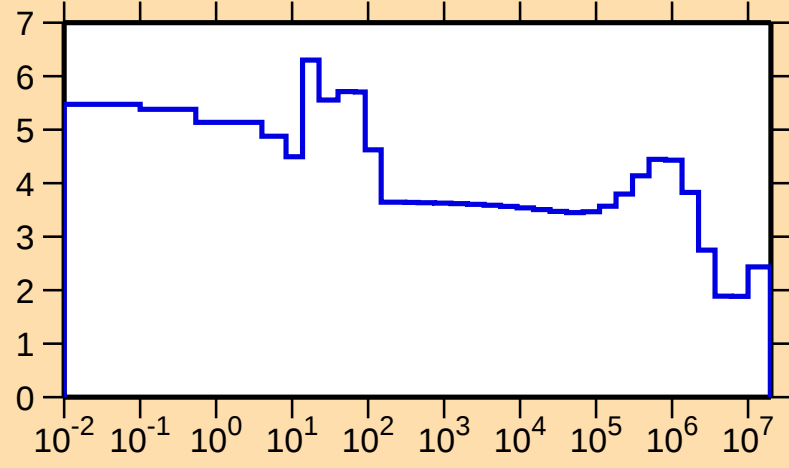
\sigma vs. E for ^{111}\text{I}(n,\text{el.})
