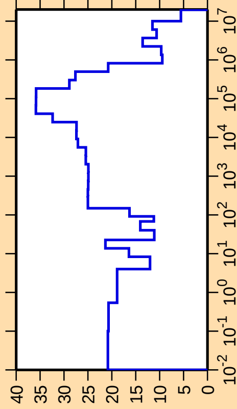
\Delta\sigma/\sigma vs. E for ^{111}\text{I}(n,\text{el.})
