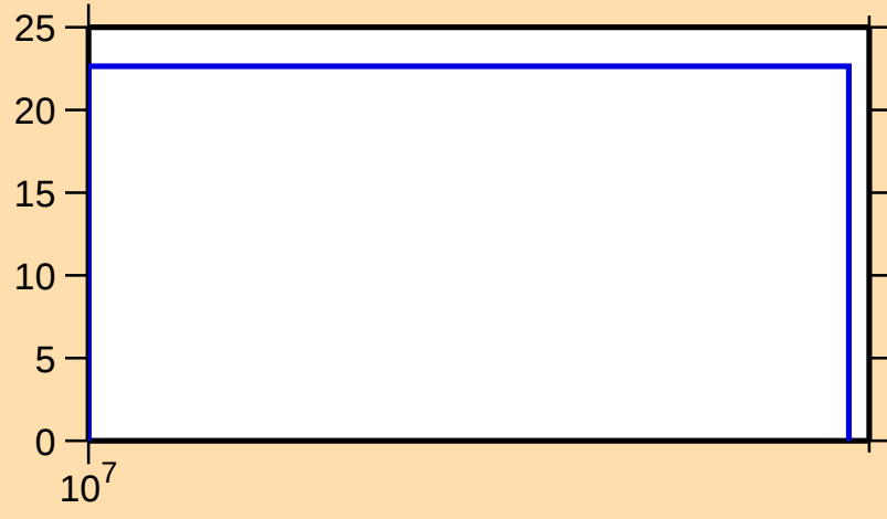
\Delta\sigma/\sigma vs. E for ^{111}\text{I}(n,\text{inel.})
