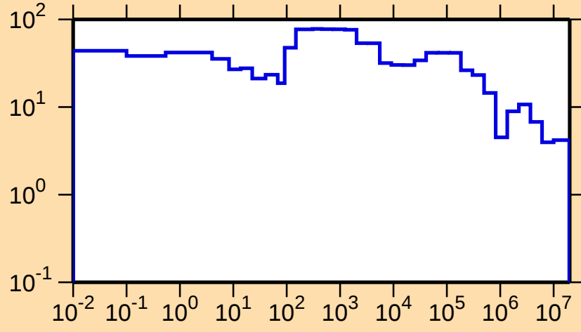
\Delta\sigma/\sigma vs. E for ^{111}\text{I}(\text{n,tot.})
