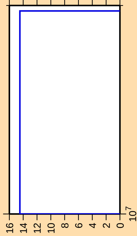
\Delta\sigma/\sigma vs. E for ^{111}\text{I}(n,nt)
