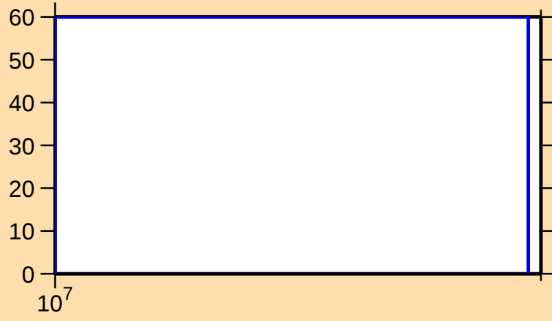
\Delta\sigma/\sigma vs. E for ^{111}\text{I}(\text{n},2\text{n})
