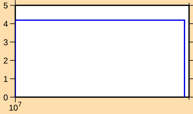
\Delta\sigma/\sigma vs. E for ^{111}\text{I}(n,\text{tot.})
