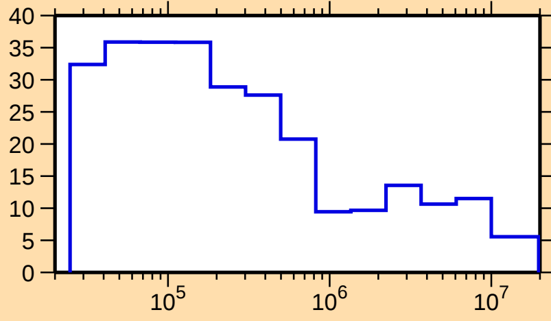
\Delta\sigma/\sigma vs. E for ^{111}\text{I}(n,\text{el.})
