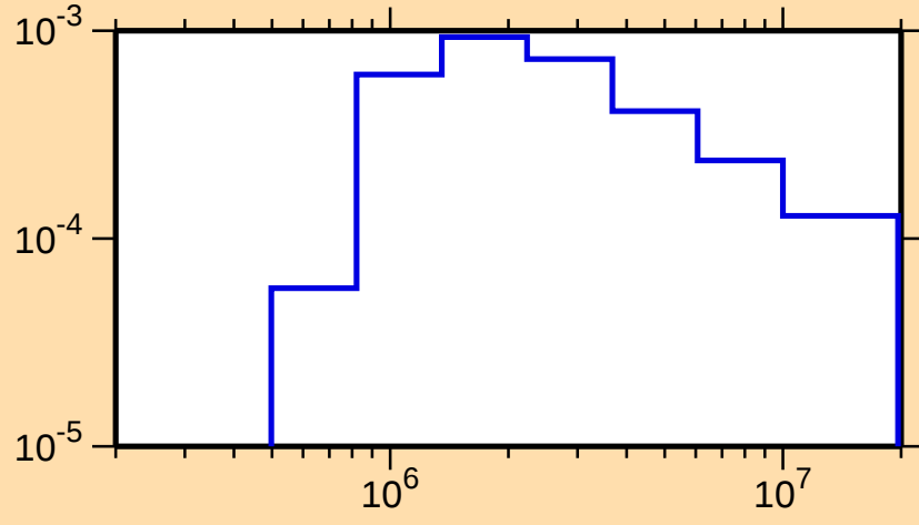
\sigma vs. E for ^{111}\text{I}(n,n_3)
