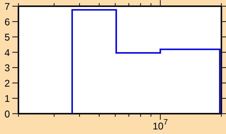
\Delta\sigma/\sigma vs. E for ^{111}\text{I}(\text{n},\text{tot.})
