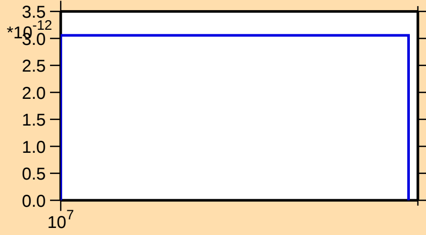
\sigma vs. E for ^{111}\text{I}(n,nt)
