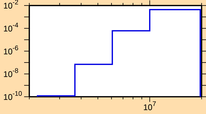
\sigma vs. E for ^{111}\text{I}(n,n\alpha)
