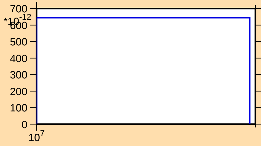
\sigma vs. E for ^{111}\text{I}(\text{mt } 34)
