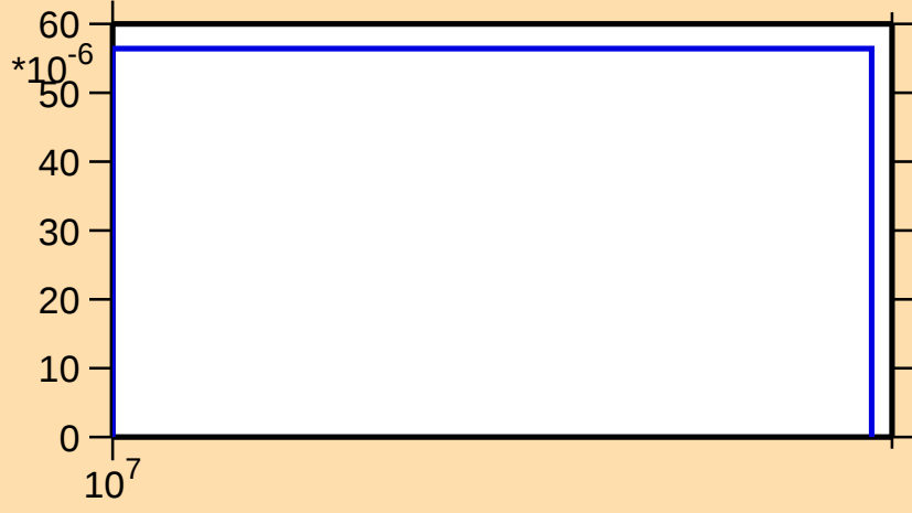
\sigma vs. E for ^{111}\text{I}(n,2n)
