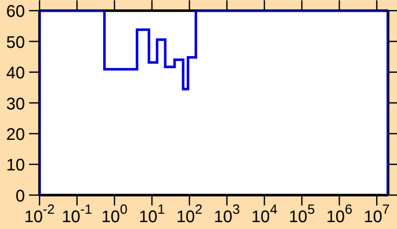
\Delta\sigma/\sigma vs. E for ^{111}\text{I}(n,\gamma)
