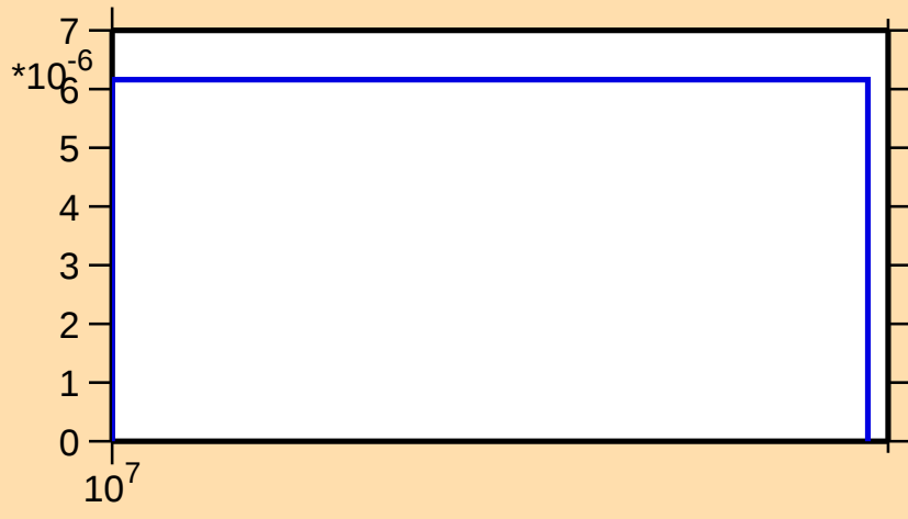
\sigma vs. E for ^{111}\text{I}(n,2np)
