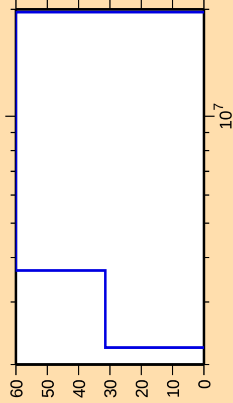
\Delta\sigma/\sigma vs. E for ^{111}\text{I}(n,n\alpha)
