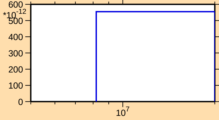
\sigma vs. E for ^{111}\text{I}(\text{mt } 34)
