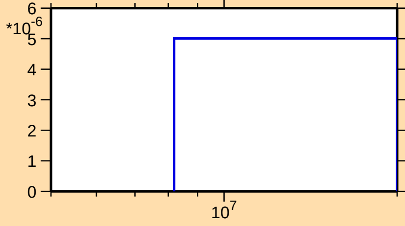
\sigma vs. E for ^{111}\text{I}(n,2np)
