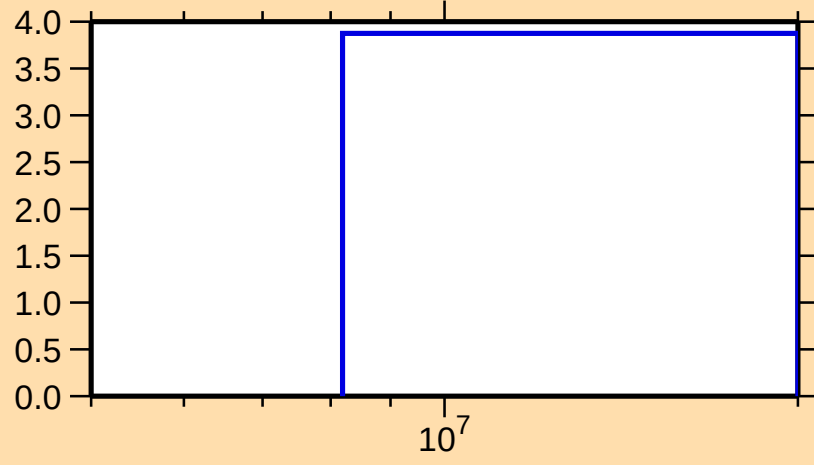
\Delta\sigma/\sigma vs. E for ^{111}\text{I}(n,\text{tot.})
