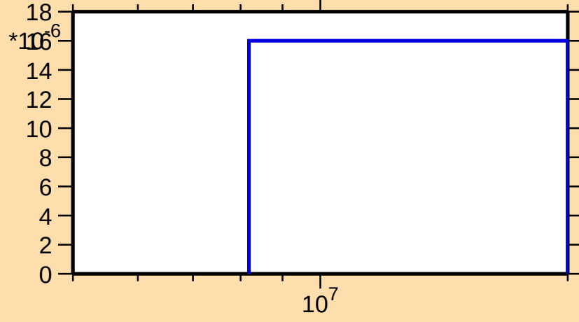
\sigma vs. E for ^{111}\text{I}(n,\text{pt})
