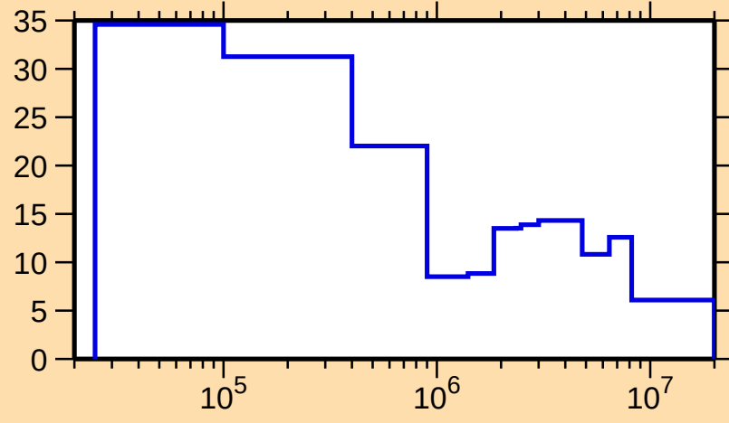
\Delta\sigma/\sigma vs. E for ^{111}\text{I}(\text{n,el.})
