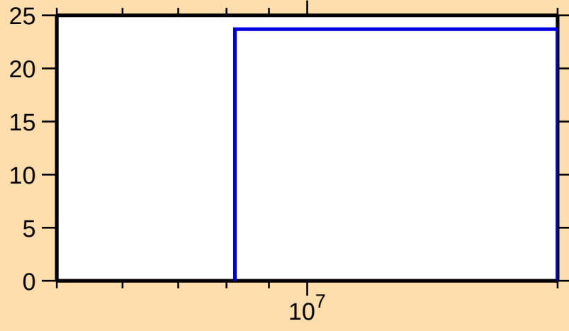
\Delta\sigma/\sigma vs. E for ^{111}\text{I}(n,\text{inel.})
