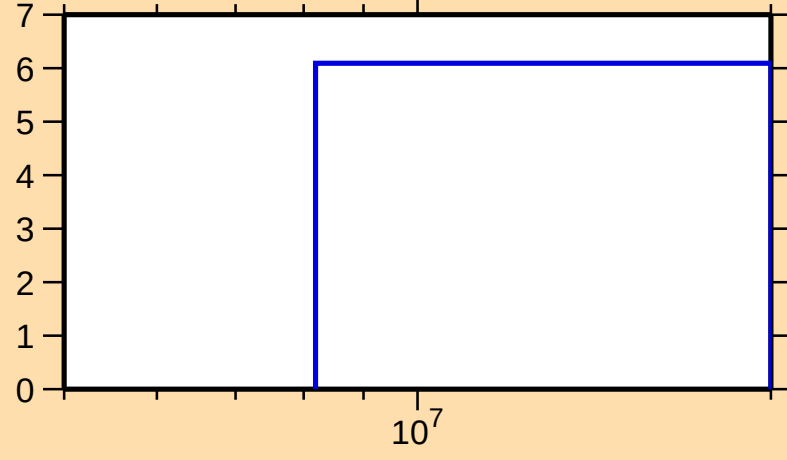
\Delta\sigma/\sigma vs. E for ^{111}\text{I}(n,\text{el.})
