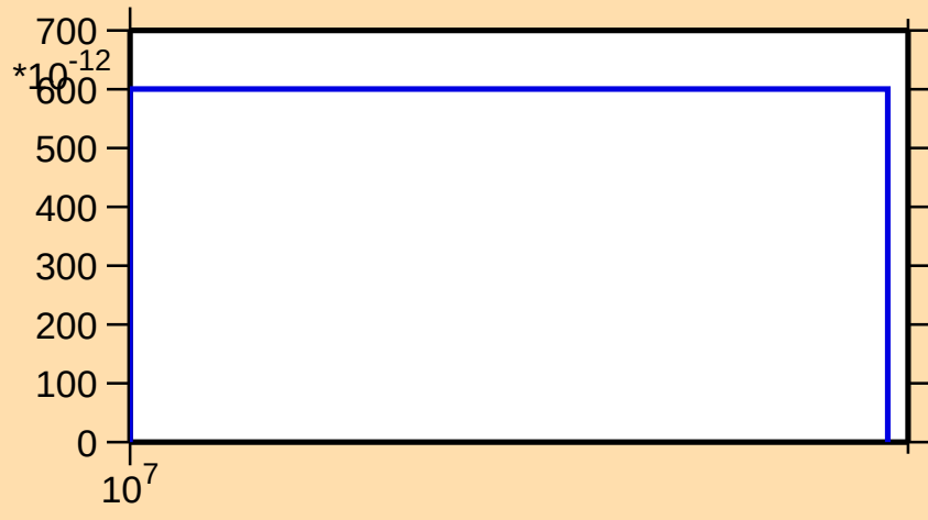
\sigma vs. E for ^{120}\text{I}(n,\text{pt})
