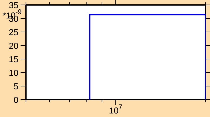
\sigma vs. E for ^{120}\text{I}(\text{mt 45})
