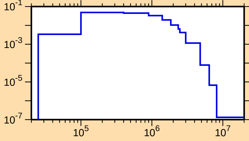
\sigma vs. E for ^{120}\text{I}(n,n_2)
