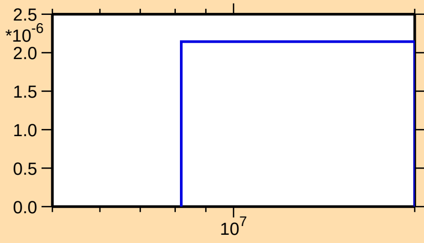
\sigma vs. E for ^{120}\text{I}(n,2n\alpha)
