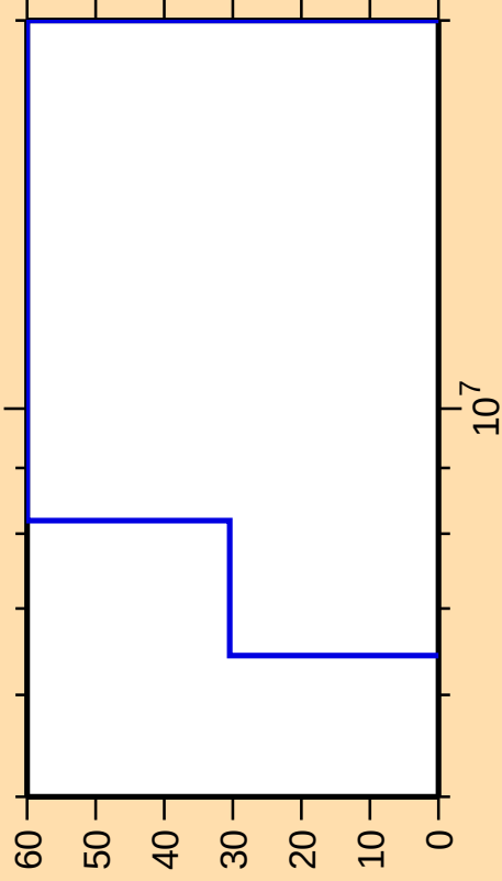
\Delta\sigma/\sigma vs. E for ^{120}\text{I}(n,p)
