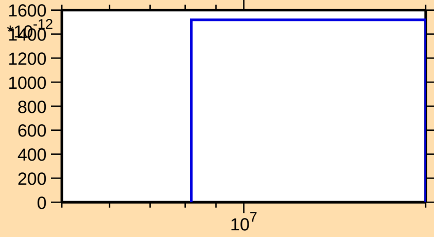
\sigma vs. E for ^{120}\text{I}(\text{n},\text{pd})
