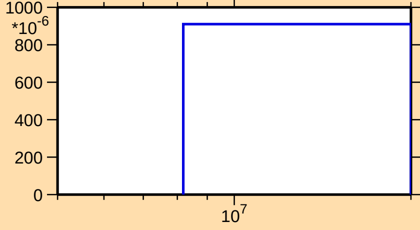
\sigma vs. E for ^{120}\text{I}(n,2np)
