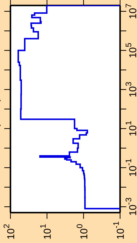
\Delta\sigma/\sigma vs. E for ^{120}\text{I}(n,\text{el.})
