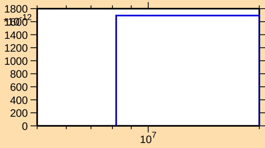
\sigma vs. E for ^{120}\text{I}(\text{mt117})
