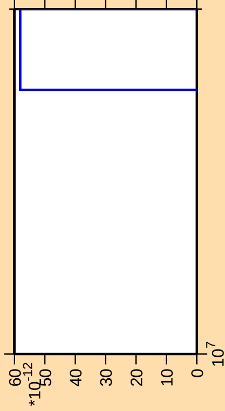
\Delta\sigma/\sigma vs. E for ^{121}\text{I} (mt 11)
