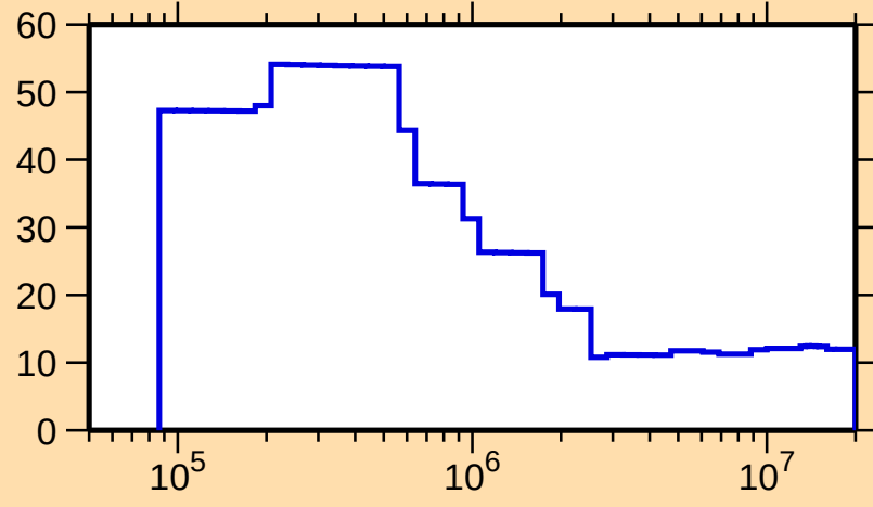
\Delta\sigma/\sigma vs. E for ^{121}\text{I}(n,\text{nonel.})
