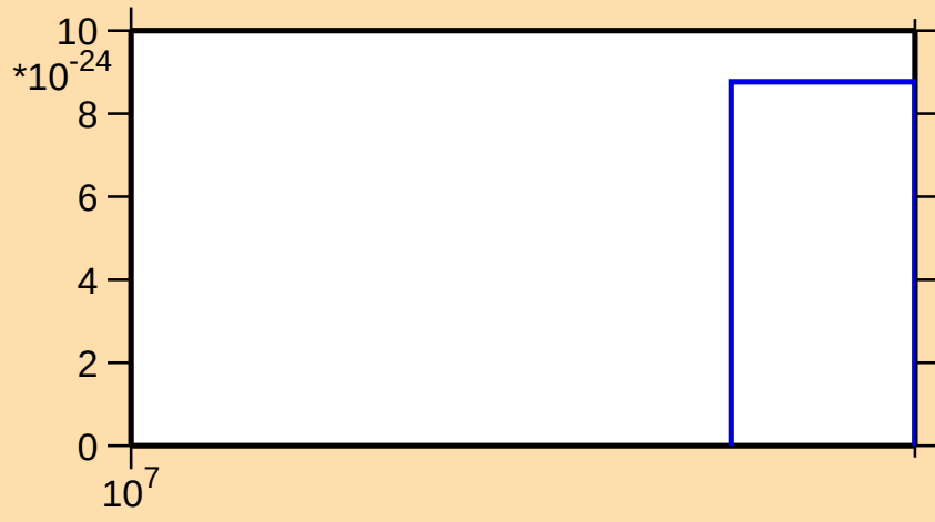
\sigma vs. E for ^{121}\text{I} (mt 11)
