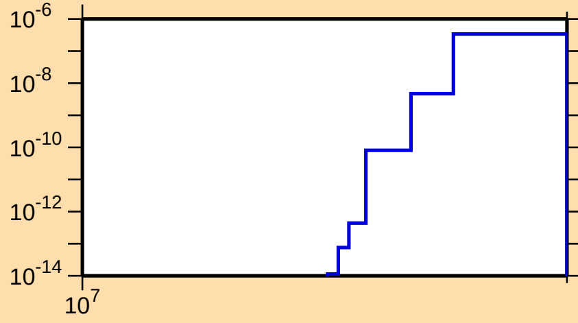
\sigma vs. E for ^{121}\text{I}(n,2n\alpha)
