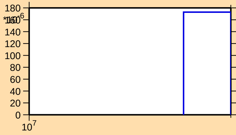
\sigma vs. E for ^{121}\text{I}(n,3n)
