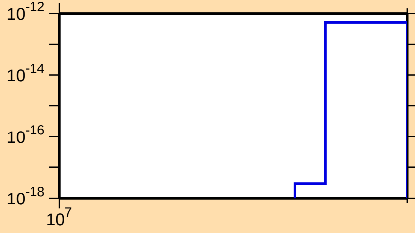
\sigma vs. E for ^{121}\text{I}(\text{n},\text{pt})
