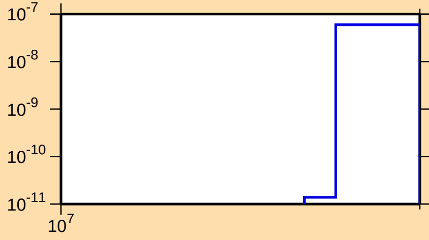
\sigma vs. E for ^{121}\text{I}(\text{n},\text{nt})
