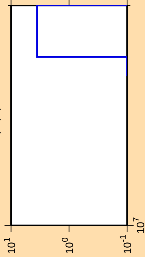
\Delta\sigma/\sigma vs. E for ^{121}\text{I}(\text{n},\text{pt})
