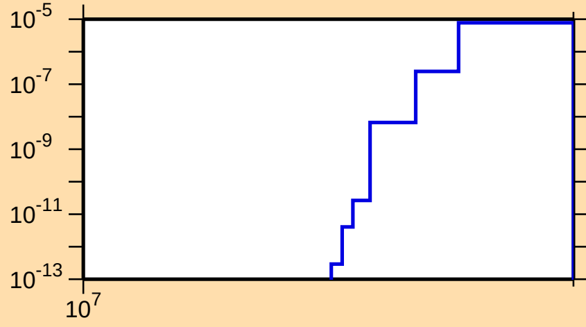
\sigma vs. E for ^{121}\text{I}(\text{n},\text{nd})
