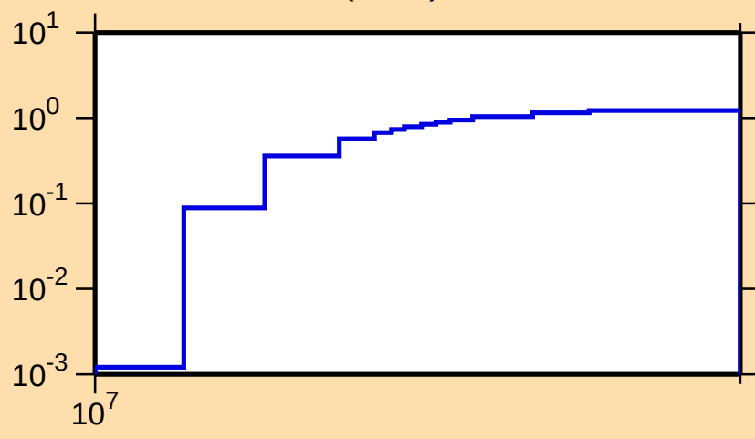
\sigma vs. E for ^{121}\text{I}(n,2n)
