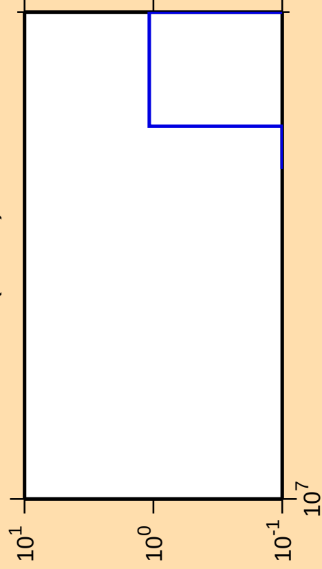
\Delta\sigma/\sigma vs. E for ^{121}\text{I} (mt 34)
