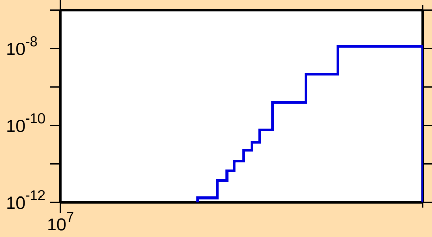
\sigma vs. E for ^{121}\text{I}(\text{mt117})
