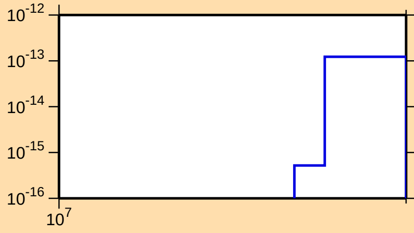
\sigma vs. E for ^{121}\text{I} (mt 34)
