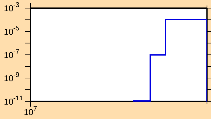
\sigma vs. E for ^{121}\text{I}(n,2np)
