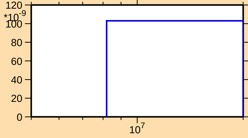
\sigma vs. E for ^{121}\text{I}(n,\text{He3})
