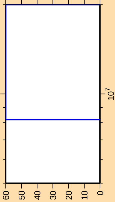
\Delta\sigma/\sigma vs. E for ^{121}\text{I}(n,t)
