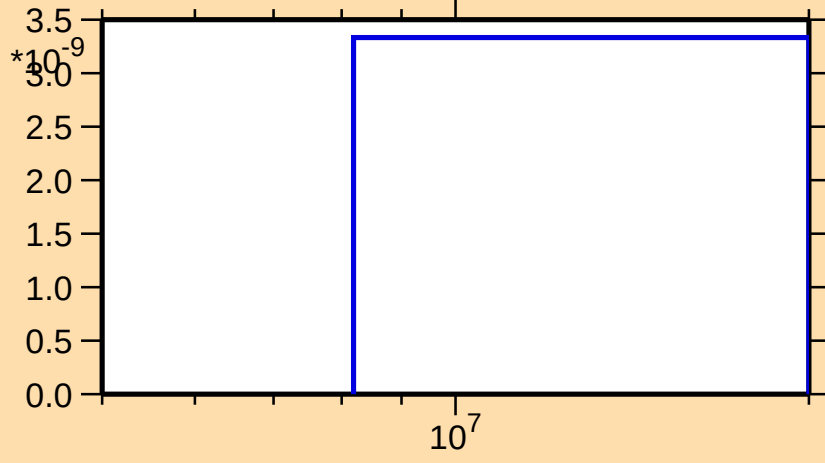
\sigma vs. E for ^{121}\text{I} (mt 45)
