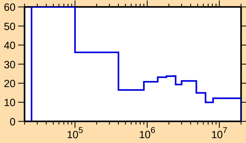
\Delta\sigma/\sigma vs. E for ^{121}\text{I}(\text{n,el.})
