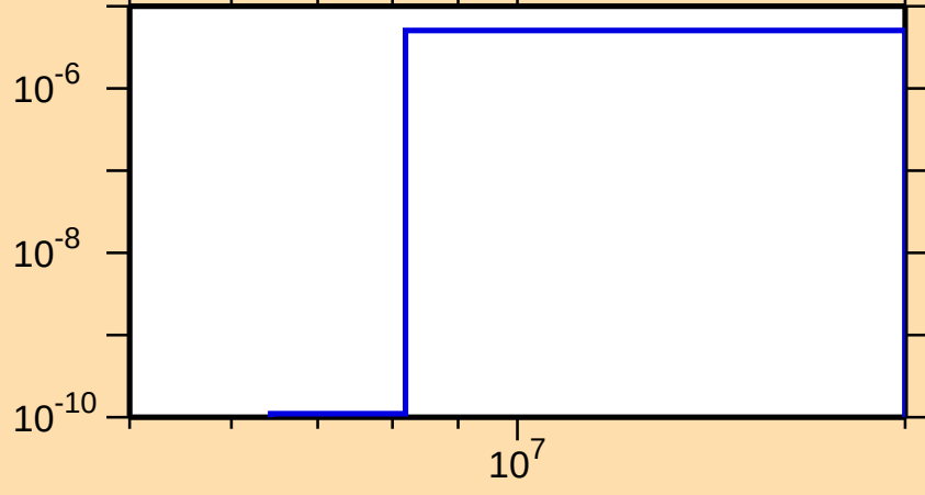
\sigma vs. E for ^{121}\text{I}(n,p\alpha)
