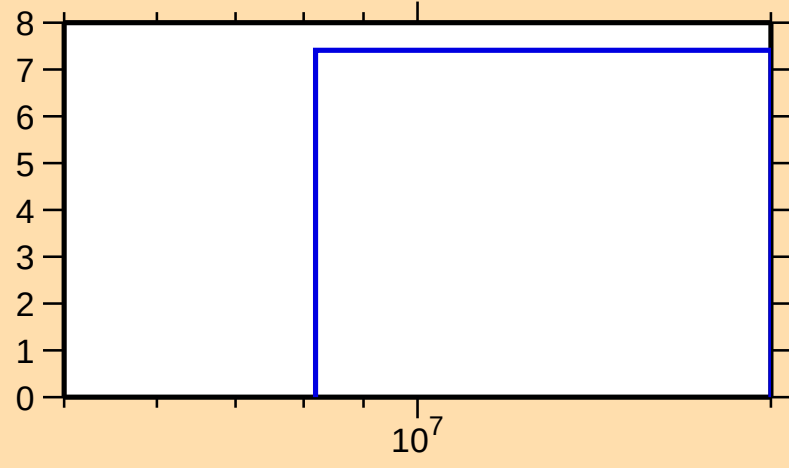
\Delta\sigma/\sigma vs. E for ^{121}\text{I}(n,\text{tot.})
