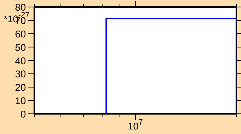
\sigma vs. E for ^{121}\text{I}(\text{mt 11})
