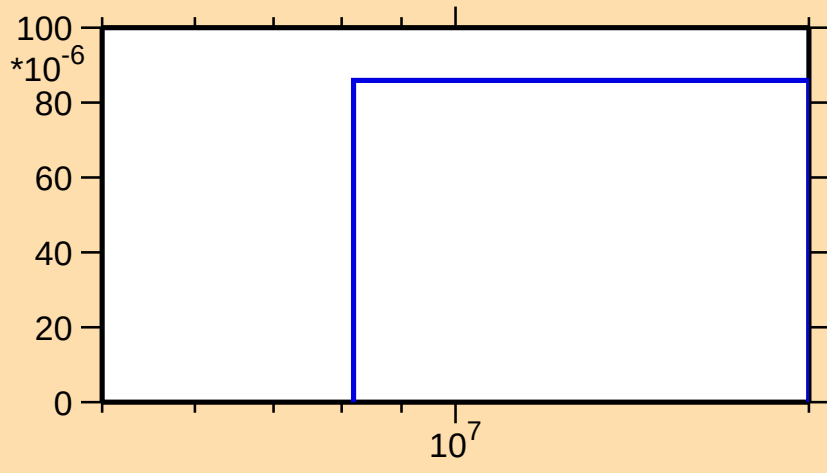
\sigma vs. E for ^{121}\text{I}(n,t)
