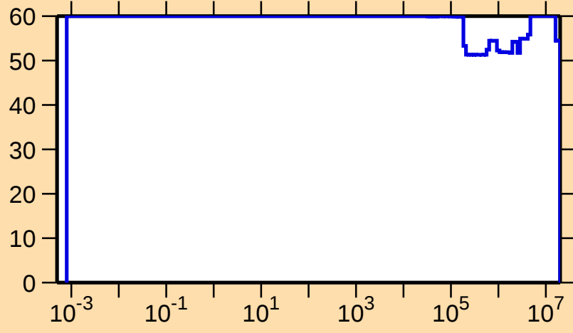
\Delta\sigma/\sigma vs. E for ^{124}\text{I}(n,p)
