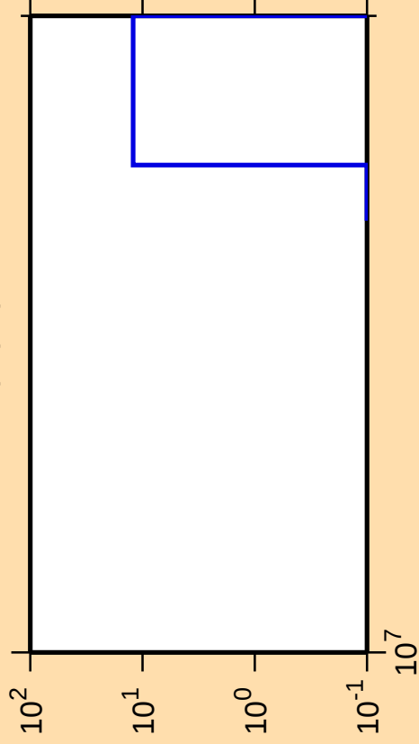
\Delta\sigma/\sigma vs. E for ^{124}\text{I}(\text{n},\text{pd})
