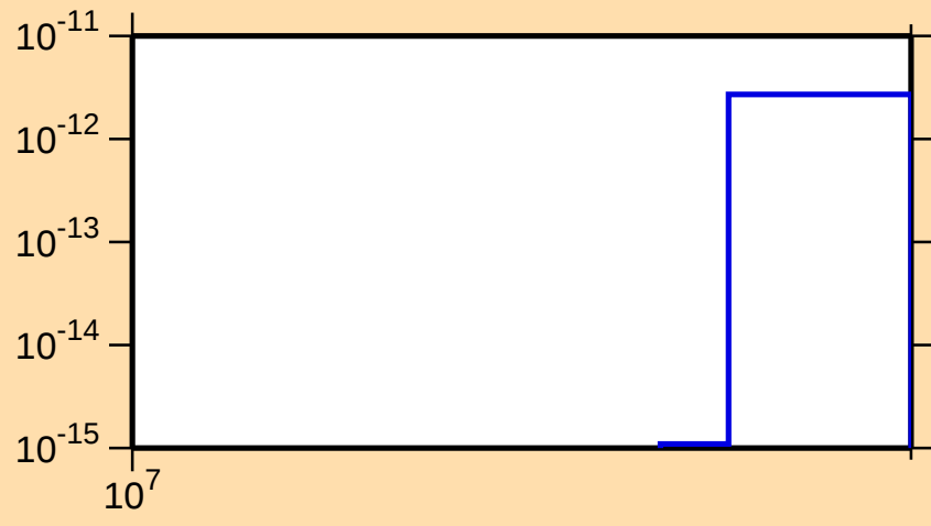
\sigma vs. E for ^{124}\text{I}(\text{n},\text{pd})
