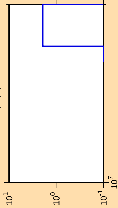
\Delta\sigma/\sigma vs. E for ^{124}\text{I}(n,\text{pt})
