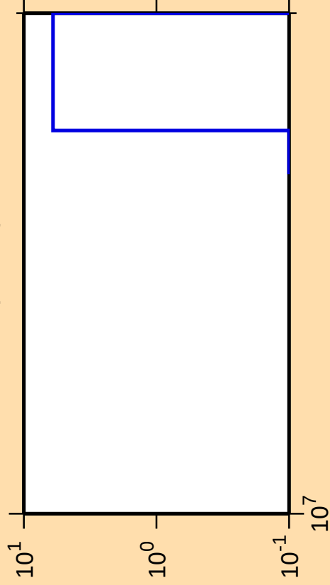
\Delta\sigma/\sigma vs. E for ^{124}\text{I} (mt 34)
