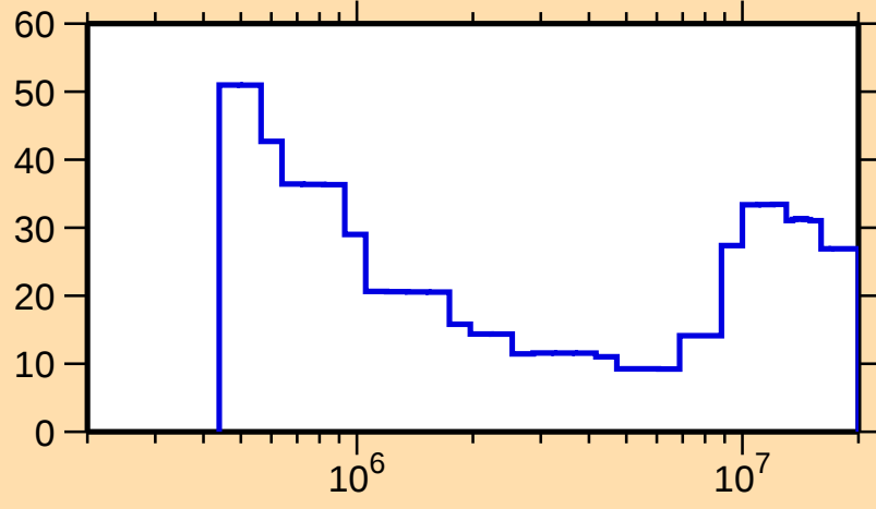
\Delta\sigma/\sigma vs. E for ^{124}\text{I}(\text{n},\text{inel.})
