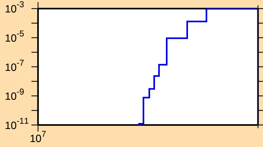
\sigma vs. E for ^{124}\text{I}(n,2np)
