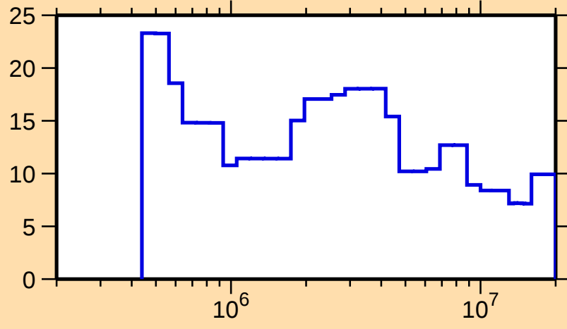
\Delta\sigma/\sigma vs. E for ^{124}\text{I}(\text{n},\text{el.})
