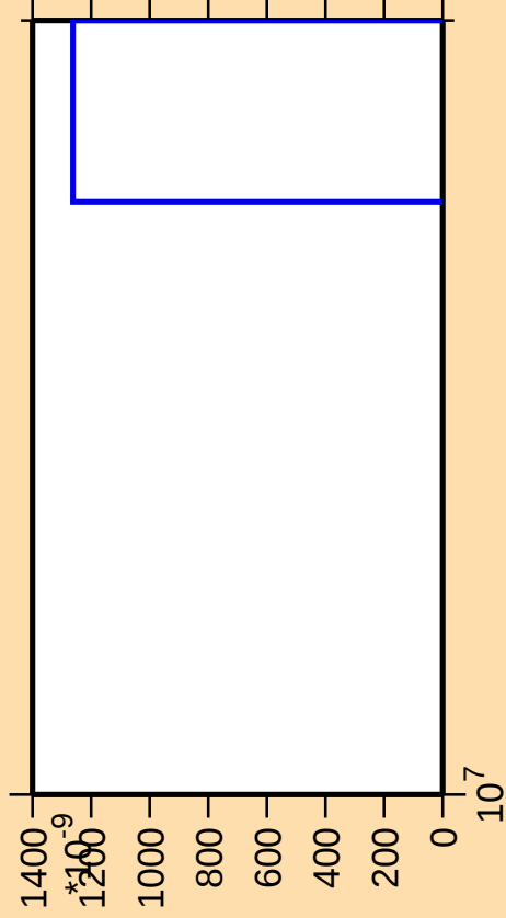
\Delta\sigma/\sigma vs. E for ^{124}\text{I}(n,3n\alpha)
