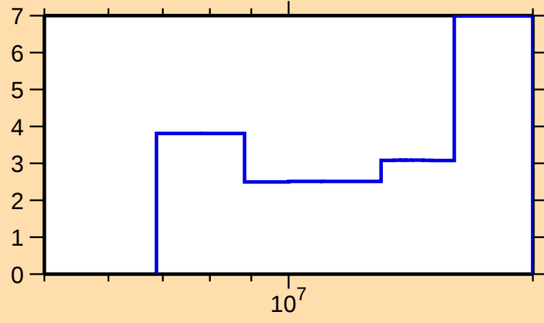
\Delta\sigma/\sigma vs. E for ^{124}\text{I}(n,\text{tot.})
