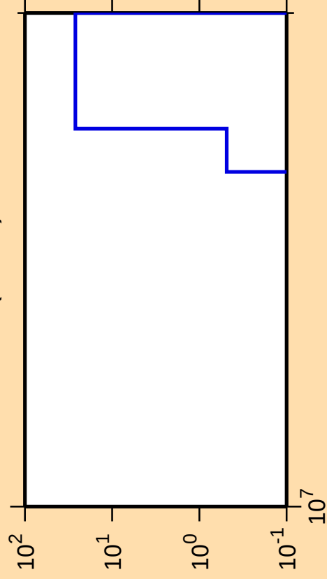
\Delta\sigma/\sigma vs. E for ^{124}\text{I}(\text{mt 45})
