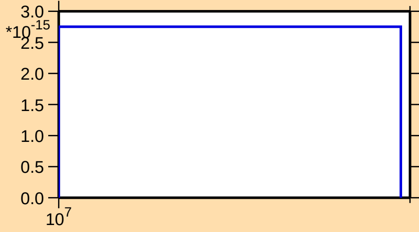
\sigma vs. E for ^{124}\text{I}(\text{n},\text{pt})
