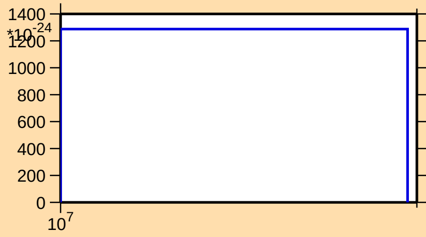
\sigma vs. E for ^{124}\text{I}(n,3n\alpha)
