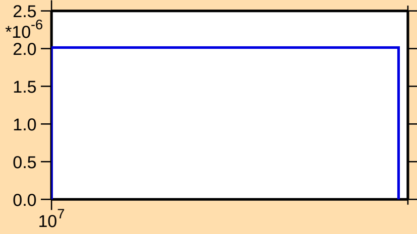
\sigma vs. E for ^{124}\text{I}(\text{n},\text{nd})
