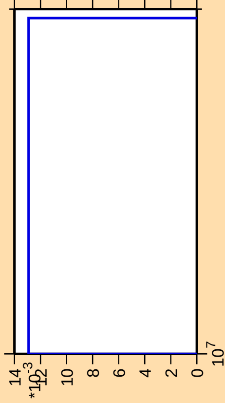
\Delta\sigma/\sigma vs. E for ^{124}\text{I}(\text{n},\text{pt})
