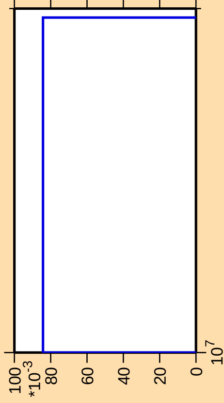
\Delta\sigma/\sigma vs. E for ^{124}\text{I}(\text{n},\text{pd})
