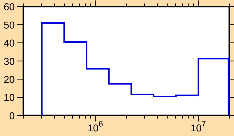
\Delta\sigma/\sigma vs. E for ^{124}\text{I}(\text{n},\text{inel.})
