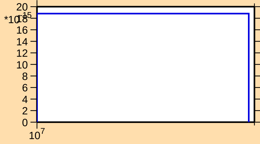
\sigma vs. E for ^{124}\text{I}(\text{n},\text{pd})
