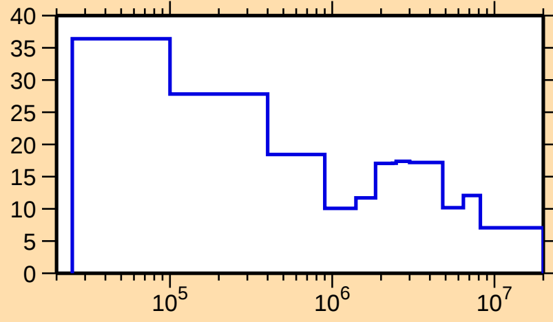
\Delta\sigma/\sigma vs. E for ^{124}\text{I}(\text{n,el.})
