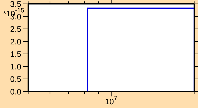
\sigma vs. E for ^{124}\text{I}(n,\text{pt})
