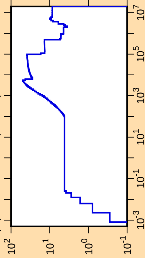
\Delta\mu/\mu vs. E for ^{127}\text{I}(\text{mt251})
