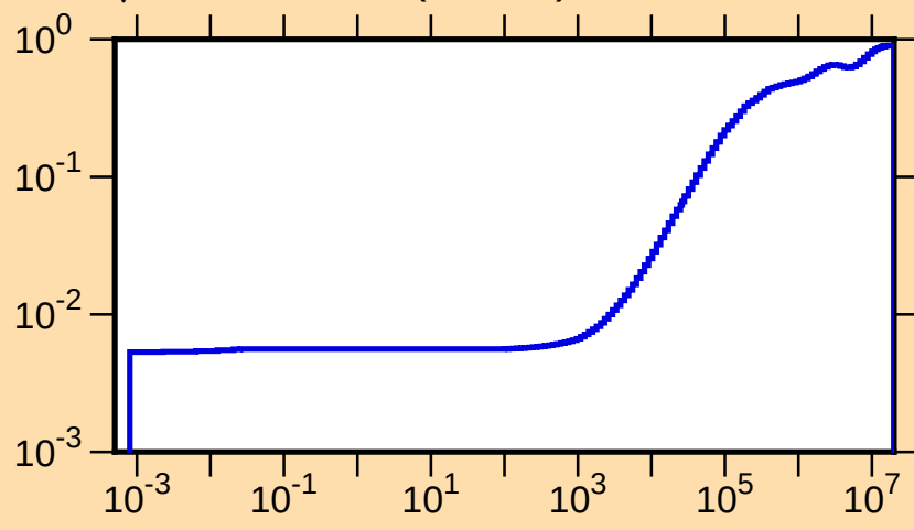
\mu vs. E for ^{127}\text{I}(\text{mt251})
