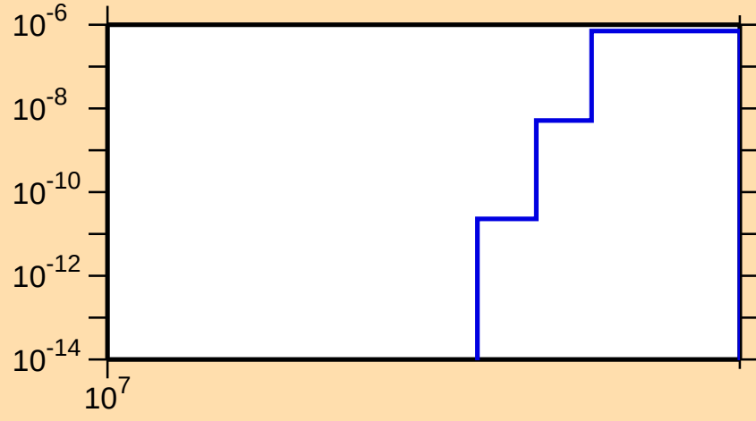
\sigma vs. E for ^{127}\text{I}(\text{n},\text{nd})
