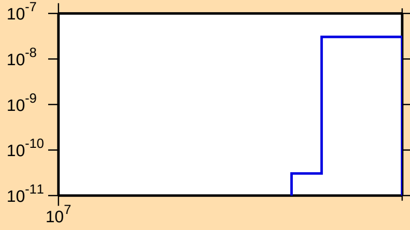
\sigma vs. E for ^{127}\text{I}(\text{n},\text{nt})
