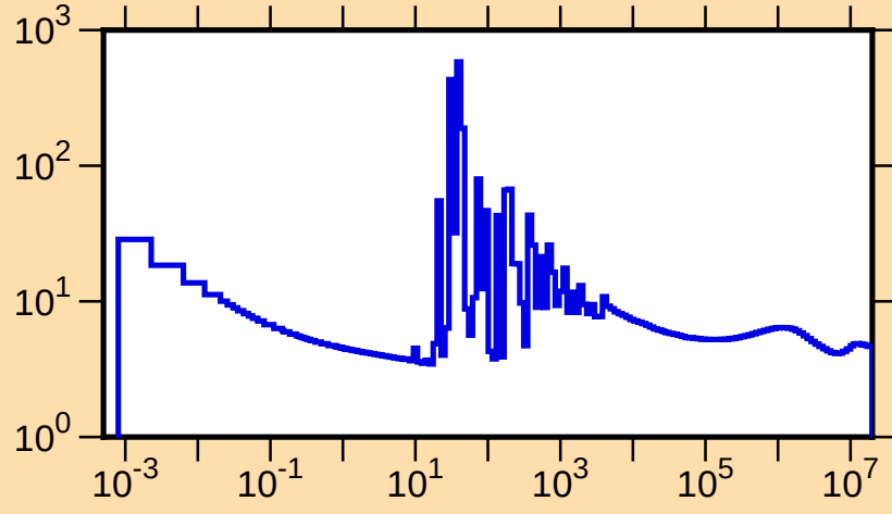
\sigma vs. E for ^{127}\text{I}(n,\text{tot.})
