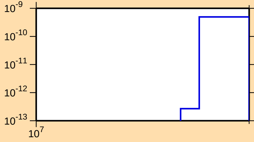
\sigma vs. E for ^{127}\text{I}(n,2n\alpha)
