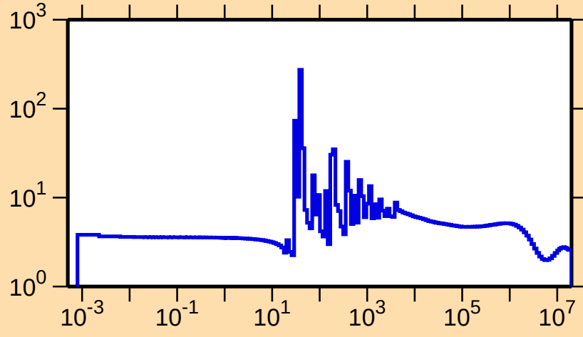
\sigma vs. E for ^{127}\text{I}(\text{n},\text{el.})
