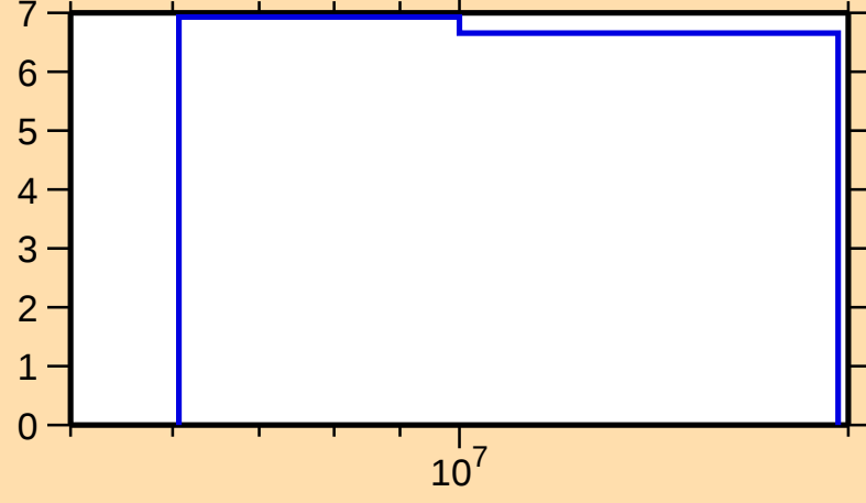
\Delta\sigma/\sigma vs. E for ^{127}\text{I}(n,\text{el.})
