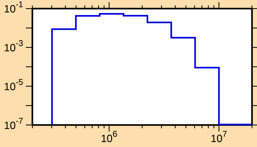
\sigma vs. E for ^{127}\text{I}(n,n_4)
