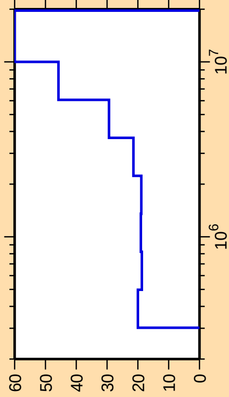
\Delta\sigma/\sigma vs. E for ^{127}\text{I}(n,n_4)
