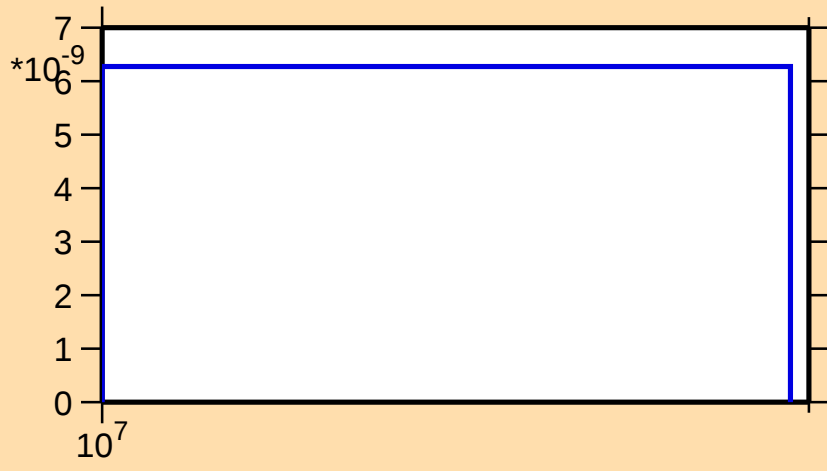
\sigma vs. E for ^{127}\text{I}(\text{n},\text{nd})
