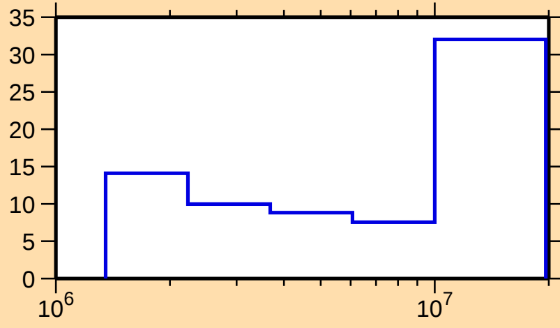
\Delta\sigma/\sigma vs. E for ^{127}\text{I}(\text{n},\text{inel.})
