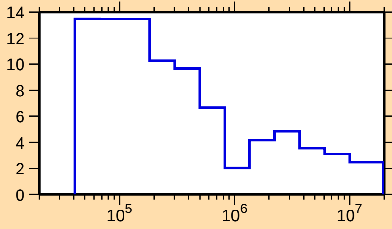
\Delta\sigma/\sigma vs. E for ^{127}\text{I}(\text{n,tot.})
