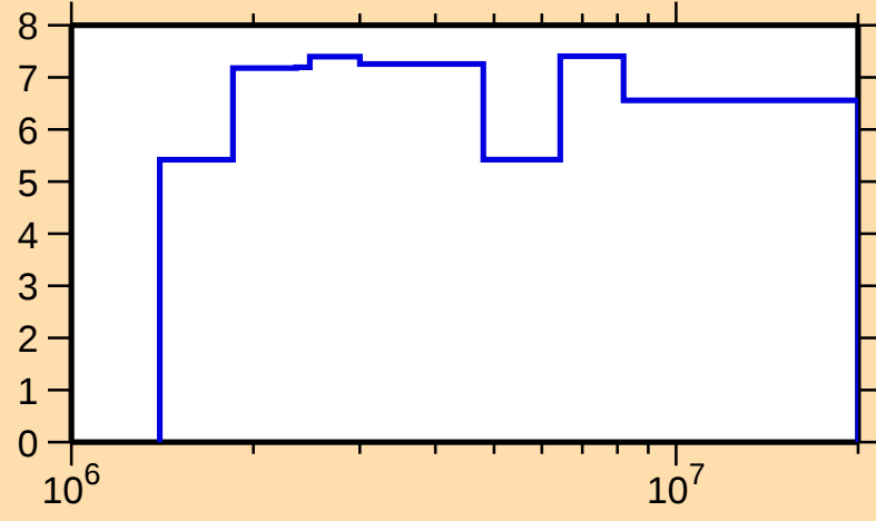
\Delta\sigma/\sigma vs. E for ^{127}\text{I}(\text{n},\text{el.})
