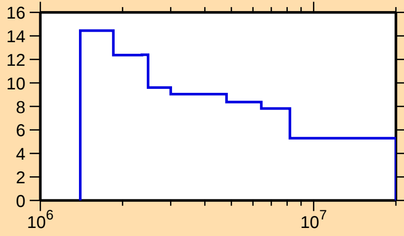
\Delta\sigma/\sigma vs. E for ^{127}\text{I}(\text{n},\text{nonel.})
