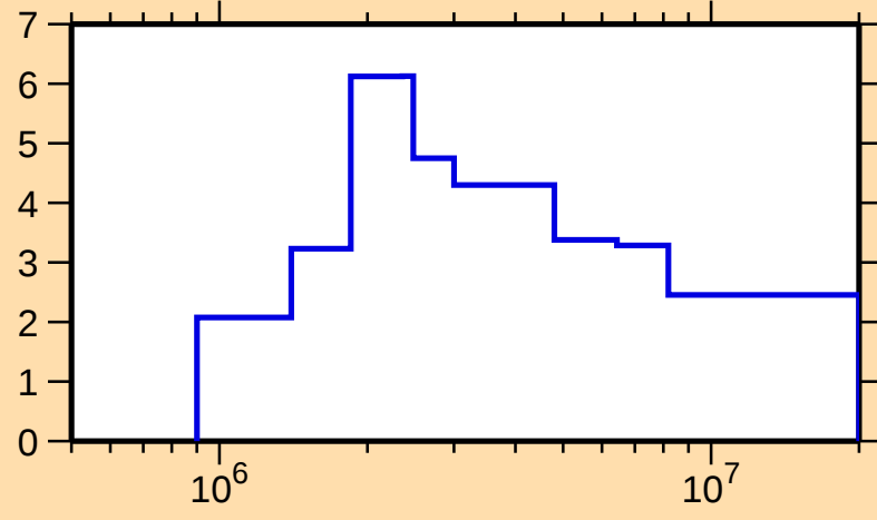
\Delta\sigma/\sigma vs. E for ^{127}\text{I}(n,\text{tot.})
