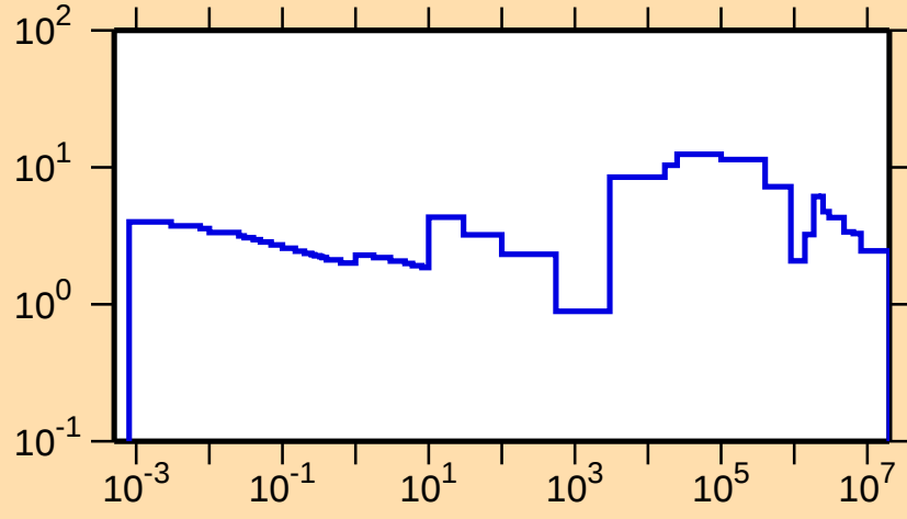
\Delta\sigma/\sigma vs. E for ^{127}\text{I}(\text{n,tot.})
