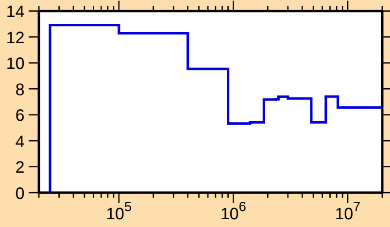
\Delta\sigma/\sigma vs. E for ^{127}\text{I}(\text{n,el.})
