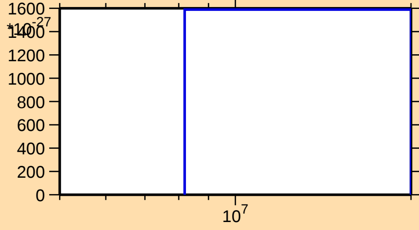
\sigma vs. E for ^{127}\text{I}(\text{mt 11})
