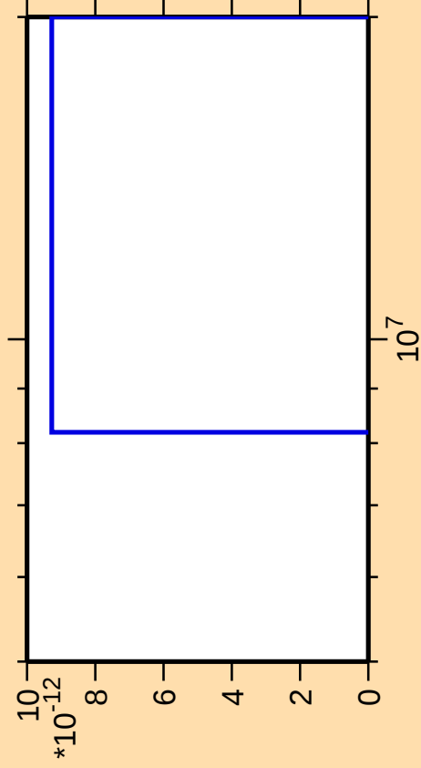
\Delta\sigma/\sigma vs. E for ^{127}\text{I}(\text{mt 11})
