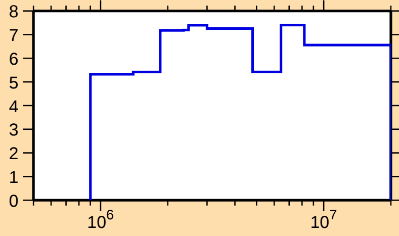
\Delta\sigma/\sigma vs. E for ^{127}\text{I}(\text{n,el.})
