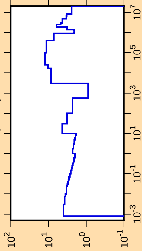
\Delta\sigma/\sigma vs. E for ^{127}\text{I}(n,\text{tot.})
