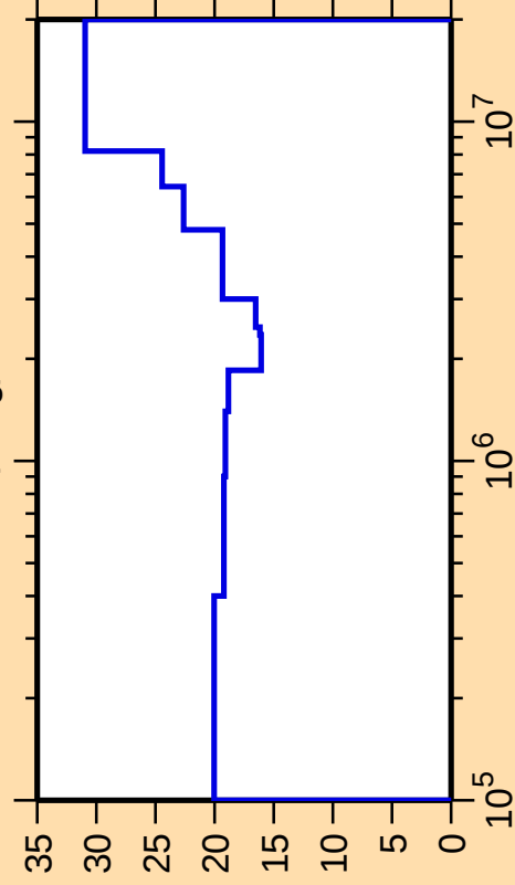
\Delta\sigma/\sigma vs. E for ^{127}\text{I}(n,n_3)
