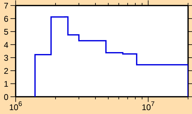
\Delta\sigma/\sigma vs. E for ^{127}\text{I}(\text{n},\text{tot.})
