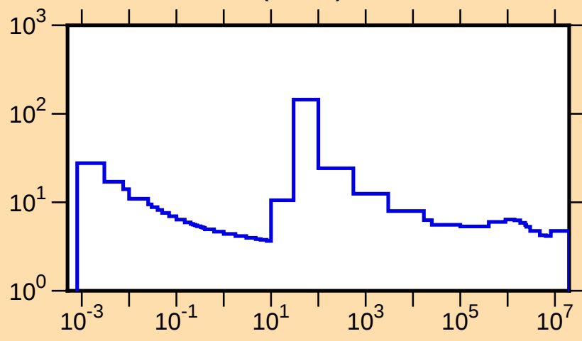
\sigma vs. E for ^{127}\text{I}(n,\text{tot.})
