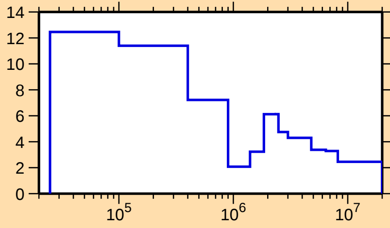
\Delta\sigma/\sigma vs. E for ^{127}\text{I}(n,\text{tot.})
