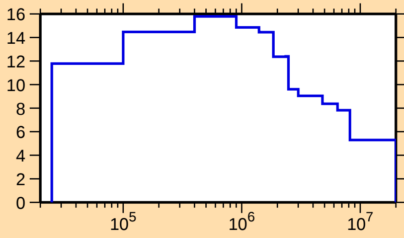
\Delta\sigma/\sigma vs. E for ^{127}\text{I}(\text{n,nonel.})
