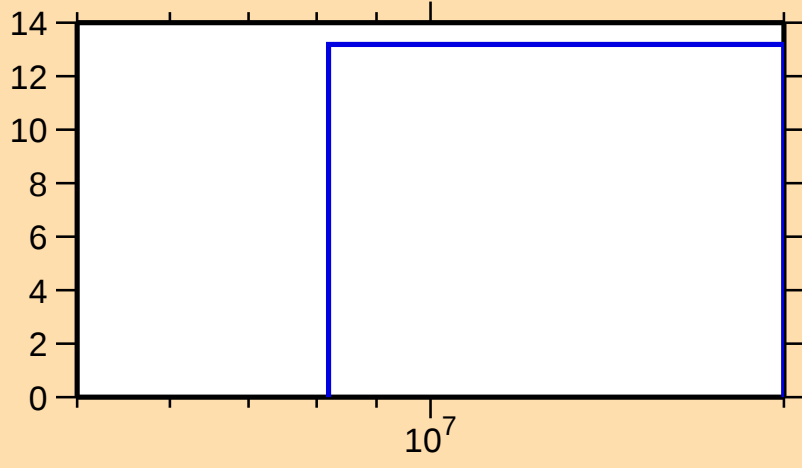
\Delta\sigma/\sigma vs. E for ^{127}\text{I}(n,2n)
