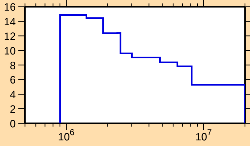
\Delta\sigma/\sigma vs. E for ^{127}\text{I}(n,\text{nonel.})
