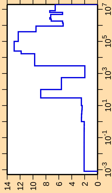
\Delta\sigma/\sigma vs. E for ^{127}\text{I}(\text{n,el.})
