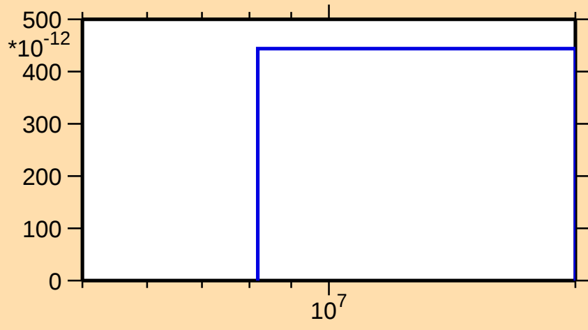
\sigma vs. E for ^{127}\text{I}(n,2np)
