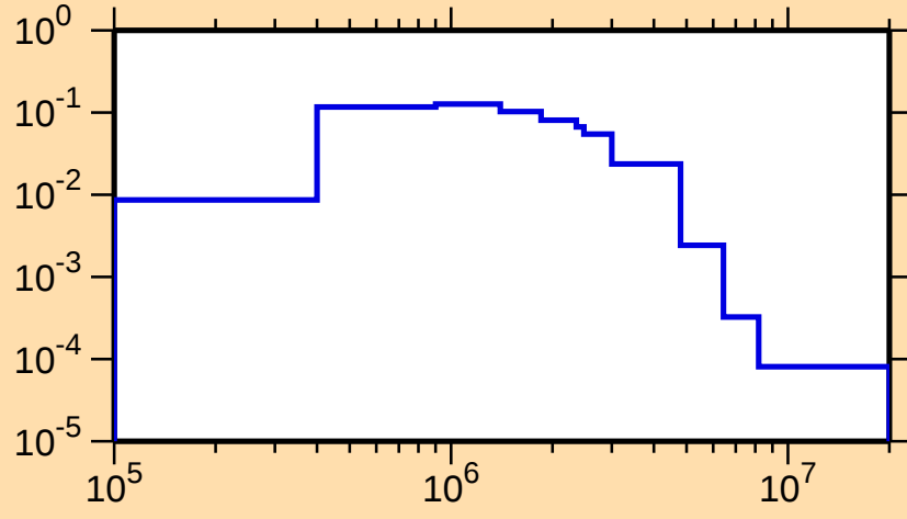
\sigma vs. E for ^{127}\text{I}(n,n_3)
