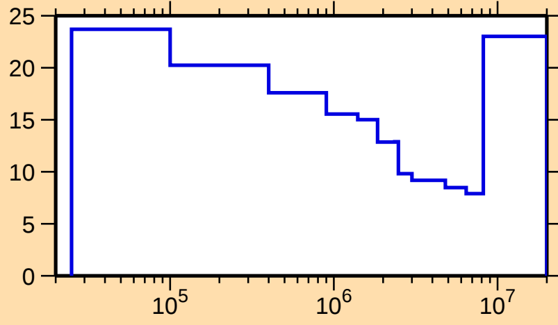
\Delta\sigma/\sigma vs. E for ^{127}\text{I}(n,\text{inel.})
