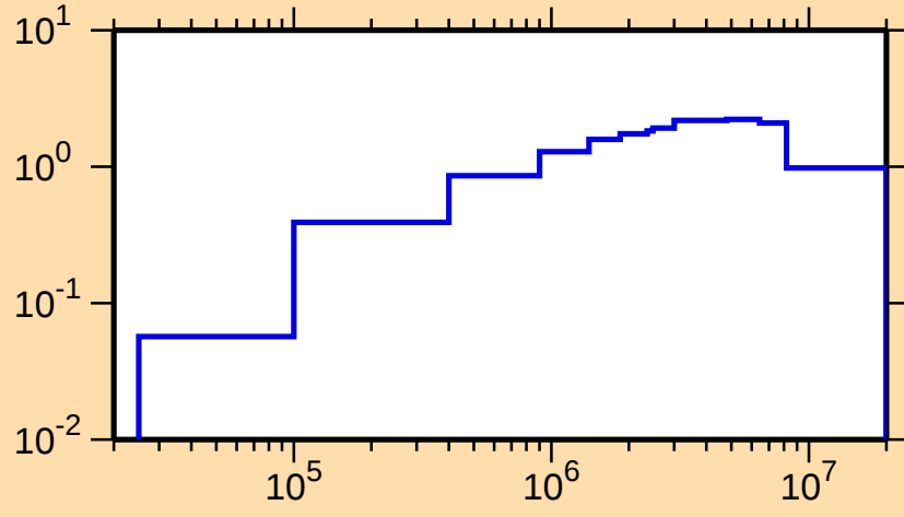
\sigma vs. E for ^{127}\text{I}(\text{n,inel.})
