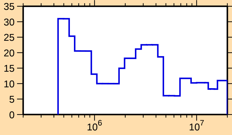
\Delta\sigma/\sigma vs. E for ^{128}\text{I}(\text{n},\text{el.})
