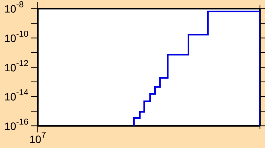
\sigma vs. E for ^{128}\text{I}(n,\text{He3})
