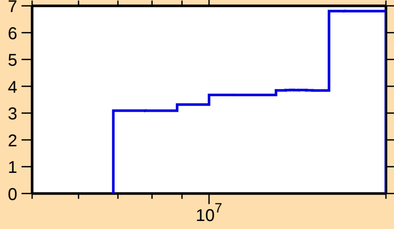
\Delta\sigma/\sigma vs. E for ^{128}\text{I}(n,\text{tot.})
