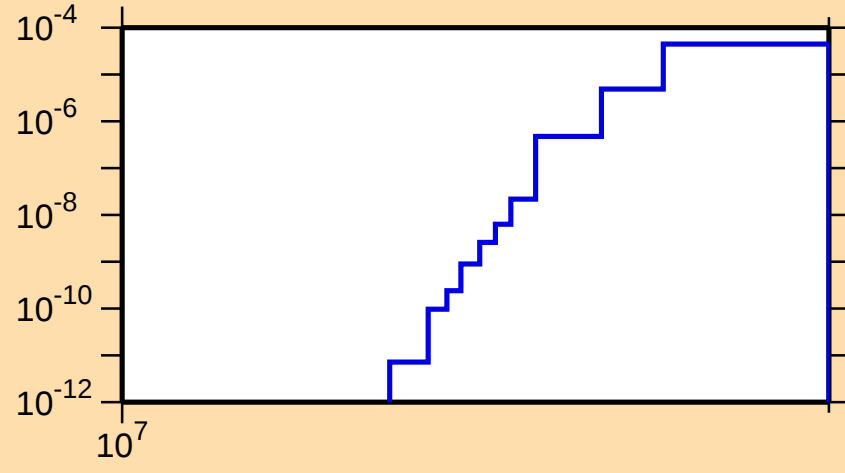
\sigma vs. E for ^{128}\text{I}(n,\text{nd})
