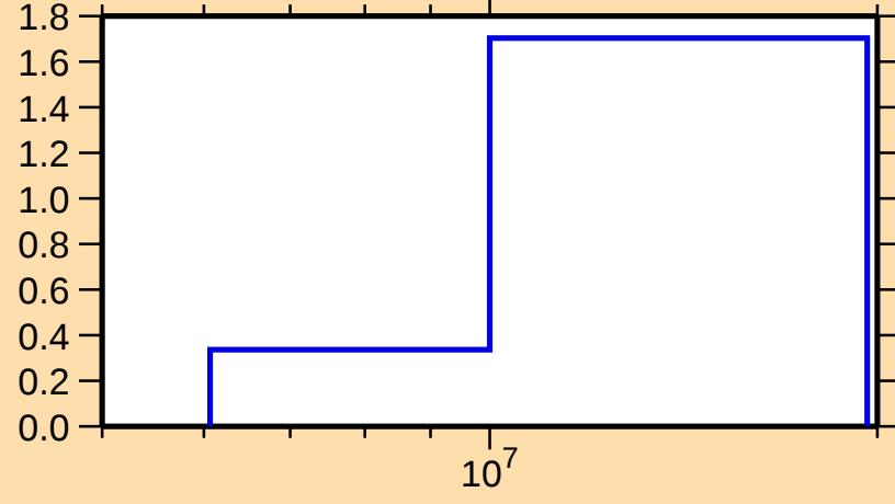
\sigma vs. E for ^{128}\text{I}(n,2n)
