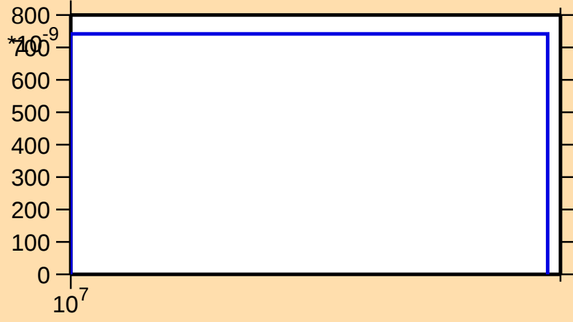
\sigma vs. E for ^{128}\text{I}(\text{n},\text{nd})
