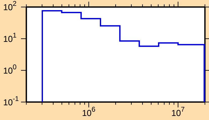
\Delta\sigma/\sigma vs. E for ^{128}\text{I}(\text{n,nonel.})
